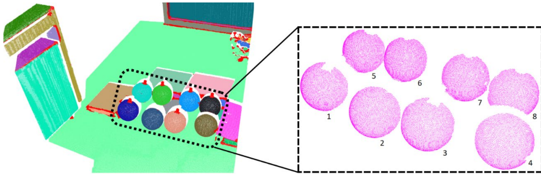
Figure 5.32: The extracted spherical clusters from region growing segments in the scanning test (Yang et al. , 2021).
