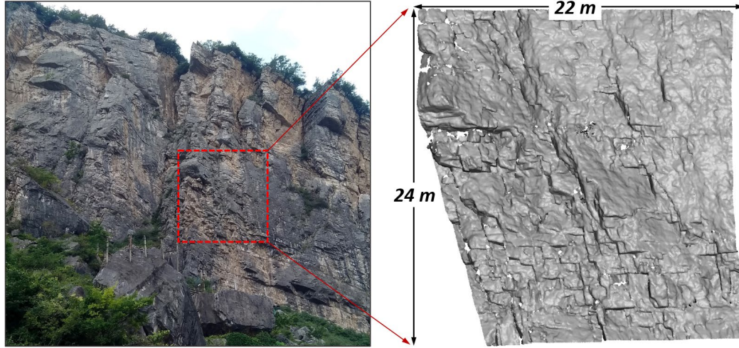
Figure 5.19: The scale and surface geometry of the selected rock cliff façade ( Yang and Schwieger, 2023 ).
