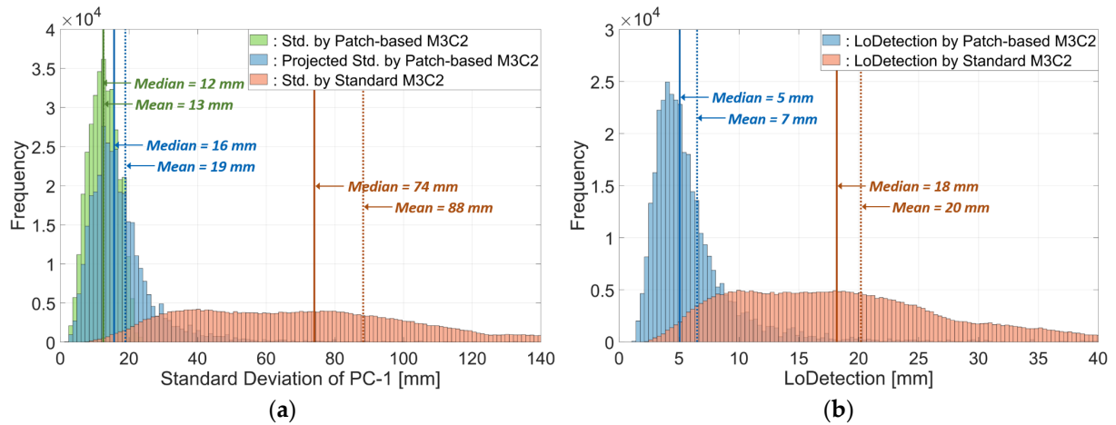
Figure 5.20: Histograms of standard deviations (a) and LoDetection (b) by standard M3C2 and PB-M3C2 ( Yang and Schwieger, 2023 ).
