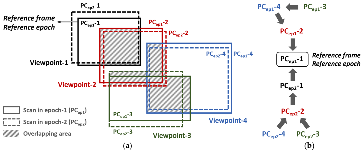
Figure 2.3: Registration strategies for multiple scans from different viewpoints and epochs: (a) Scans acquired from different viewpoints and epochs with overlapping areas; (b) Possible registration sequences of scans to the reference frame/epoch (each arrow indicates a transformation matrix).
