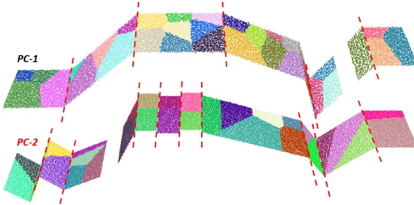
Figure 5.8: Generated patches by supervoxel-based over-segmentation (boundaries of the planes are highlighted by red dashed lines) (Yang and Schwieger, 2023).
