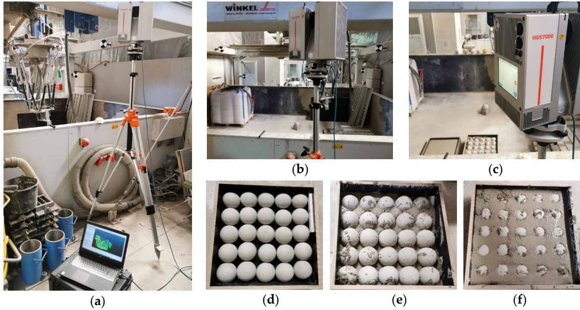
Figure 5.35: The experimental setup (a-c) and the production process of an exemplary concrete component (d-f) (Yang et al. , 2021).
