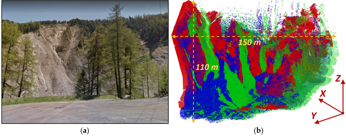
Figure 4.12: Nesslrinna landslide (a) and acquired TLS point clouds (b) (red: PC-1; blue: the registered PC-2; green: the unregistered PC-2 generated by defined transformation parameters).
