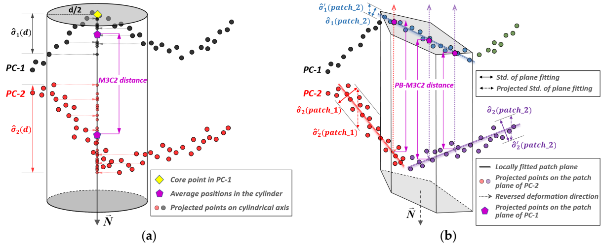
Figure 5.5: The distance calculation between two surfaces by standard M3C2 (a) and PB-M3C2 (b) (Yang and Schwieger, 2023).
