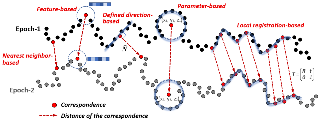
Figure 2.6: A schematic illustration of five kinds of correspondence definitions.
