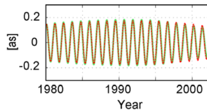
Fig. 5.3.4: Model results for polar motion (x-component) applying the combined bandpass filtered atmospheric and oceanic time series (NCEP+ECCO, red dashed). For comparison, the Chandler oscillation deduced from the C04 series by means of wavelet filtering (cf. Fig. 5.3.1) is added in green.
