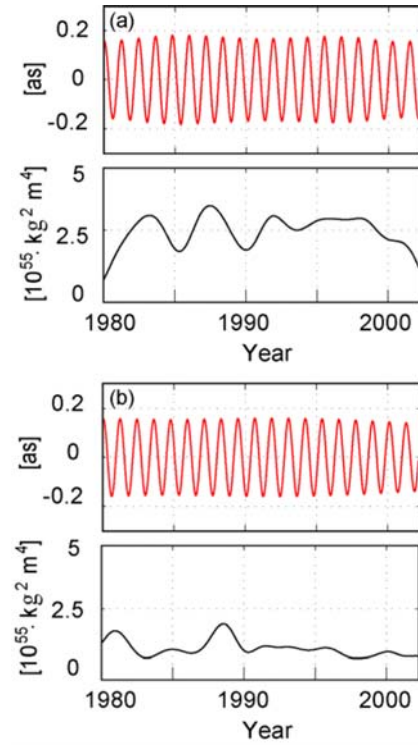
Fig. 5.3.3: Model results for polar motion (x-component) applying band-pass filtered (a) atmospheric and (b) oceanic time series of the tensor elements \Delta I_{13}(t) and \Delta I_{23}(t) (upper panels) in comparison with the integral wavelet energy of the excitations in the spectral band between 400 and 460 days (lower panels).
