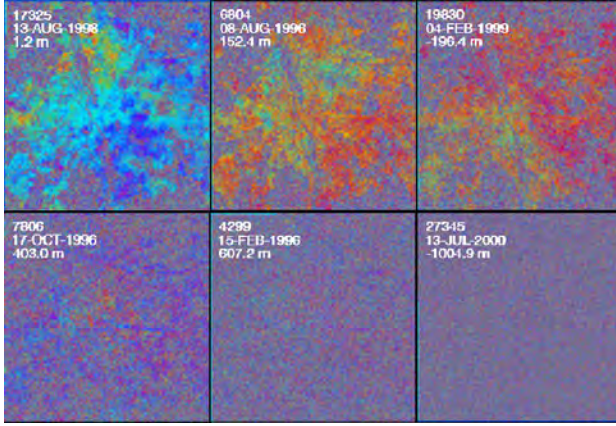
(a) Some examples of differential interferometric SAR images (dInSAR) sorted by perpendicular baseline. No spectral shift filtering is applied for PSI. Consequently, large baselines (lower right) show a high level of decorrelation, i.e., phase noise affects visual interpretation. Nevertheless, single point targets feature stable phase values, which are investigated in the framework of PSI.
