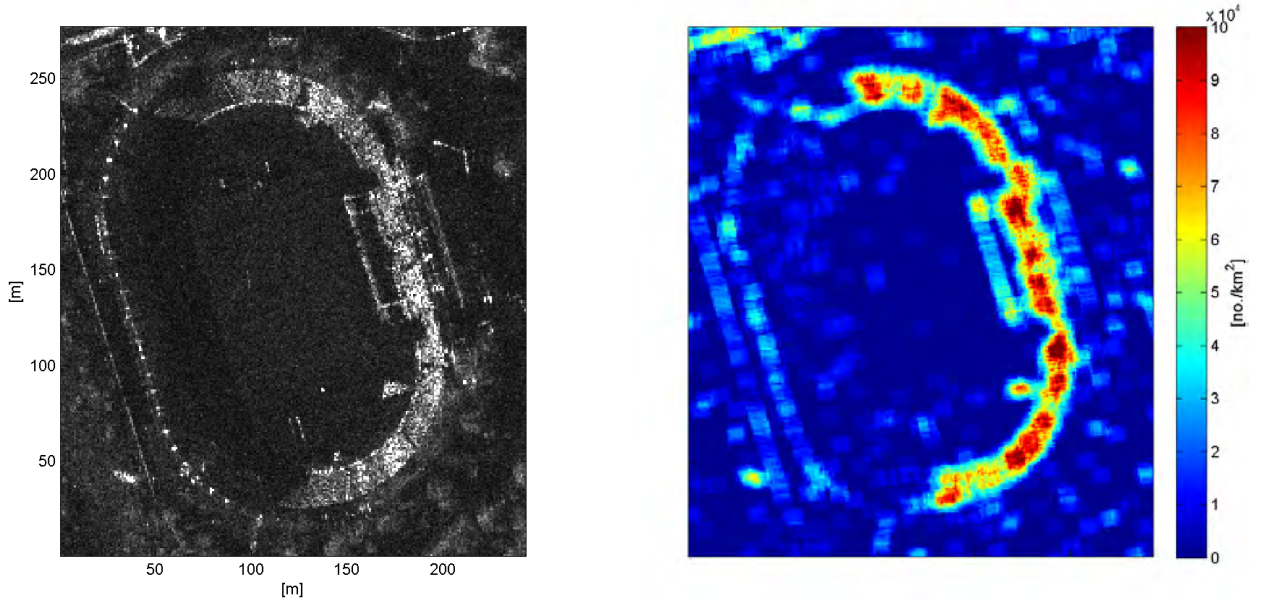
(b) Meanmap and density map of stack A51, VV.
