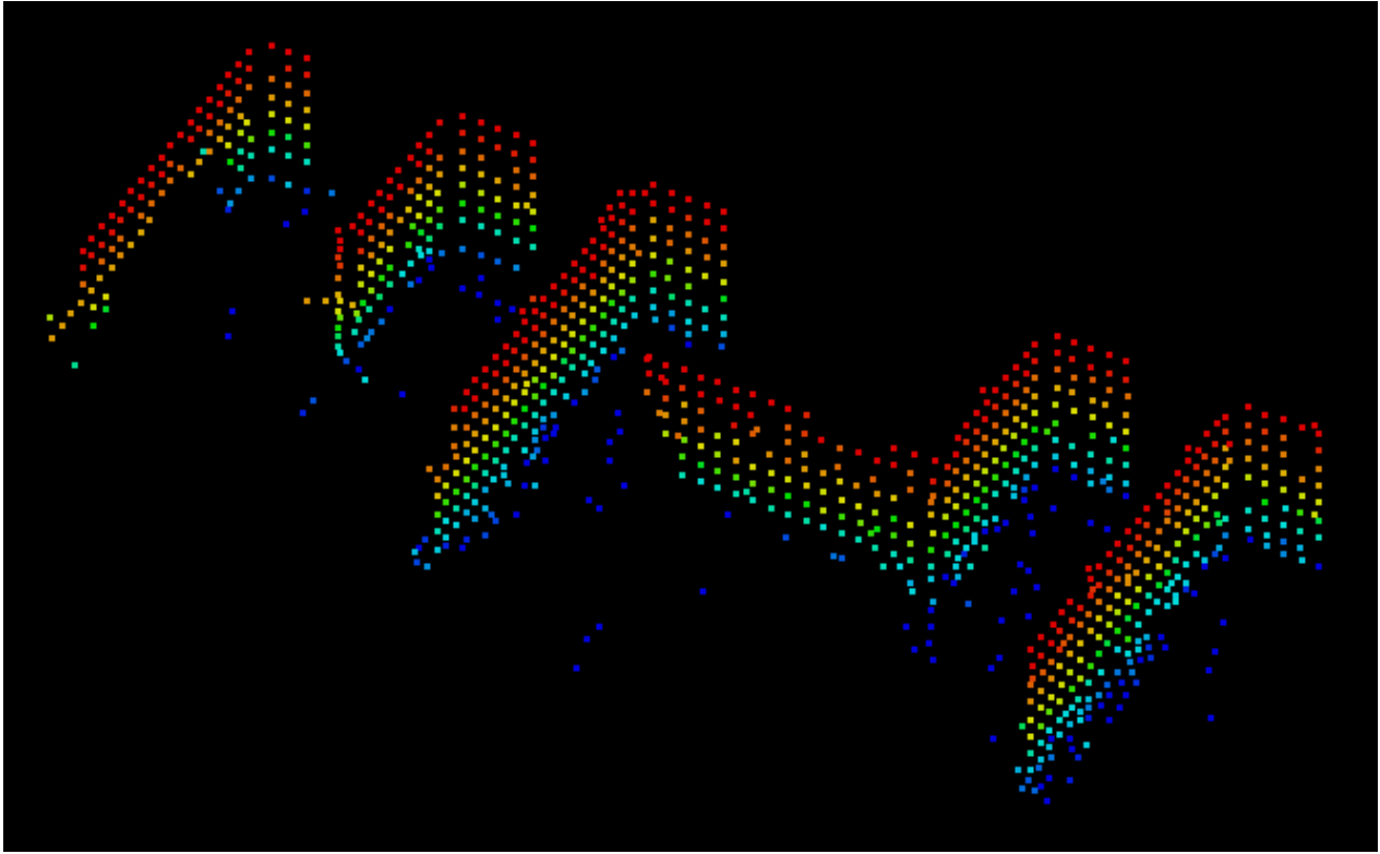
(a) Clipping of point cloud to PS originating from several building facades of identical architecture. 8 floors show linearly aligned PS at a regular spacing, most likely originating from rows of regularly spaced windows.
