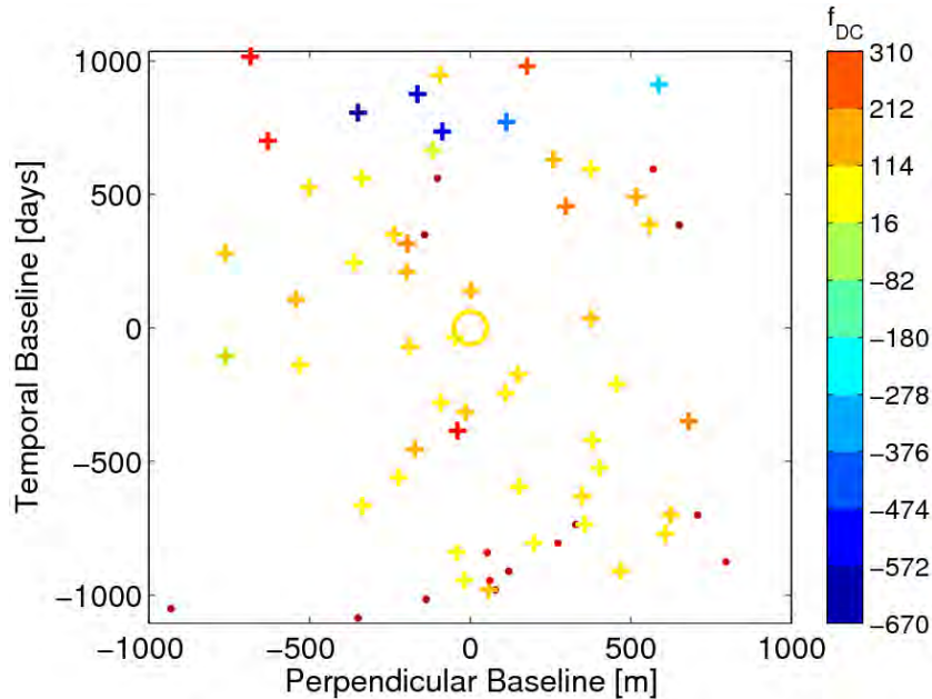
Figure 7. Plot of the distribution of the acquisitions in time and perpendicular baseline space with respect to the selected master scene (circle). Dots and crosses represent data of ERS-1 and ERS-2 respectively. Colors indicate Doppler centroid frequencies (squint angles).
