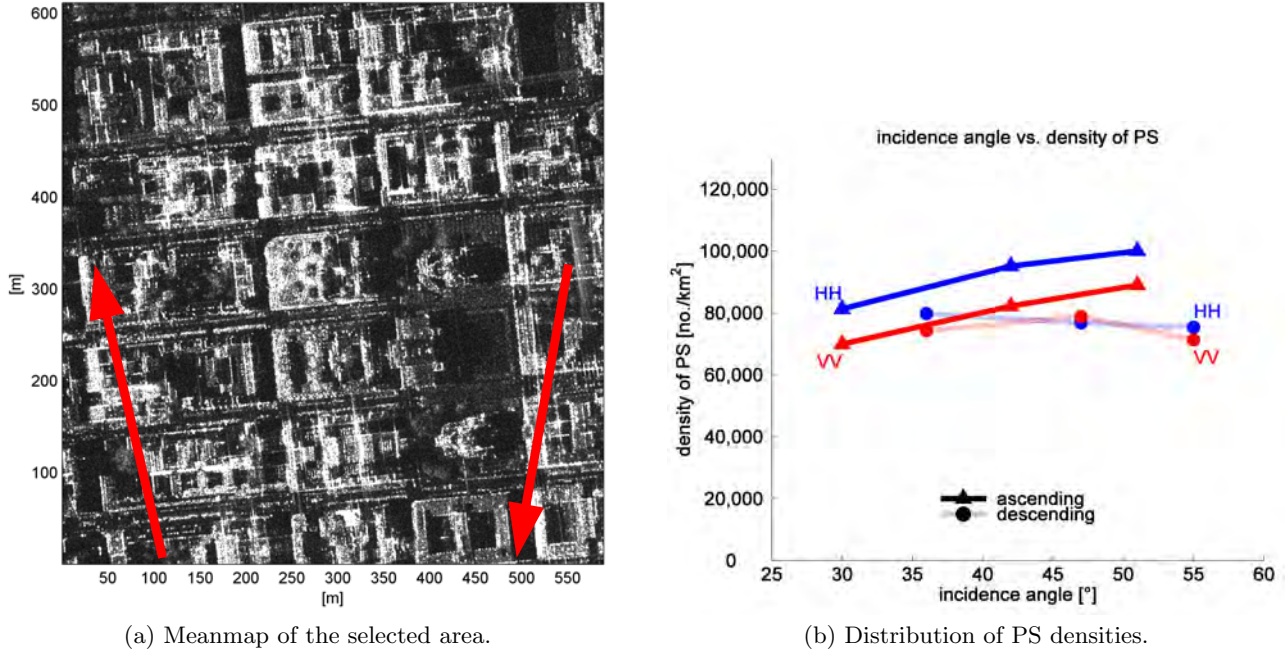
Figure 27. Left: Meanmap of first sample area used for analysis on polarization (stack A51 VV shown here). Red arrows indicate azimuth directions for ascending (left arrow) and descending (right arrow) stacks. Right: Distribution of PS densities with increasing incidence angle. Different polarization indicated by different colors and by HH/VV signatures. Solid lines including triangular markers indicate ascending tracks. Diffuse lines including round markers indicate descending tracks. PS selection requirement: SCR \geq 3.0
