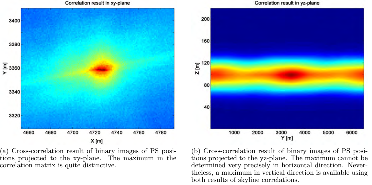
Figure 69. 2D Cross-correlation results of binary images created from PS positions projected to the xy- and yz-plane. Highest correlation (i.e., best fit) indicated by red color.
