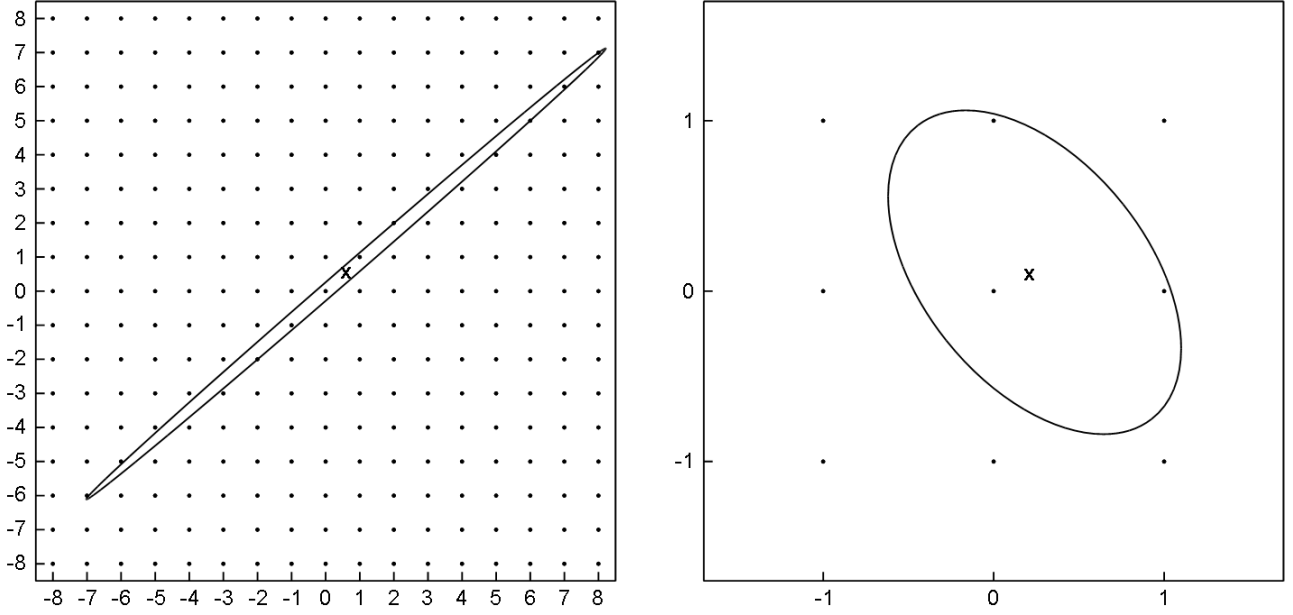
Figure 22. Example for a 2D search space before (left) and after (right) the decorrelation of the ambiguities by applying the transformation matrix Z . The size of the integer search grid is significantly reduced. The float ambiguity vector is indicated by a cross.
