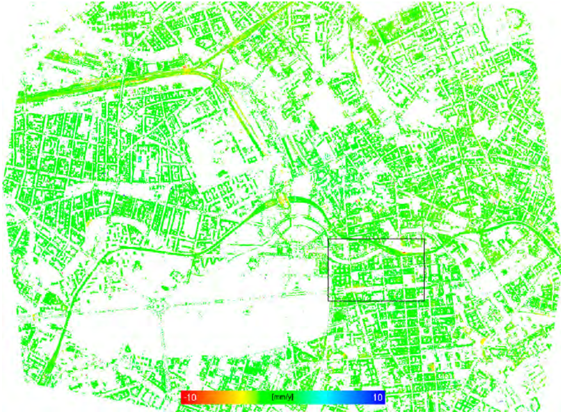
Figure 86. Top view on PS of Berlin test site colorcoded by the estimated linear components in vertical direction in the interval [-10, +10] mm/y. Significant subsidence is visible for some locally limited areas. Area of Figure 87 indicated by black rectangle.
