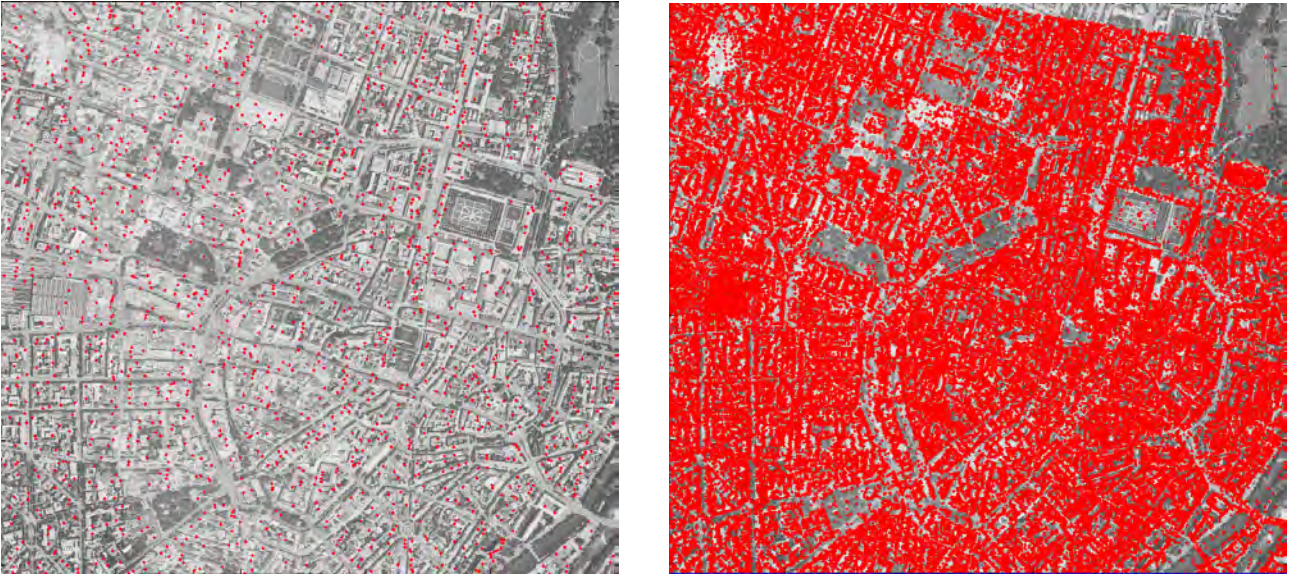
Figure 26. Visual comparison of PS detectable from stacks of medium (left) and high resolution (right) SAR data of Munich. The geocoded PS (red dots) are overlaid on an aerial image. The results are based on stacks of ERS and TerraSAR-X high resolution spotlight data.
