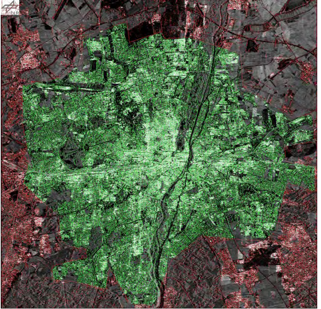
Figure 10. All PS candidates detected for the test site of Munich. The estimation is restricted to the selection of green points, covering the complete city center. Due to the selection criteria, especially bright points are identified as PS.
