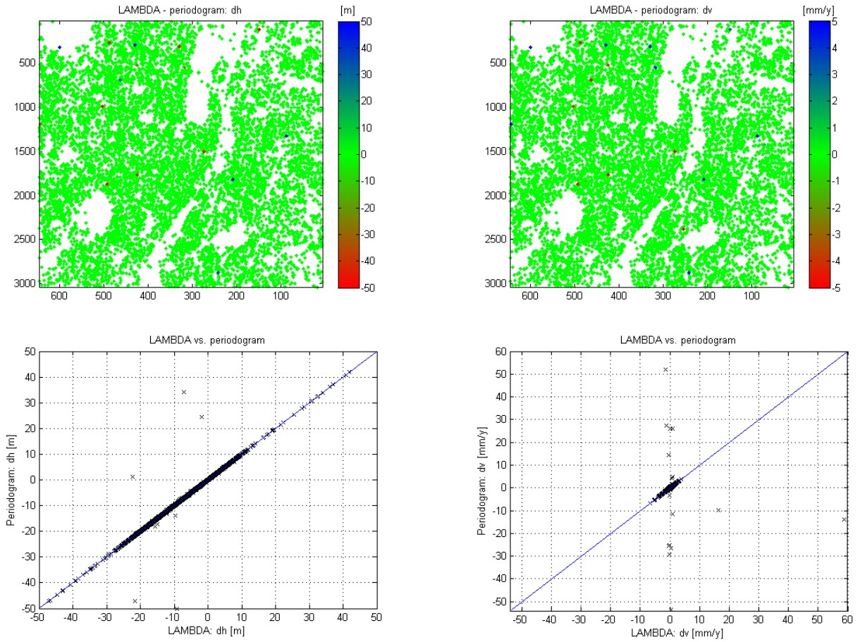
Figure 25. Top: Comparison between final results using the two different estimates of the reference network. Only a few single PS show larger deviations. Bottom: Scatterplot of both results show only a few discrepancies between the two final results for both parameters.
