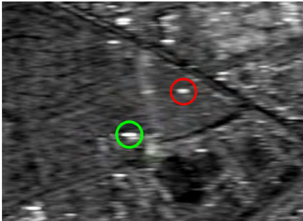
(a) Zoom into the temporal mean image of Munich. Circles indicate the two PS between which the deformation is analyzed. The green circle indicates the PS at the church (stable basement), while the red marker shows the position of the PS at the garden cottage (directly connected to ground) affected by seasonal motion.
