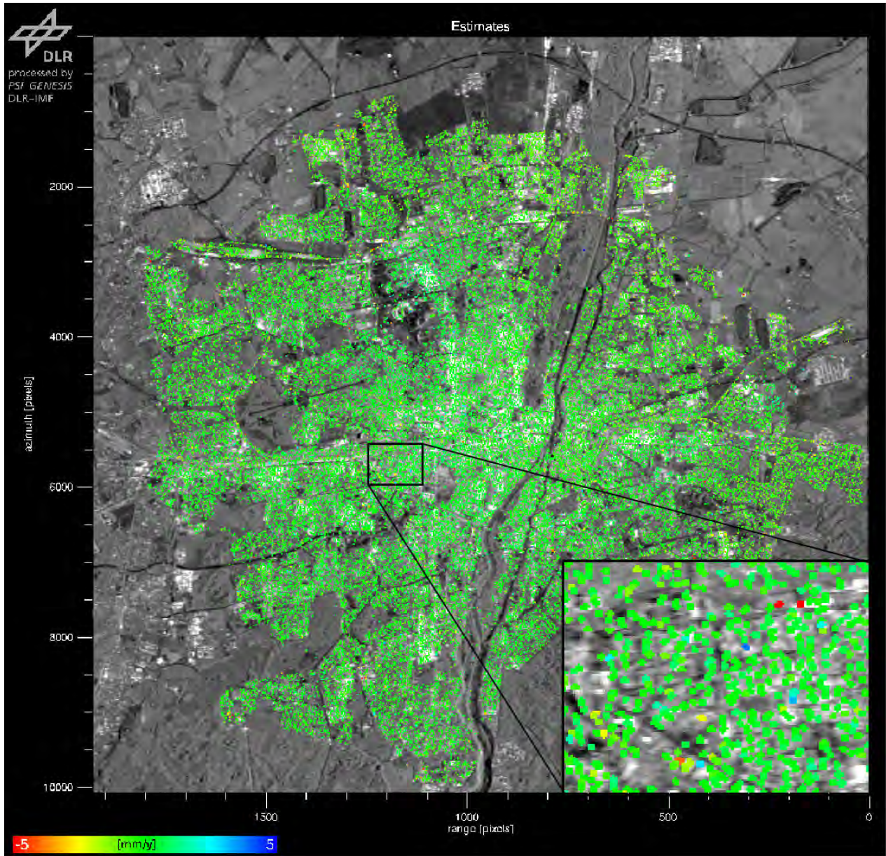
Figure 12. Linear deformation estimated for the test site of Munich in the interval [-5, 5] , units: mm/y. Green color indicates stable points. Blue colors shows LOS deformation towards the sensor, red colors imply motion in the opposite direction (subsidence). No large area deformation pattern is present; only a few single points are affected by significant deformation (see zoom of area highlighted by black rectangle on bottom right).
