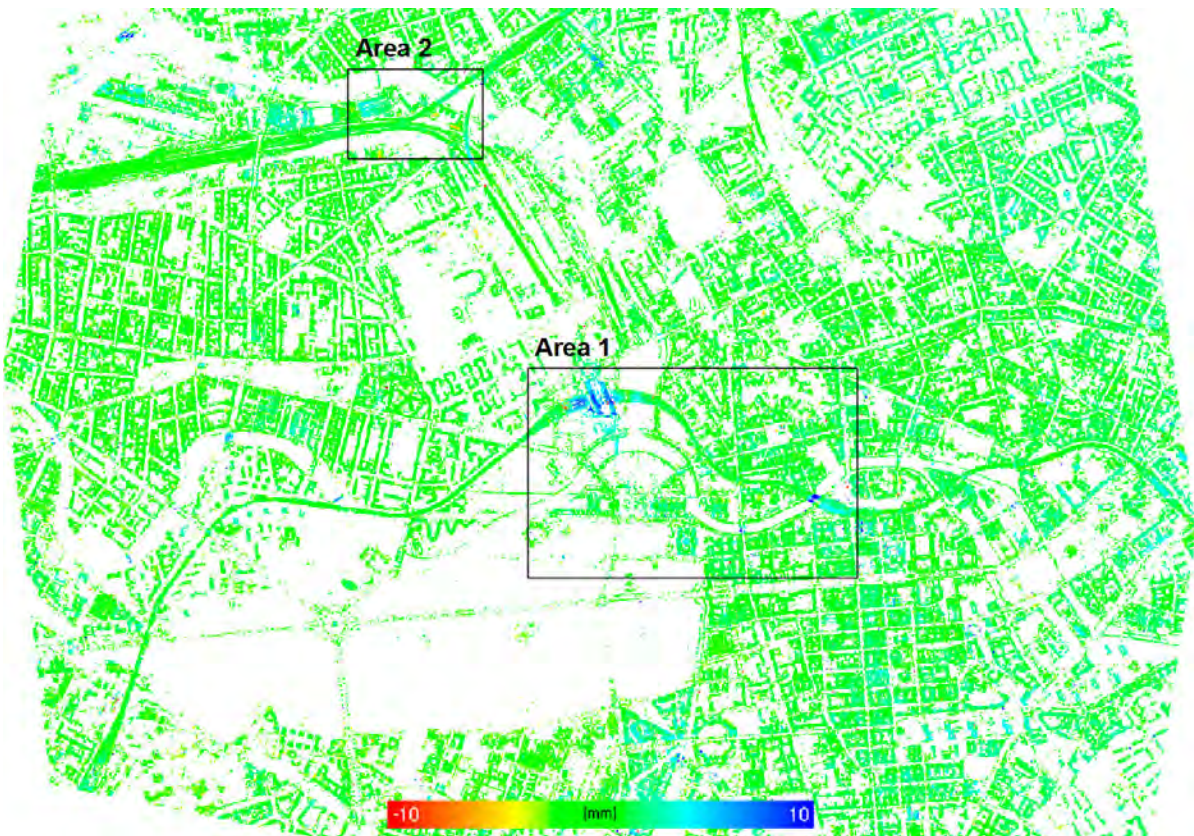
Figure 79. Top view on PS of Berlin test site colorcoded by the estimated seasonal components in vertical direction in the interval [-10, +10] mm.
