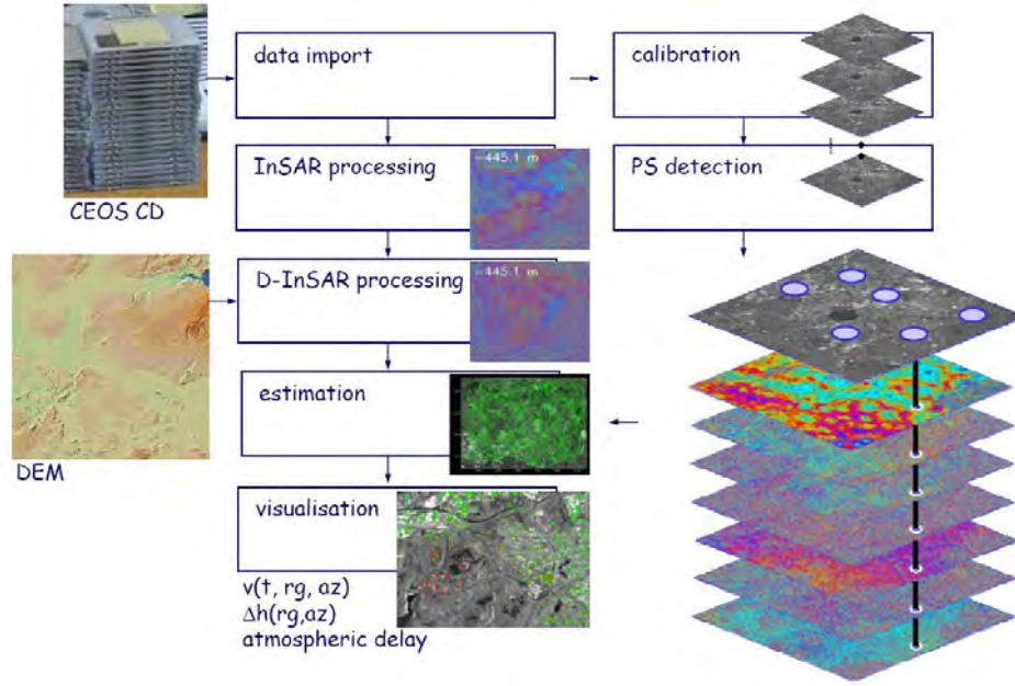
Figure 6. Flow chart of PSI estimation, proposed by Adam et al. (2003).
