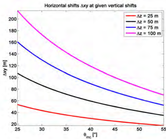
(a) Horizontal shift \Delta xy at four different fixed vertical offsets \Delta z , indicated by different colors. Graphs show dependence on incidence angles \theta_{inc} .
