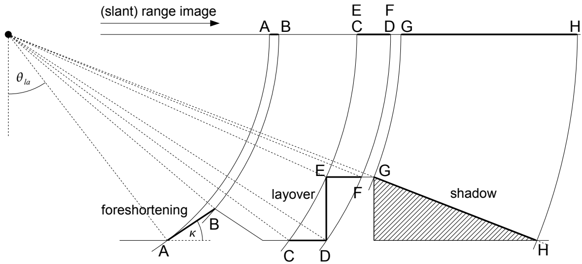
Figure 3. Geometrical effects in SAR images. Distance between A-B is compressed in the slant range image (foreshortening). Areas C-D, D-E and E-F are mapped into the same range cells (layover). None of the surfaces between G and H are illuminated by the sensor, which results in empty range cells in the radar image (radar shadow). Two important parameters are look angle of the sensor \theta_{la} and slope of terrain \kappa .
