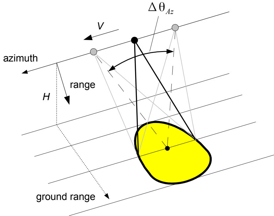
Figure 1. Acquisition geometry of a spotlight SAR system. The side looking sensor (flying at height H with velocity V ) illuminates a certain area on ground (yellow part, limited in ground range by its swath width). The scene is mapped to the azimuth - slant range plane (flying direction - look direction). In spotlight mode the resolution is increased by sweeping the azimuth beam backwards (beam steering angle \Delta\theta_{Az} ) in order to extend illumination time of each scatterer.
