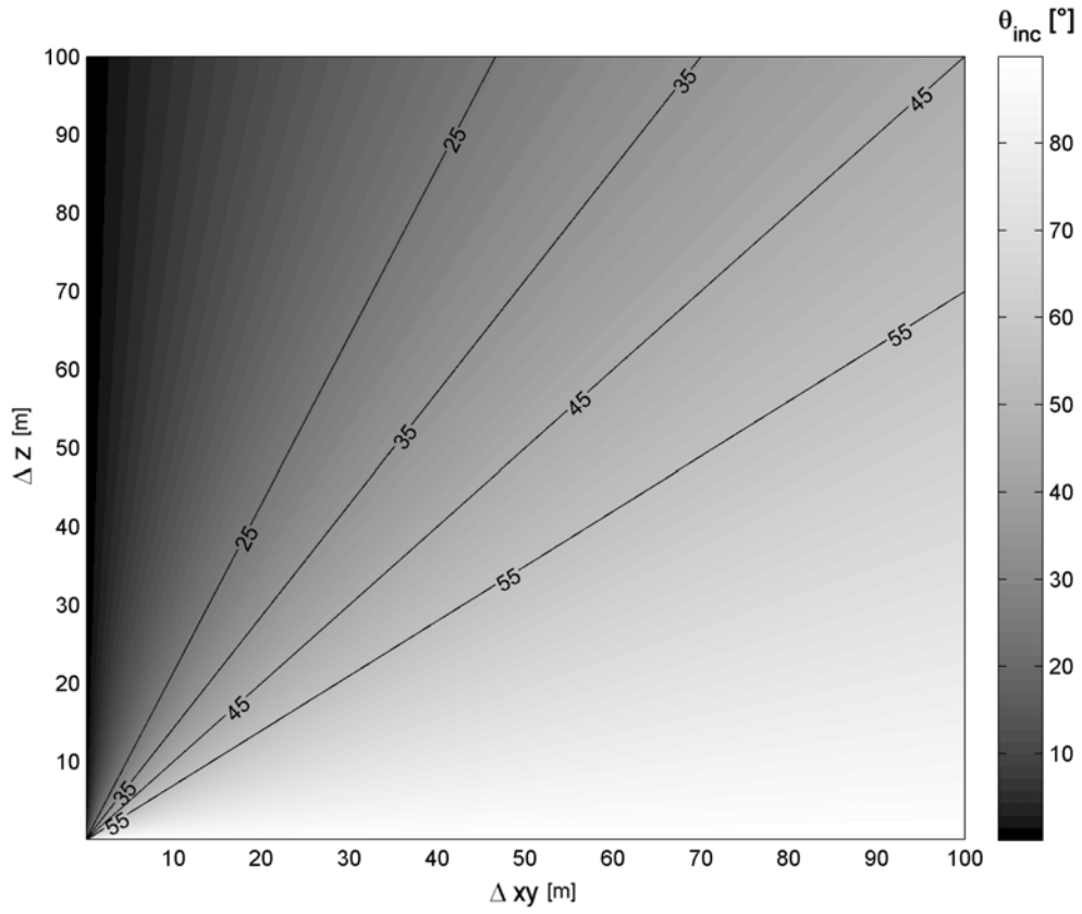
Figure 37. Plot of maximum incidence angles in order to allow an extraction of potential PS from ground floor. Geometry given by distance \Delta xy between two buildings and height \Delta z of the front building inducing shadow on the other one. Isolines of different incidence angles are overlaid on top.
