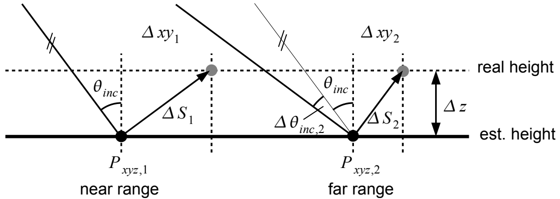
(b) Incidence angles vary between near and far range positions P_{xyz,1} and P_{xyz,2} . Therefore, the shifts in elevation directions \Delta S_1, \Delta S_2 as well as the shifts in horizontal directions \Delta xy_1, \Delta xy_2 differ. Consequently, the shift has to be modeled depending on the range coordinate of each PS, implemented by individual shift directions based on the local incidence angle \theta_{inc} + \Delta \theta_{inc} . The vertical component of the shift is equal for all points of one stack.
