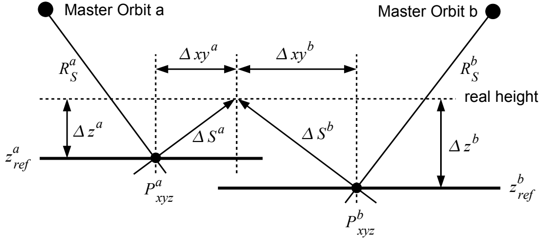
(a) Side view on acquisition geometry of cross-heading tracks. Two identical PS ( P_{xyz}^a, P_{xyz}^b ) from both point clouds may differ in vertical as well as horizontal positions, indicated by \Delta z^a, \Delta z^b and \Delta xy^a, \Delta xy^b . These offsets are induced by uncertainties in the height of the reference points z_{ref}^a, z_{ref}^b . A shift by \Delta S^a, \Delta S^b in elevation directions of the respective points will lead to identical coordinates for both PS in their final absolute positions at the real height. R_S^a, R_S^b indicate range distance between master orbits and PS.
