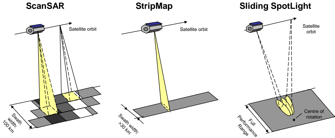
Figure 16. TerraSAR-X acquisition modes (left to right): ScanSAR, StripMap and Spotlight. Each mode differs in coverage and resolution.
