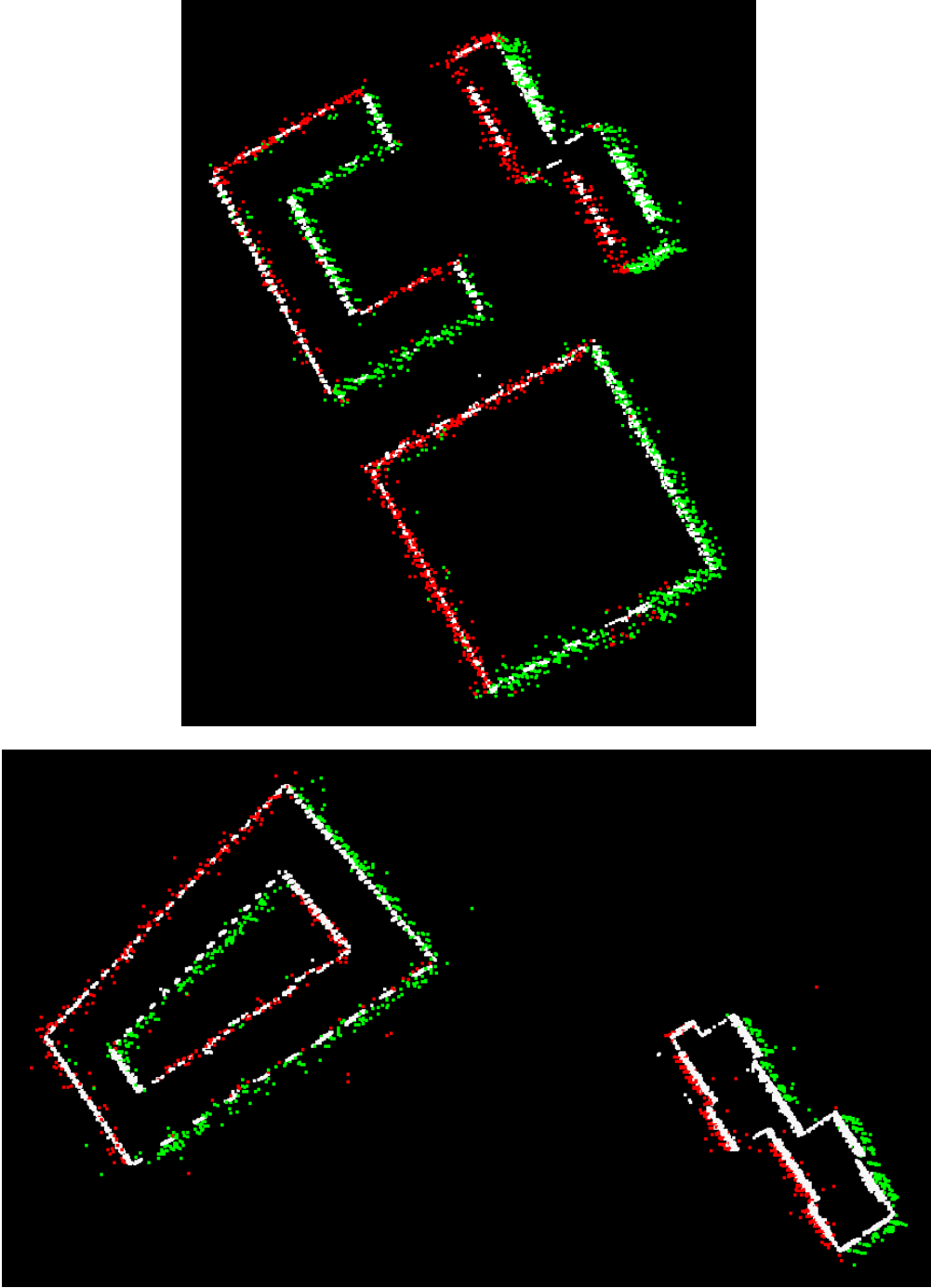
Figure 77. Top view on PS positions after fusion of ascending stack A42 (red dots) and descending stack D36 (green dots). The white dots represent the reference data of the LIDAR point cloud. All data is clipped to the parts corresponding to facades of the buildings. Two examples of different location of Berlin test site are given. The deviations of a mean plane obtained from the PS and one calculated from the reference LIDAR point cloud are investigated.
