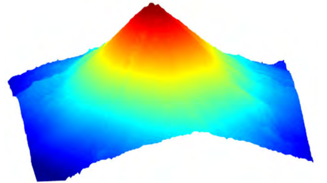
(d) Side view on the DEM of the volcano. Colorcoding of heights like in Figure 4c.
