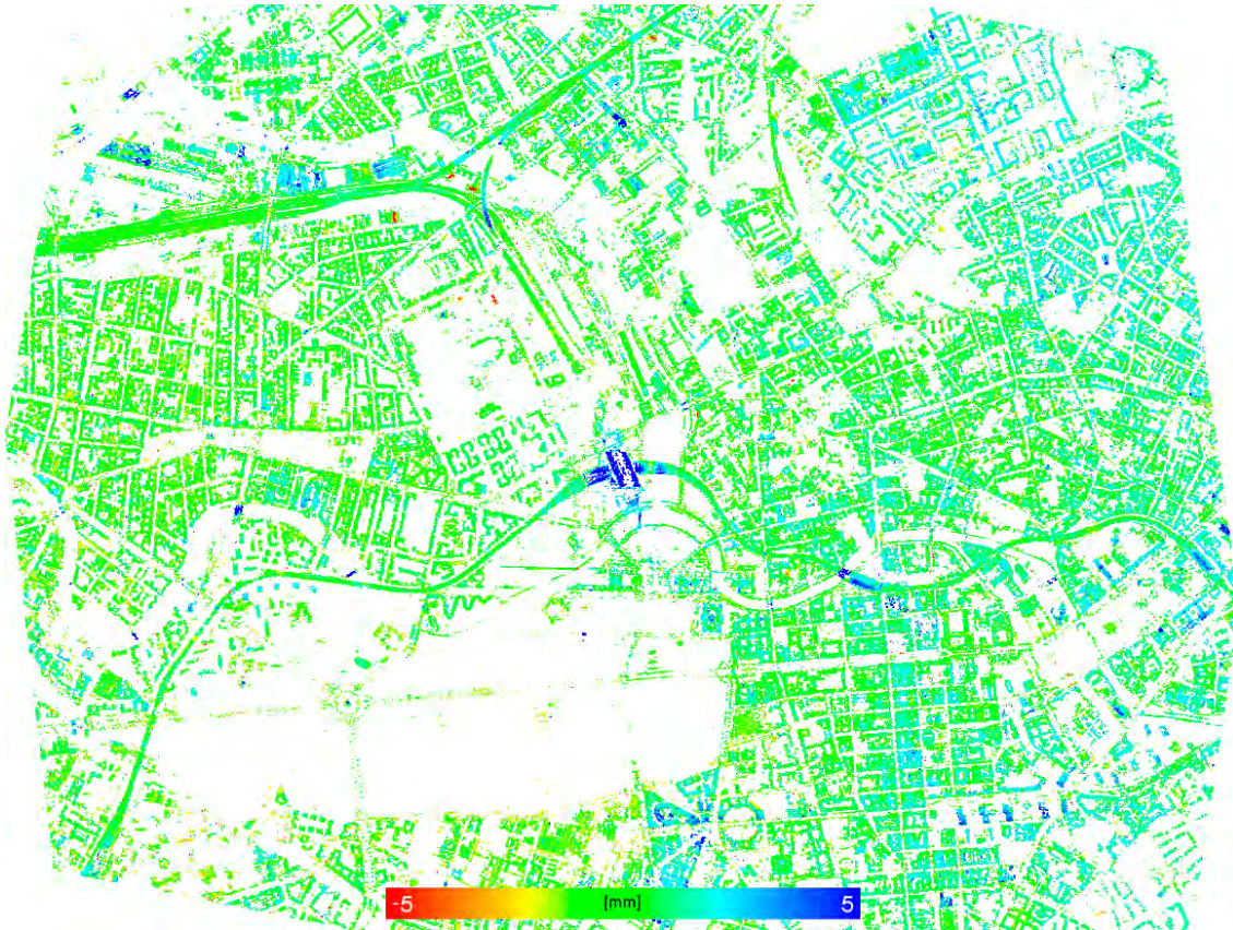
Figure 85. Top view on PS of Berlin test site colorcoded by the estimated seasonal components in vertical direction in the interval [-5, +5] mm.
