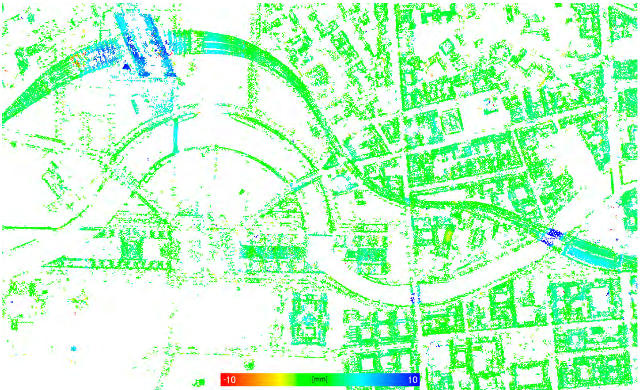
Figure 81. Top view on PS of area 1 in Berlin (cf. Section 4.4.2) colorcoded by the estimated seasonal components in vertical direction in the interval [-10, +10] mm.
