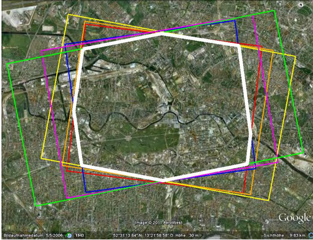
Figure 17. Test Site Berlin. Rectangles indicate different stacks, separated by color: Ascending stacks A30 (green), A42 (purple) and A51 (blue); descending stacks D36 (yellow), D47 (orange) and D55 (red). Layover generated in Google Earth TM . White polygon indicates area covered by all stacks.
