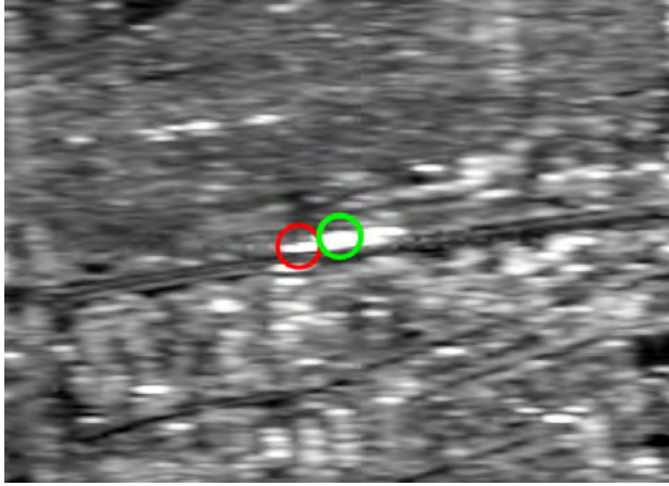
(a) Zoom into the temporal mean image of Munich. Circles indicate the two PS between which the deformation is analyzed. In this case the PS are situated at different parts of one large building. Green circle indicates stable PS; red circle marks position of subsiding point.
