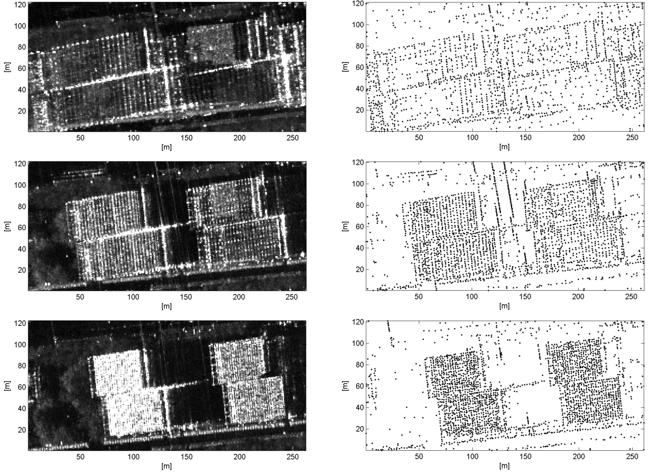
Figure 34. First sample area for analysis on incidence angle influence. Left: Meanmaps of skyscrapers at increasing incidence angles; top to bottom: Stack A30, A42, A51, all VV; right: plot of detected PS positions (black dots). Note the major change in number of PS switching from step to mid range incidence angles (top to mid figures). Also note the regular patterns that are induced by rows of windows on the facade of the building.
