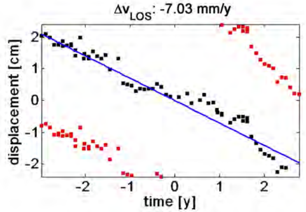
(b) Phase history between two PS given by relative motion after the removal of estimated relative height offset. Phase distribution ( \pm 2\pi ambiguities in red) is overlaid by the estimated linear trend (solid line). The displacement rate has been estimated to be approximately 7 mm/y.
