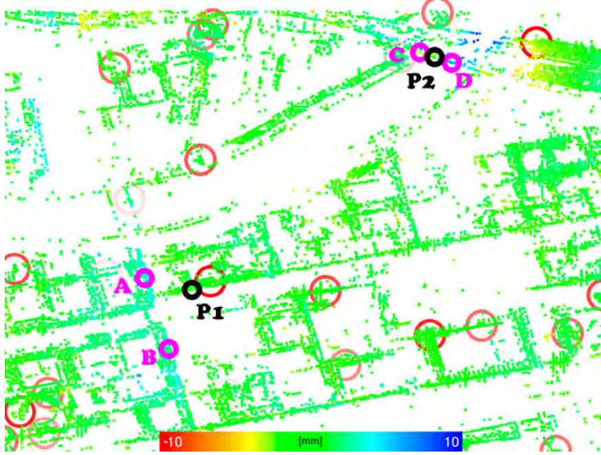
Figure 46. Sample location (area 1) \bar{1}.25 km south-east of central train station (between Brandenburger Tor and train station Berlin-Friedrichsstraße ) showing larger deformation signals at final PS in Berlin. Circles indicate points of reference network, intensity of circle color shows deformation rate between 0 and 1 mm (intense red color) of periodic motion. Colors of points represent estimated seasonal amplitudes of deformation signal between -10 mm (red = subsidence in summer) and +10 mm (blue = uplift in summer) in LOS. Relative displacement in subsequent phase history plots between PS indicated by black (P1 and P2) and each magenta (A-D) circle. Points are plotted in the azimuth-range plane.
