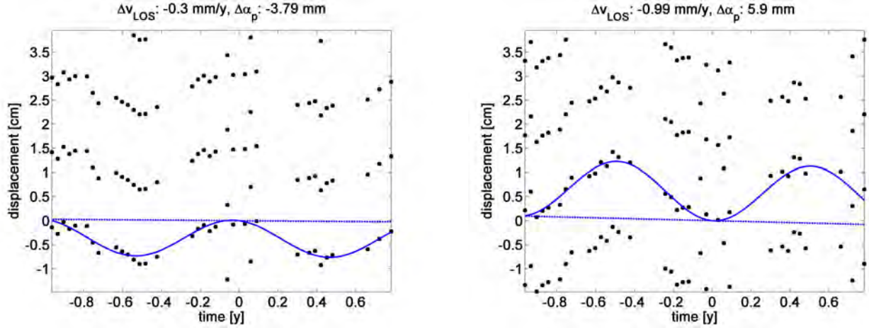
Figure 48. Phase history (including \pm 2\pi ambiguities) showing relative deformation rate between two PS of area 1. Black dots represent relative deformation signal. Blue line indicates estimated deformation. First number in title corresponds to estimated linear, second to amplitude of periodic deformation. Left: Dominating seasonal amplitudes of -3.79 mm (selection P2-C). Right: Dominating seasonal amplitudes of +5.9 mm (selection P2-D).
