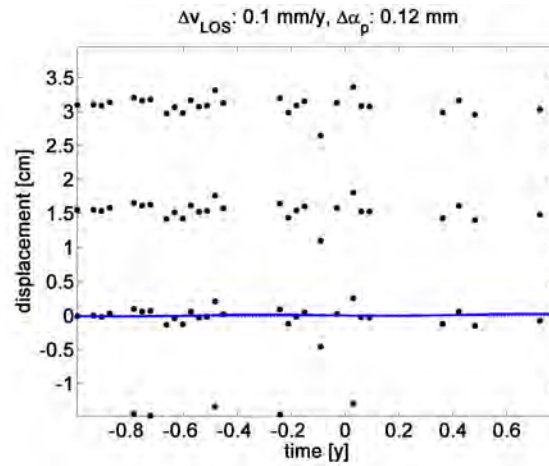
Figure 50. Phase history (including \pm 2\pi ambiguities) showing relative deformation rate between two PS of area 2. Black dots represent relative deformation signal. Blue line indicates estimated deformation. First number in title corresponds to estimated linear, second to amplitude of periodic deformation. No significant motion present, neither linear nor seasonal (selection P-A).
