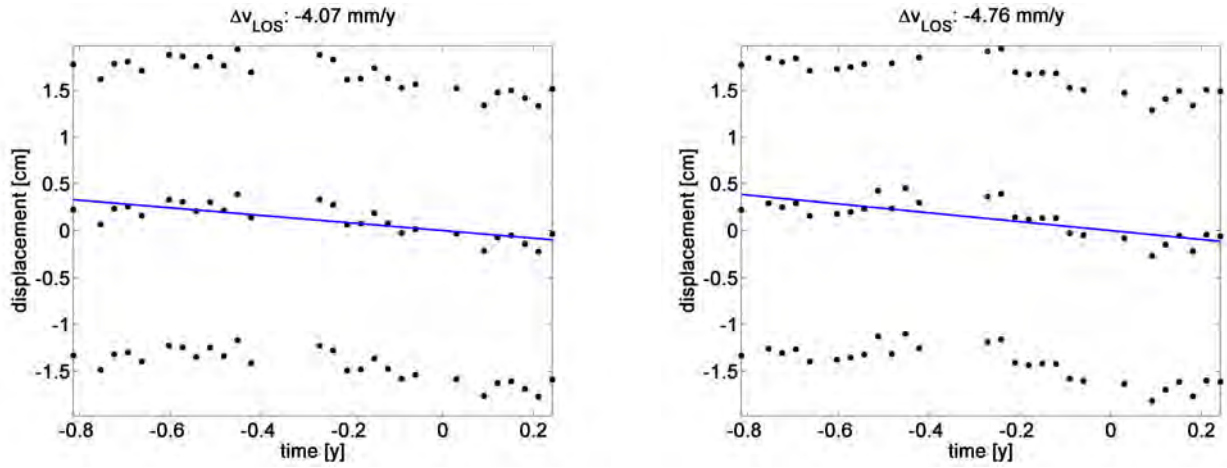
Figure 43. Phase history (including \pm 2\pi ambiguities) showing relative deformation rate between two PS of area 2. Black dots represent relative deformation signal. Blue line indicates estimated deformation. Left: -4.07 mm/y of subsidence (selection P-C). Right: -4.76 mm/y of subsidence (selection P-D).
