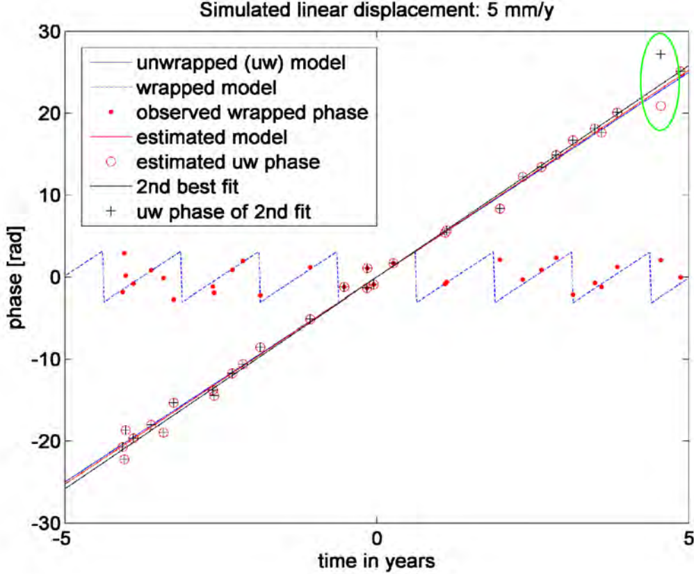
Figure 21. Example for integer ambiguity estimation taken from PSI. The linear slope is estimated from the initial distribution of wrapped phase observations (red dots), simulated from a deformation model and noise. The unwrapped true model is plotted as blue line, the estimated best and second best solutions are indicated by red and black lines. The corresponding unwrapped phase values are shown as red circles and black crosses. The second best solution differs in one single ambiguity (area highlighted by green ellipse), which is at a distance of one cycle ( 2\pi ) in comparison to the best solution.
