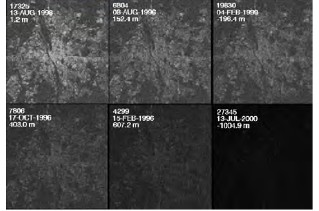
(b) Coherence estimates of dInSAR results, sorted by perpendicular baseline. Decorrelation effects increase faster for larger perpendicular baselines than for larger temporal differences between the acquisitions.
