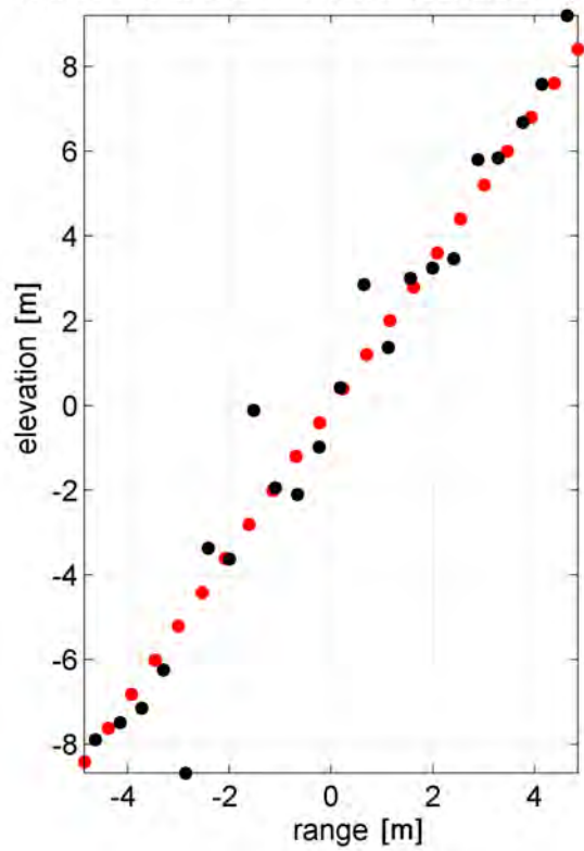
(b) View on PS in range-elevation plane. As expected, deviations in elevation direction are much larger than in azimuth or range.
