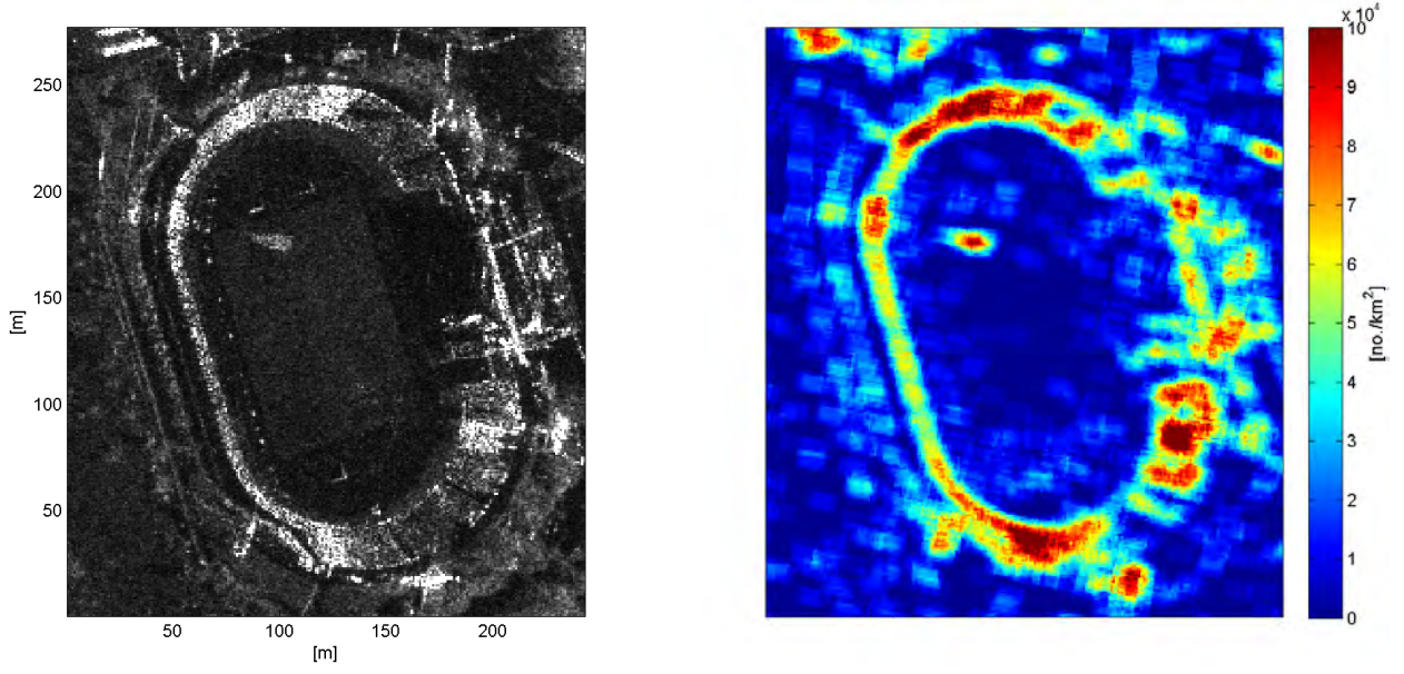
(a) Meanmap and density map of stack D36, HH.
