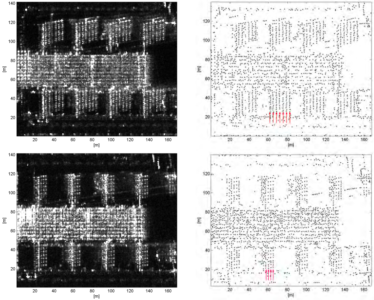
Figure 35. Second sample area for analysis on incidence angle influence. Left: Meanmaps of building at increasing incidence angles; top to bottom: Stack A42, A51, all VV); right: plot of detected PS positions (black dots). Note the loss of PS due to shadow effects, i.e., the reduction of 7 visible floors to 4 visible floors, indicated by red arrows.
