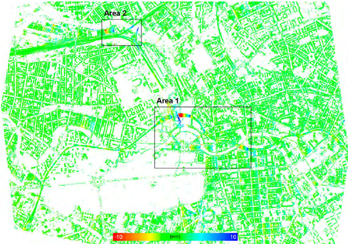
Figure 78. Top view on PS of Berlin test site colorcoded by the estimated seasonal components in west-eastern direction in the interval [-10, +10] mm.
