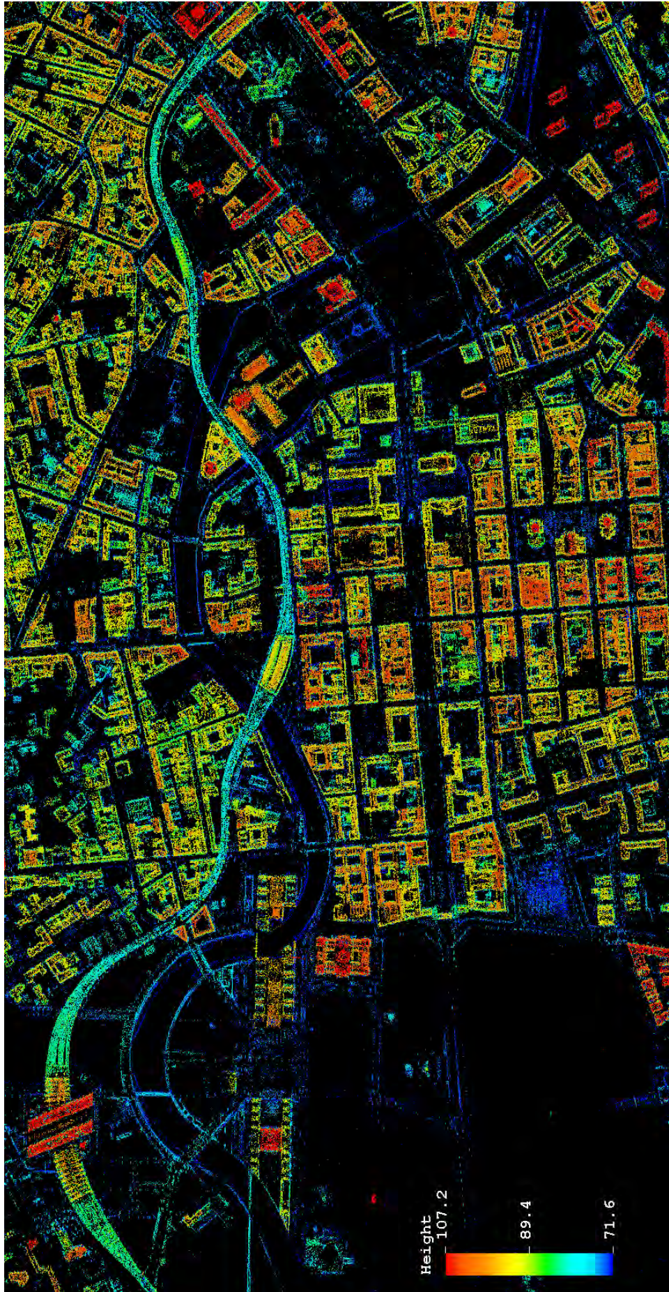
Figure 73: Top view on PS point cloud generated from fusion of 5 stacks of Berlin test site. PS are colorcoded by their height between approximately 72 m and 107 m. The outline of buildings is completed by the combination of ascending and descending stacks. The 3D information from the point cloud on the structure of the city becomes apparent. In addition deformations estimates are available for each single PS.
