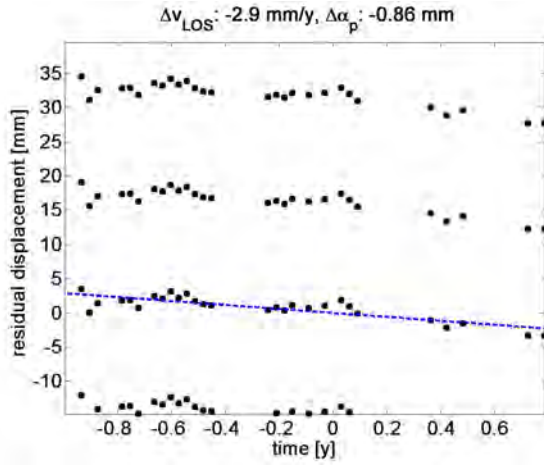
(a) Residual phase history for two PS at Berlin central train station.
