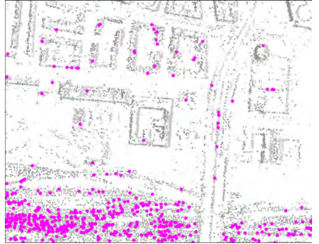
(c) Zoom to area 2 highlighted in Figure 71a.
