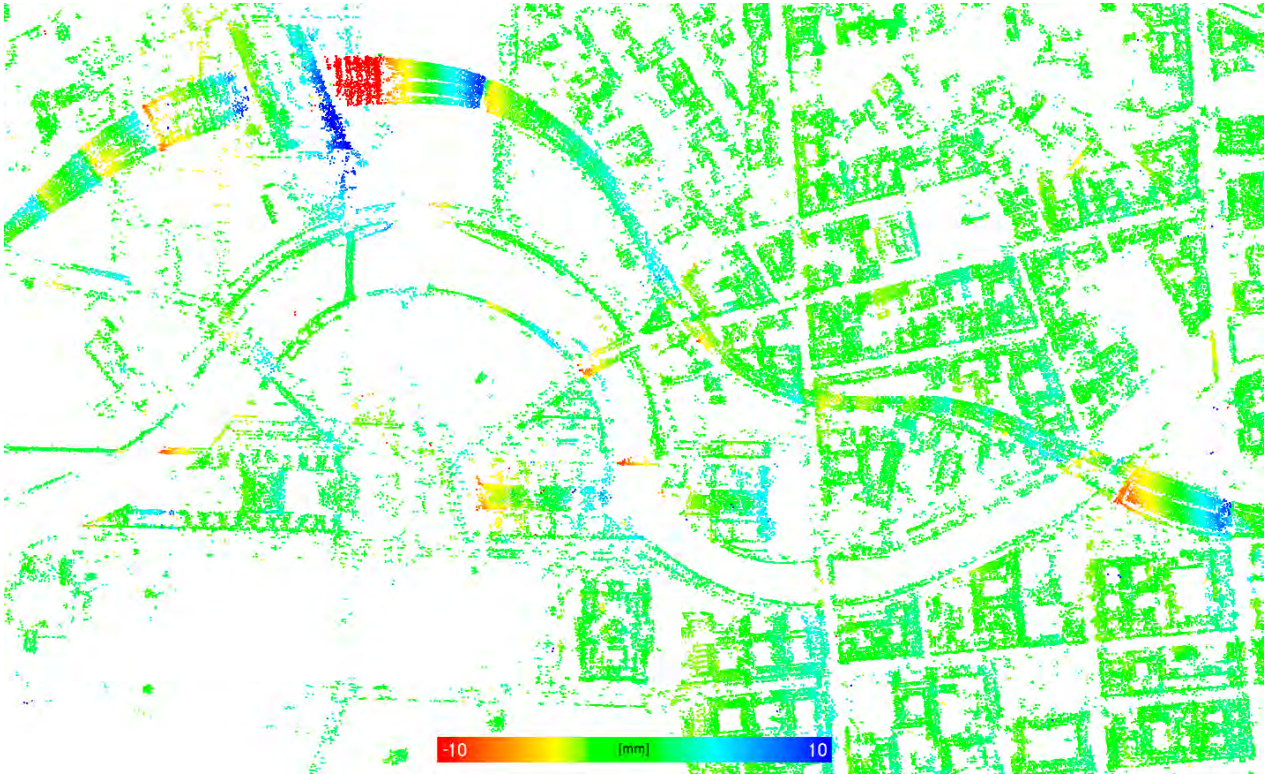
Figure 80. Top view on PS of area 1 in Berlin (cf. Section 4.4.2) colorcoded by the estimated seasonal components in west-eastern direction in the interval [-10, +10] mm.
