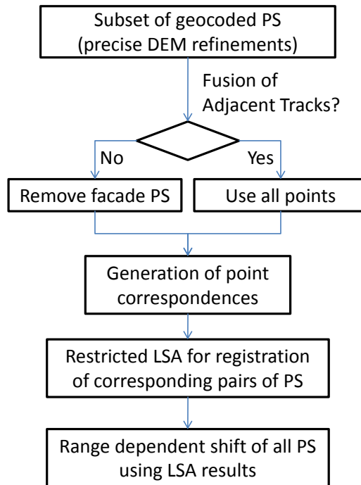
Figure 68. Flowchart of the proposed fusion algorithm.
