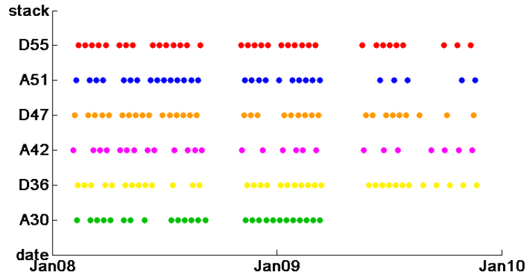
Figure 18. Acquisition time plot for Berlin test site showing temporal distribution of datasets.
