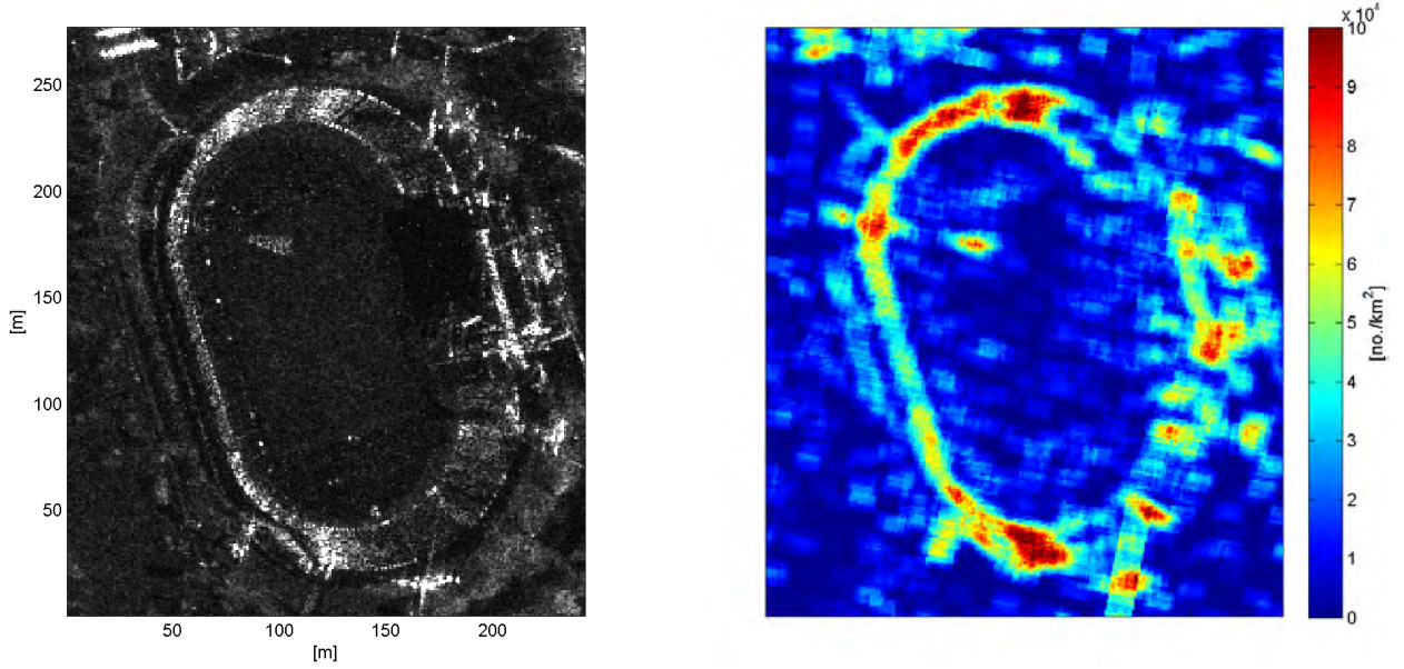
(b) Meanmap and density map of stack D36, VV.
