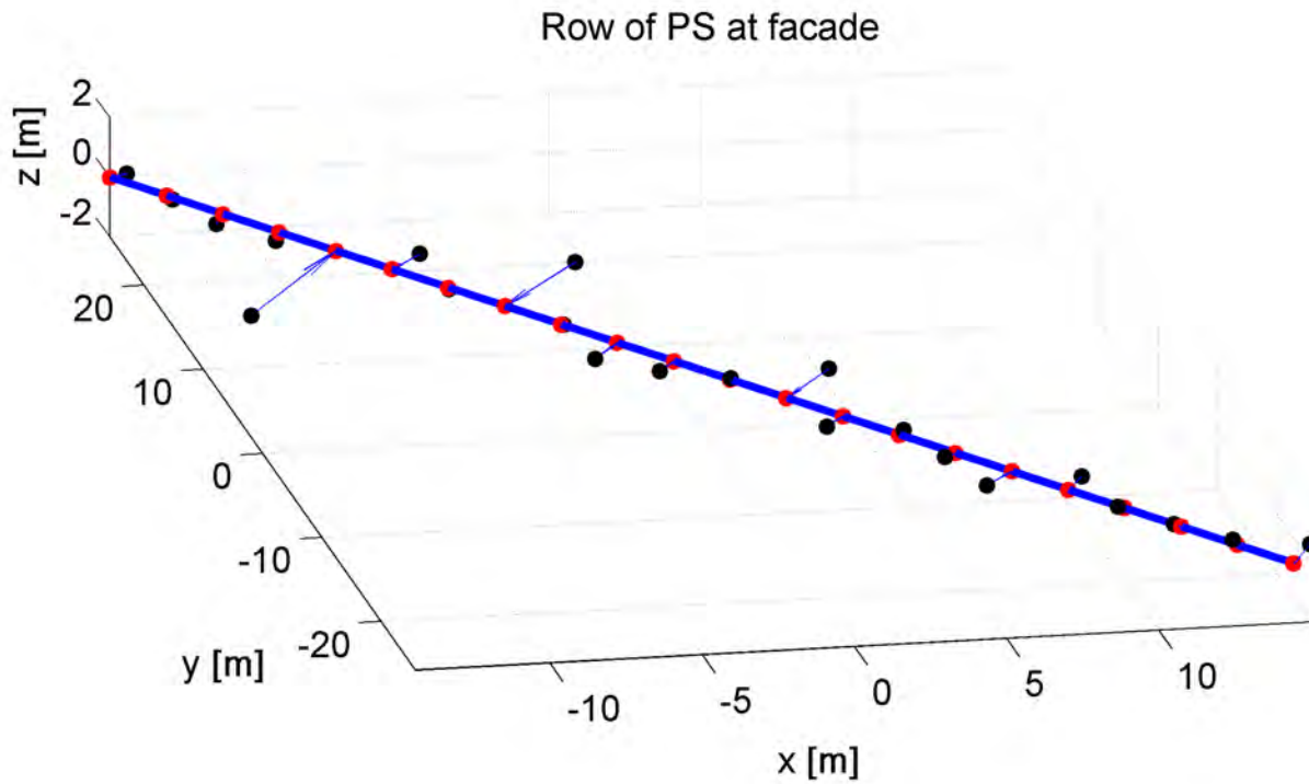
(b) View on PS positions from a different side compared to Figure 64a. The deviations of the geocoded PS in elevation become apparent. Blue arrows indicate necessary adjustments to PS positions in order to fit an equally spaced horizontal alignment.
