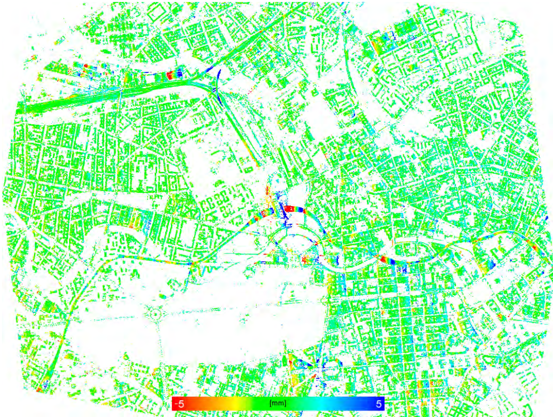
Figure 84. Top view on PS of Berlin test site colorcoded by the estimated seasonal components in west-eastern direction in the interval [-5, +5] mm.
