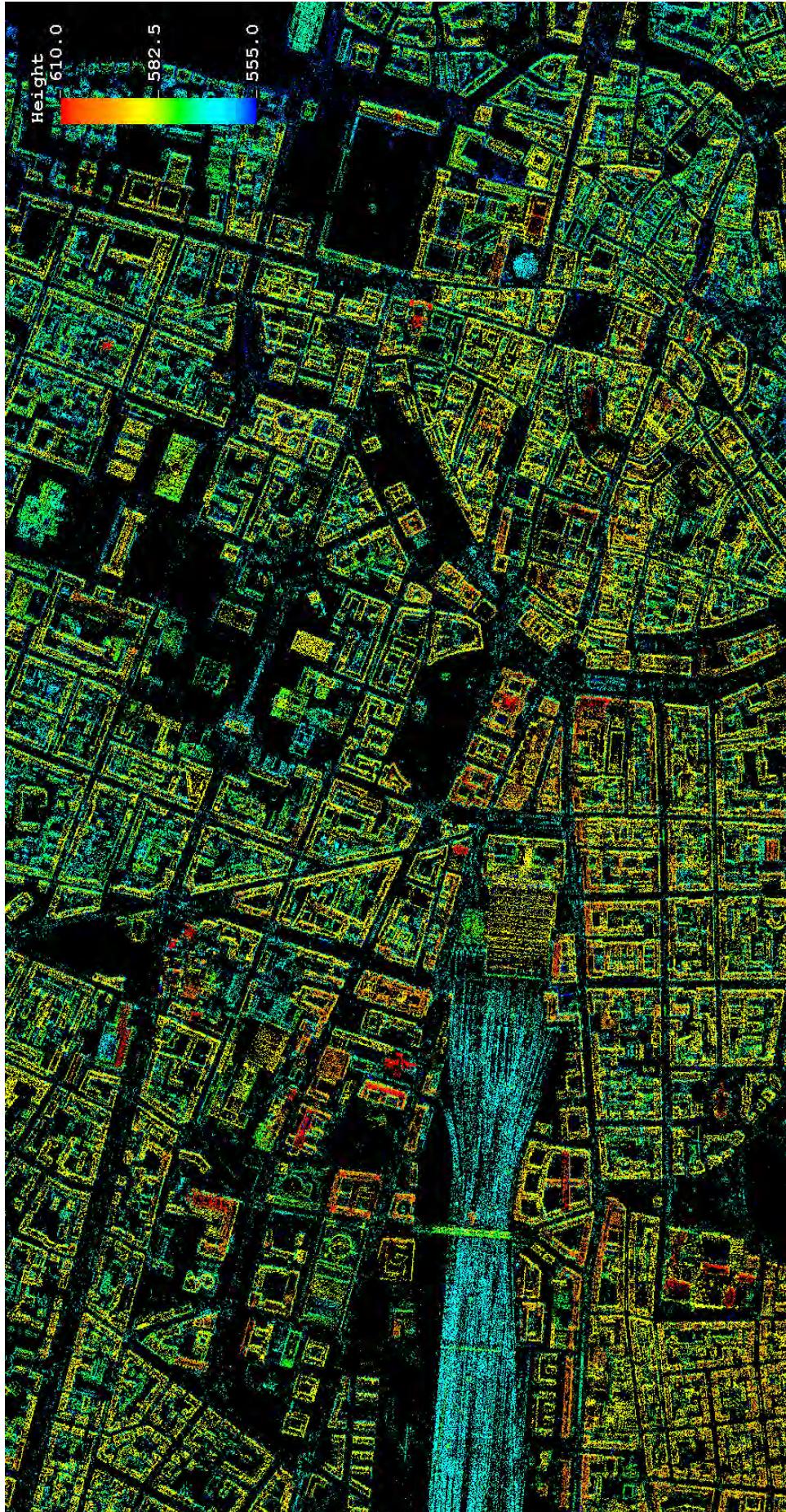
Figure 74: Top view on PS point cloud generated from fusion of 3 stacks of Munich test site. PS are colorcoded by their height between approximately 555 m and 610 m. The outline of buildings is completed by the combination of ascending and descending stacks. The 3D information from the point cloud on the structure of the city becomes apparent. In addition deformations estimates are available for each single PS.
