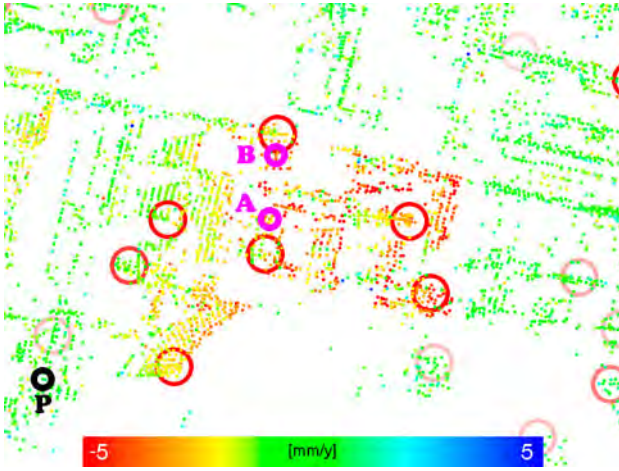
(a) Area 1 north-east of central train station in Munich (Sophienstrasse).
