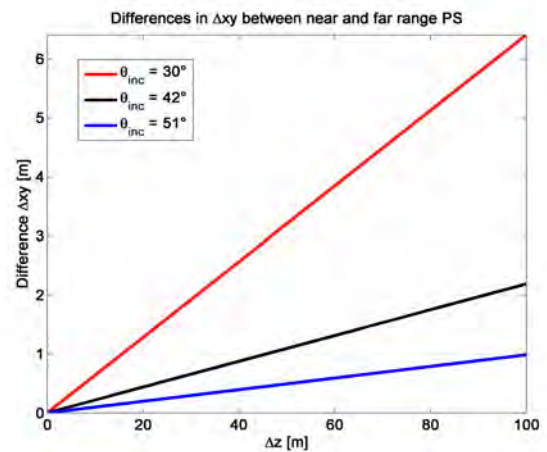
(b) Differences in horizontal shifts within one scene between PS at near and far range locations depending on the vertical offset \Delta z . Results for three typical stack parameters are given, indicated by different colors of mean incidence angle.
