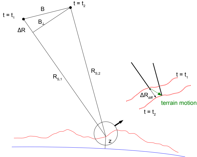
Figure 5. Influence of surface deformation on the interferometric phase. Change in range \Delta R_{diff} due to terrain motion between acquisitions at times t_1 and t_2
