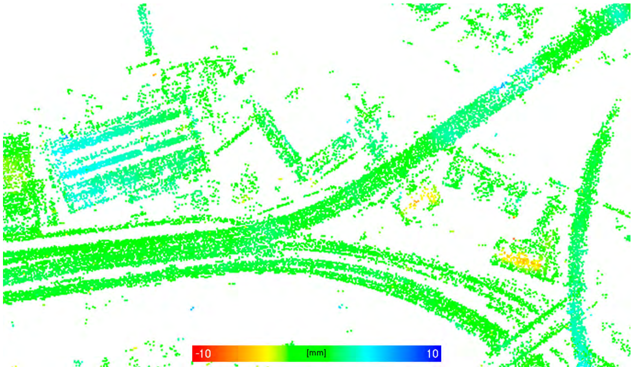
Figure 83. Top view on PS of area 2 in Berlin (cf. Section 4.4.2) colorcoded by the estimated seasonal components in vertical direction in the interval [-10, +10] mm.
