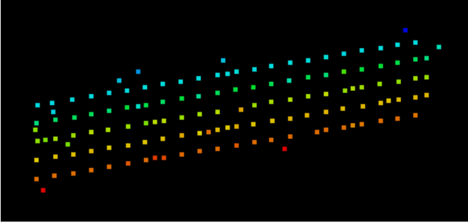
(a) Approximate clipping of point cloud to PS originating from building facade. Upper 5 floors show 22 linearly aligned PS each.
