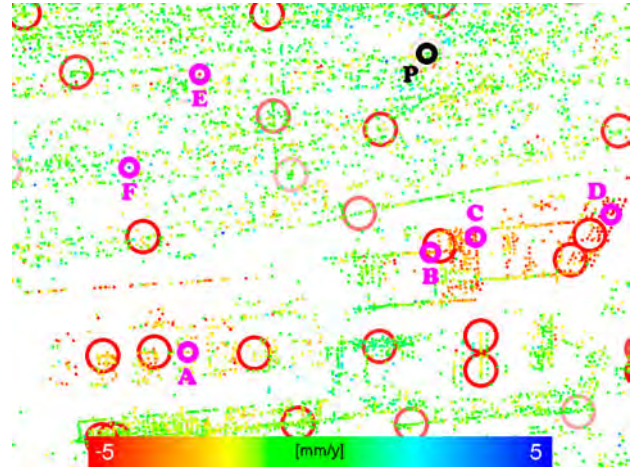
(b) Area 2 west of central train station in Munich (west of Hackerbrücke).
