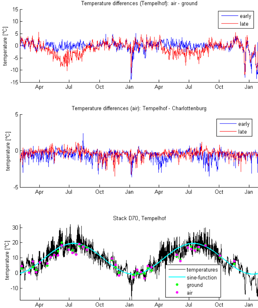
Figure 54. Top: Morning (early) and late afternoon (late) temperature differences between solid ground and air in 2 m above ground at measurement station Tempelhof. Middle: Morning (early) and late afternoon (late) temperature differences between two different locations within Berlin test site. One station is located in Charlottenburg, the other in Tempelhof. Bottom: Temperature history for station Tempelhof superimposed by a sine function fitted to the distribution. In addition, the temperatures of ground and air are indicated at the exact times of acquisitions for stack D70 by green and purple dots. Temperature data covering two years (starting January 2008) provided by FU-Berlin, Institut für Meteorologie.
