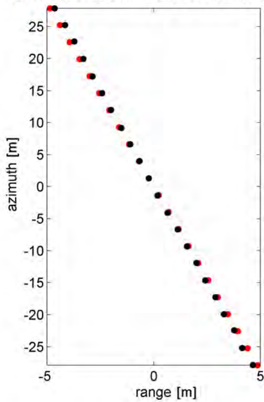
(a) View on PS positions in range-azimuth plane. Differences between adjusted and initial positions are very small.
