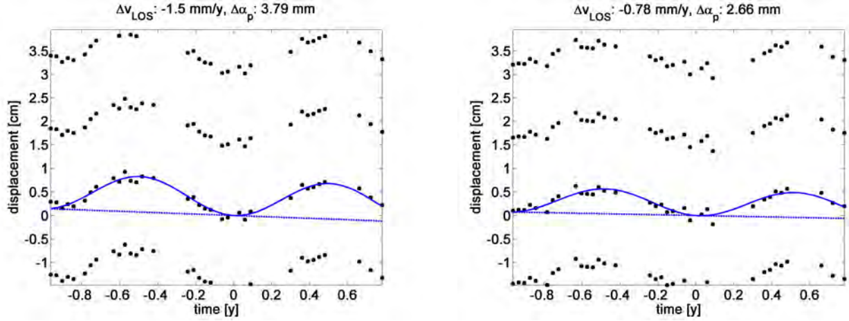
Figure 47. Phase history (including \pm 2\pi ambiguities) showing relative deformation rate between two PS of area 1. Black dots represent relative deformation signal. Blue line indicates estimated deformation. First number in title corresponds to estimated linear, second to amplitude of periodic deformation. Left: Dominating seasonal amplitudes of +3.79 mm (selection P1-A) and slight subsidence of -1.5 mm/y. Right: Dominating seasonal amplitudes of +2.66 mm (selection P1-B) and slight subsidence of -0.78 mm/y.
