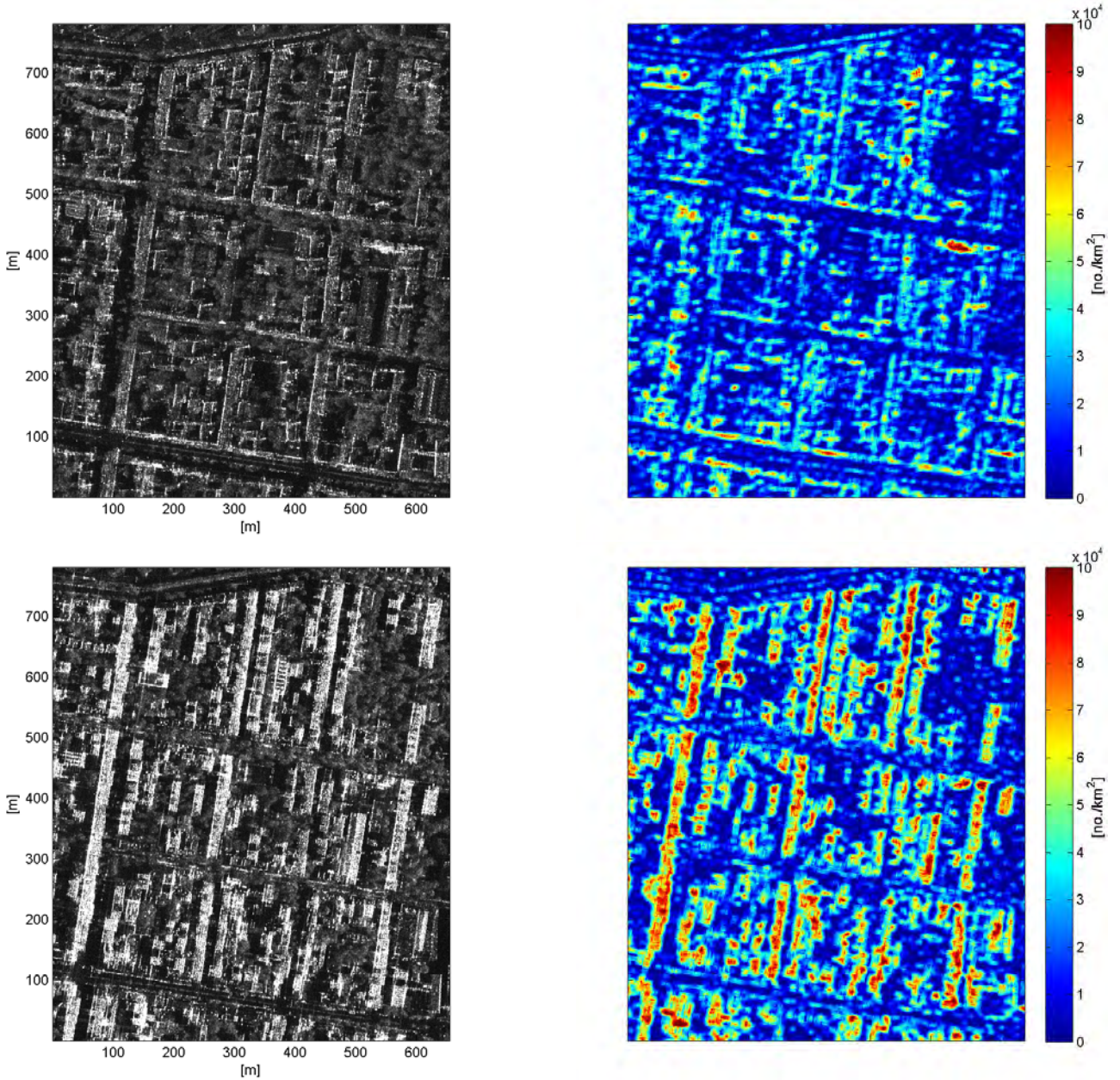
Figure 30. Meanmaps and density maps of sample area 3. Top: Meanmap and density map of stack A42, VV; bottom: Meanmap and density map of stack D47, VV. Colors indicate local densities up to 100,000 PS/km 2 (in red).
