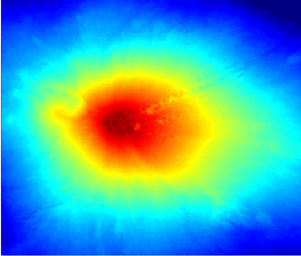
(c) Top view on the DEM of the volcano after phase unwrapping. Colors correspond to relative heights between 0 m (blue) and approximately 2600 m (dark red).
