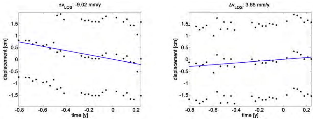
Figure 44. Phase history (including \pm 2\pi ambiguities) showing relative deformation rate between two PS of area 2. Black dots represent relative deformation signal. Blue line indicates estimated deformation. Left: -9.02 mm/y of subsidence (selection P-E). Right: +3.65 mm/y of uplift (selection P-F).
