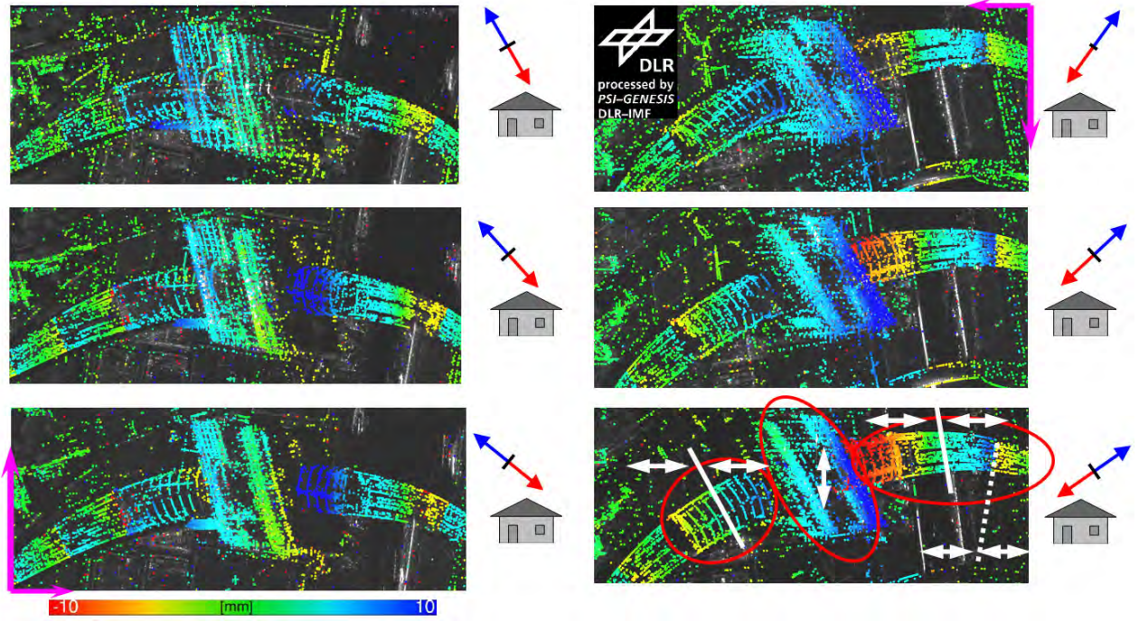
Figure 55. Estimated seasonal amplitudes at central train station obtained from each of the 6 stacks of Berlin. Left, top to bottom: Ascending stacks A30, A42 and A51. Right: Descending stacks D36, D47 and D55. Colors indicate amplitudes between -10 mm (red) and +10 mm (blue). Azimuth and range directions given by long and respectively short purple arrows at bottom left and top right. Houses and red-blue colored arrows indicate direction of motion with respect to LOS (side view on train station). White arrows show parts of dominating horizontal (left-right) and vertical (up-down) motion. White solid bars mark stable part, possibly fixed to ground. Dashed bar indicates position of rail tracks that are moving towards each other during summer times.
