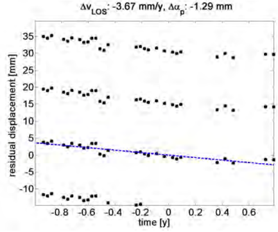
(b) Residual phase history for two PS within the area shown in Figure 87.
