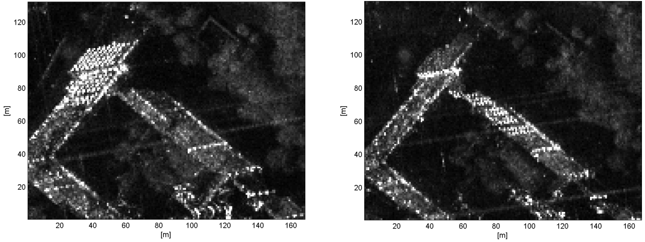
Figure 32. Sample area used for analysis on track direction. Left: Meanmap of stack A42. Right: Meanmap of stack A51.
