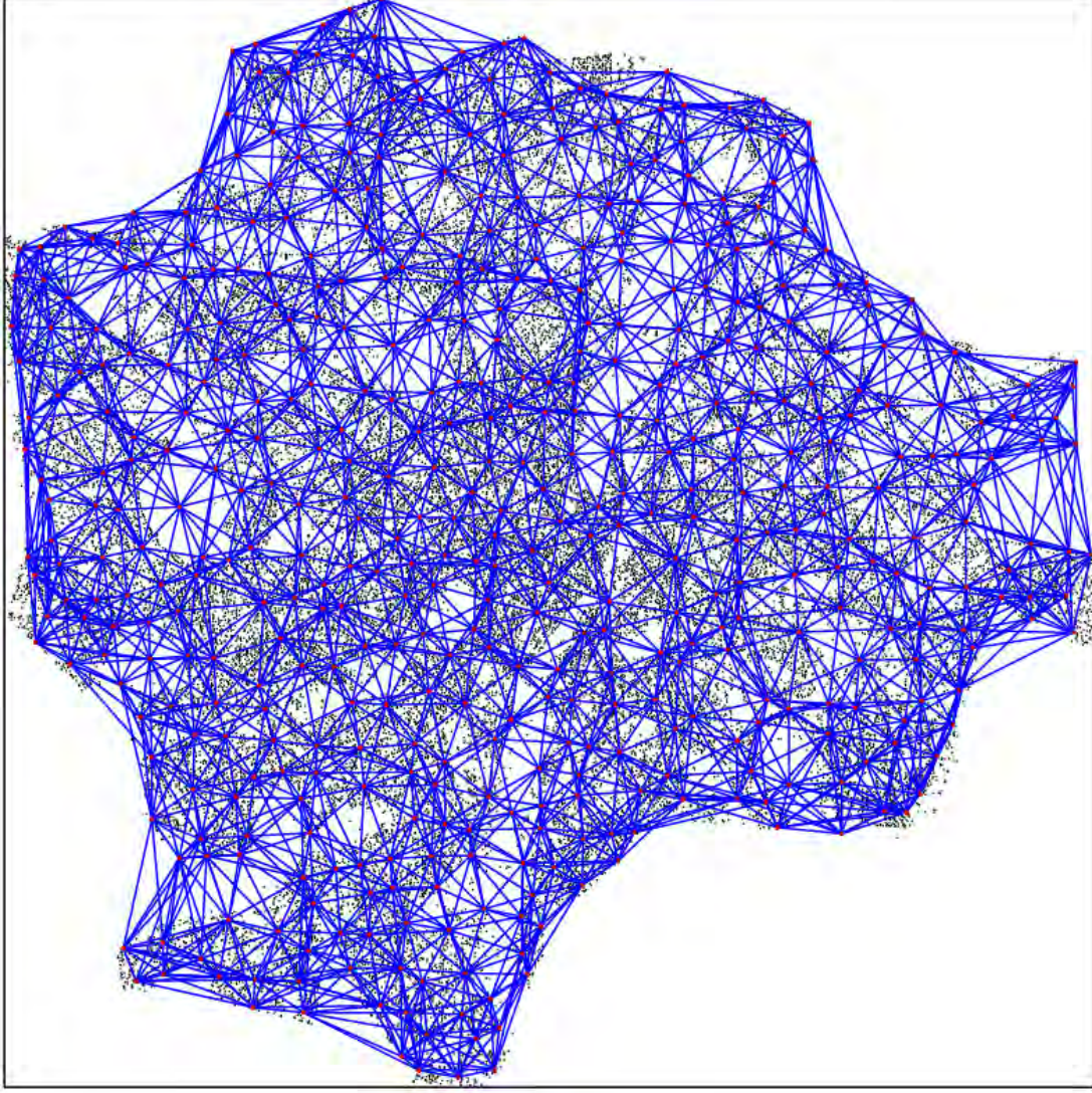
Figure 11. Reference network for the test site of Munich. Red dots represent PS of the reference network, black dots all remaining PS. For all arcs indicated in blue the parameters of deformation and DEM refinement are estimated separately.
