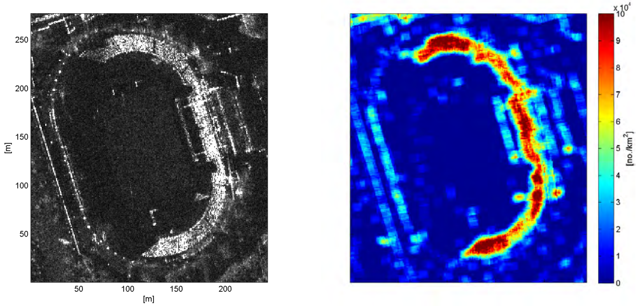
(a) Meanmap and density map of stack A51, HH.
