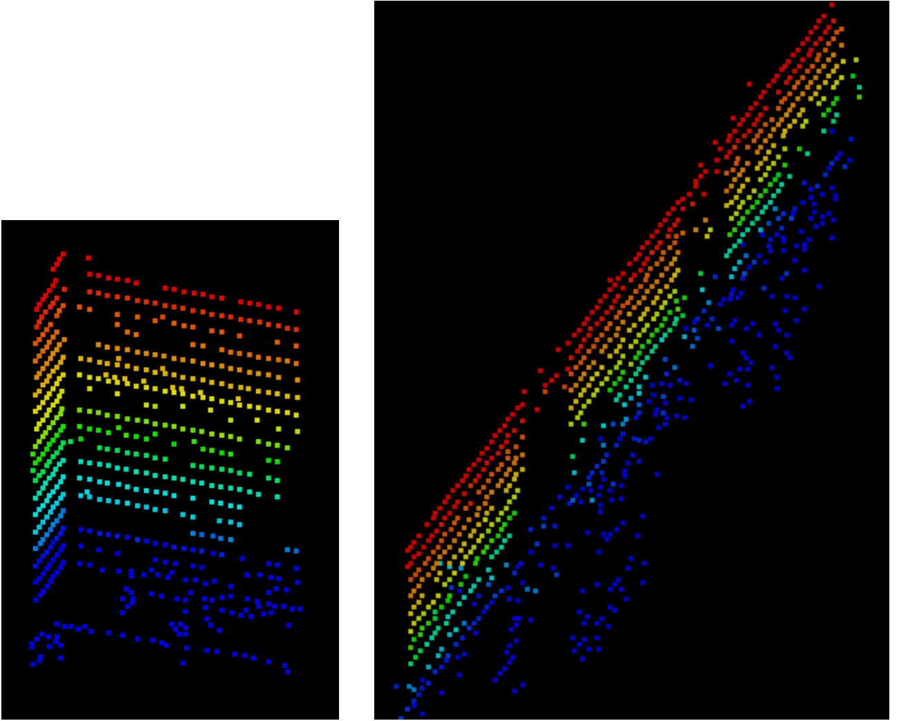
(a) PS originating from two facades of a skyscraper.
