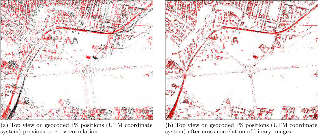
Figure 70. By reason of large vertical offsets the two stacks (one indicated in black, the other in red) show large horizontal separation (left). Point clouds shifted by results of refined cross-correlation show a good fit between both stacks (right). Therefore, corresponding close range pairs can be selected.
