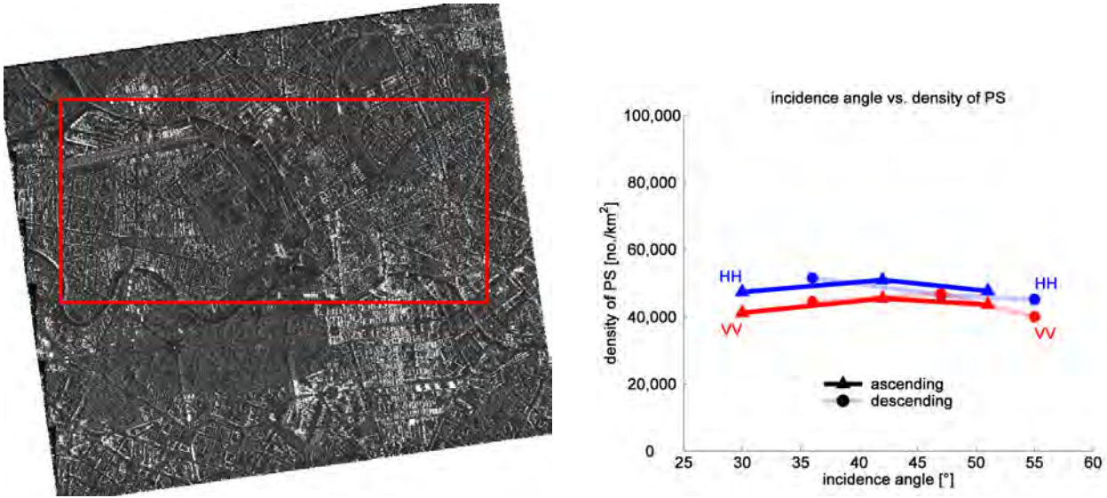
Figure 38. Large sample area for the analysis of PS densities (red rectangle). Left: Meanmap of stack A42. Right: Distribution of PS densities with increasing incidence angle. Different polarization indicated by different colors and by HH/VV signatures. Solid lines including triangular markers indicate ascending tracks. Diffuse lines including round markers indicate descending tracks. PS selection requirement: SCR \geq 3.0
