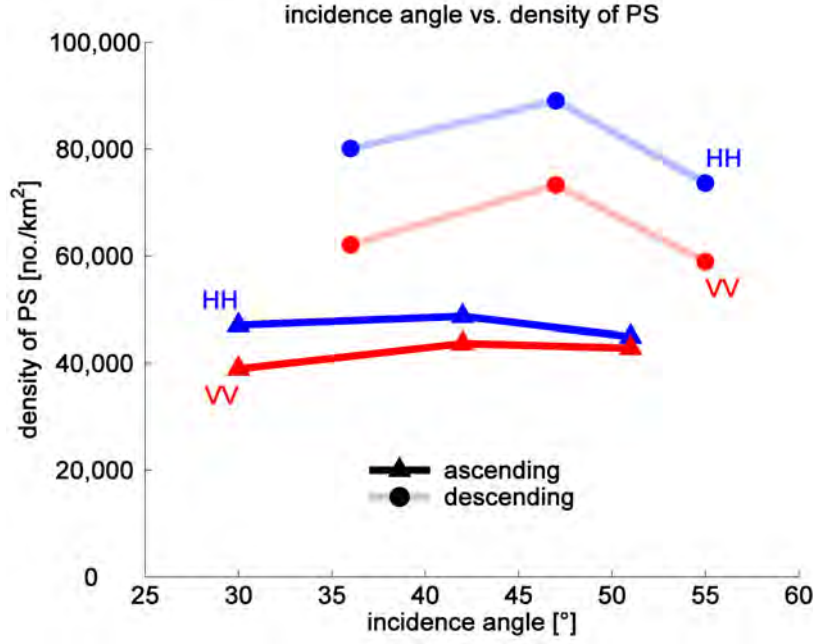
Figure 31. Distribution of PS densities with increasing incidence angle for sample area 3 shown in Figure 30. Different polarization indicated by different colors and by HH/VV signatures. Solid lines including triangular markers indicate ascending tracks. Diffuse lines including round markers indicate descending tracks. PS selection requirement: SCR \geq 3.0
