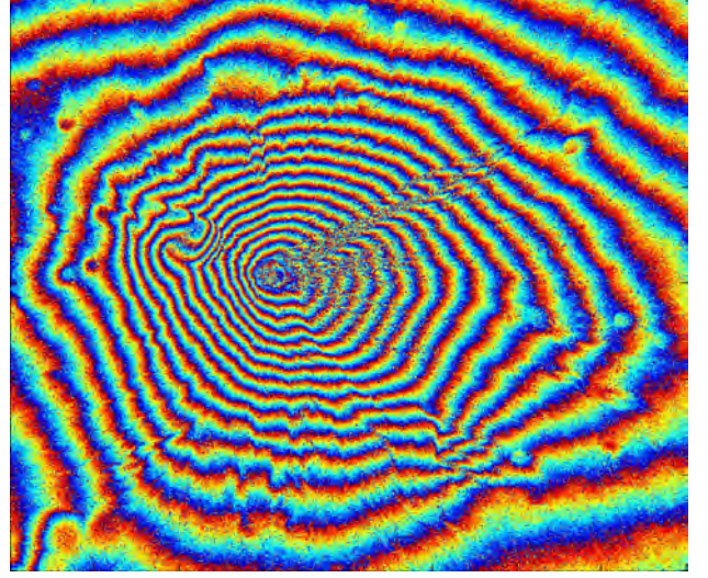
(b) Interferometric phase of the volcano after correction of the phase pattern induced by the reference surface (flat earth phase).
