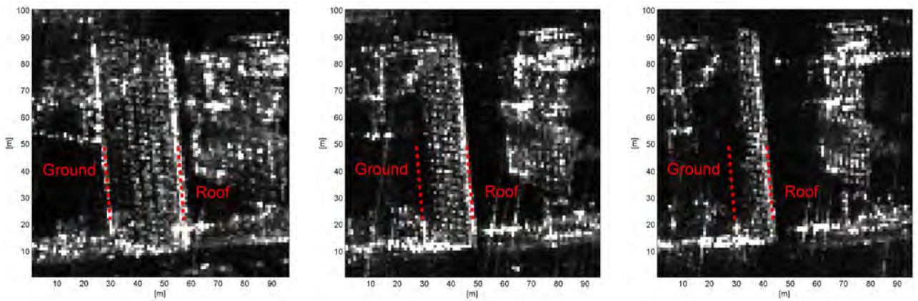
Figure 36. Third sample area for analysis on incidence angle influence. From left to right: Meanmaps of building at increasing incidence angles (Stack D36, D47, D55, all VV) heavily affected by shadow of the front building (situated to the right). Approximate location of ground and roof indicated by dashed red lines.
