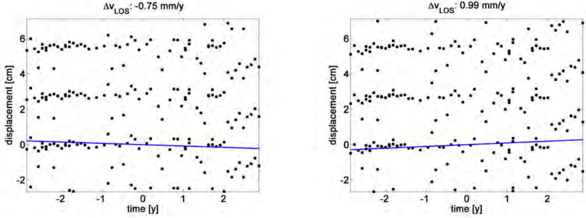
Figure 24. Comparison of deformation phase histories of one arc between both estimators. The estimated linear trend differs by 1.74 mm/y. The result of the periodogram (left) maximizes the ensemble coherence. However, the result of LAMBDA (right) seems to fit better. Black dots represent deformation phase (including \pm 2\pi ambiguities) after the removal of estimated relative height offset. Solid blue line indicates the estimated linear deformation.
