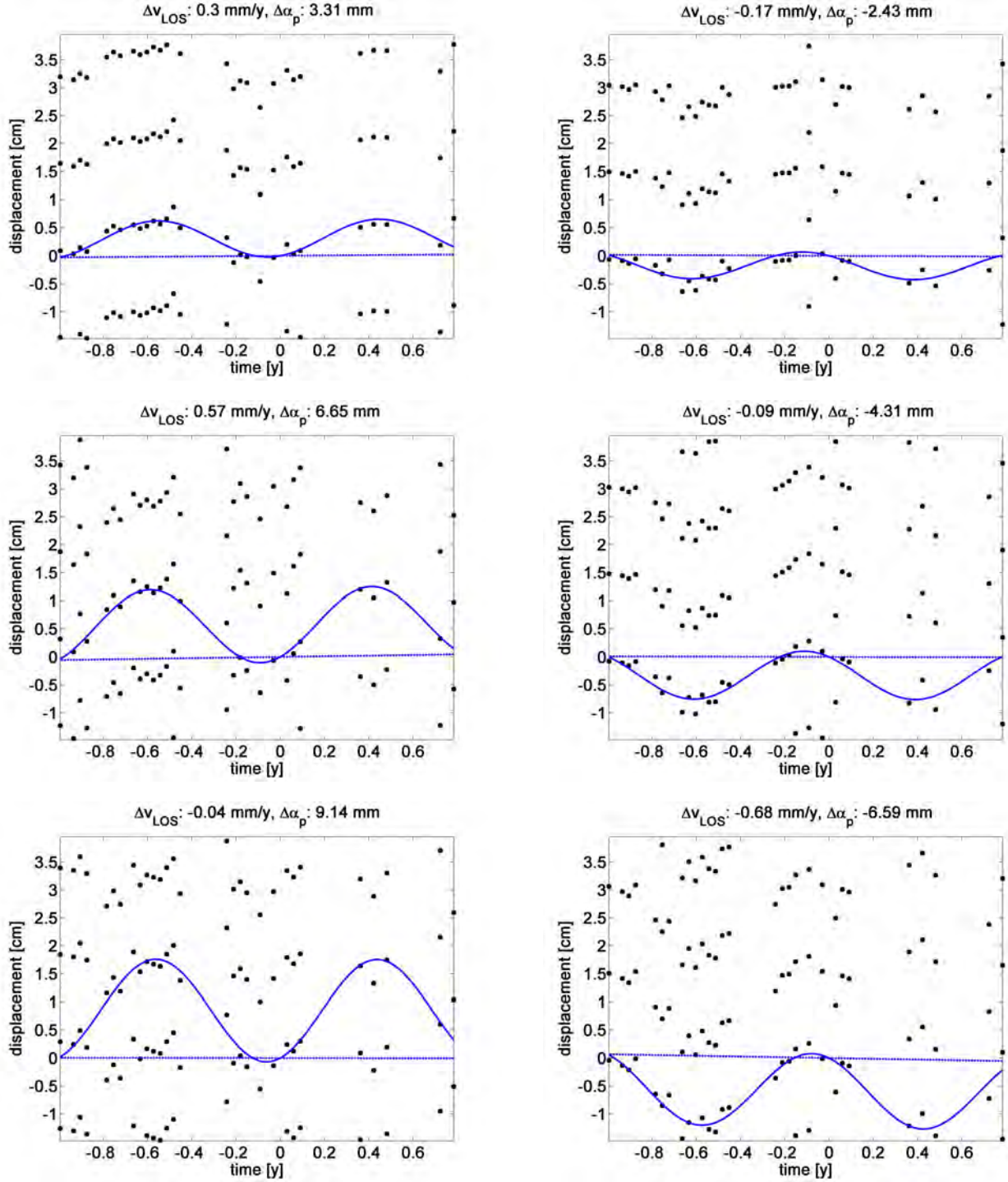
Figure 51. Phase histories (including \pm 2\pi ambiguities) showing relative deformation rate between two PS of area 1. Black dots represent relative deformation signal. Blue line indicates estimated deformation. First number in title corresponds to estimated linear, second to amplitude of periodic deformation. Left, top to bottom: Increasing positive amplitudes of seasonal motion of selection P-B, P-C and P-D up to +9.1 mm. Right, top to bottom: Increasing negative amplitudes of seasonal motion of selection P-E, P-F and P-G up to -6.6 mm.
