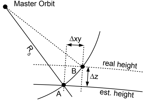
Figure 15. Principle of geocoding PS. The location of the point A in 3D can be obtained from an intersection of a circle, given by the orbital position of the master and precise range distance R_s , with the ellipsoidal height of each PS, given by the DEM and the estimated refinement. By reason of inaccurate DEM information for the reference PS, the point A may deviate from the real location B. In addition the the height offset \Delta z , a difference in horizontal positions \Delta xy is present.
