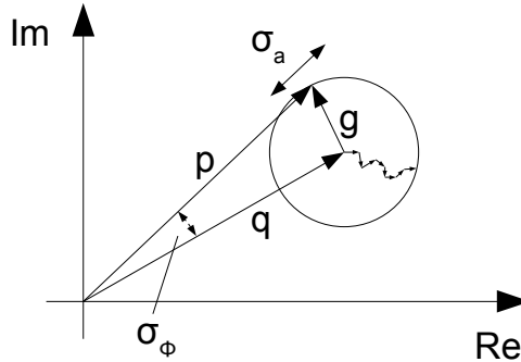
Figure 9. Observed signal p of a dominant scatterer q in clutter g within the resolution cell.
