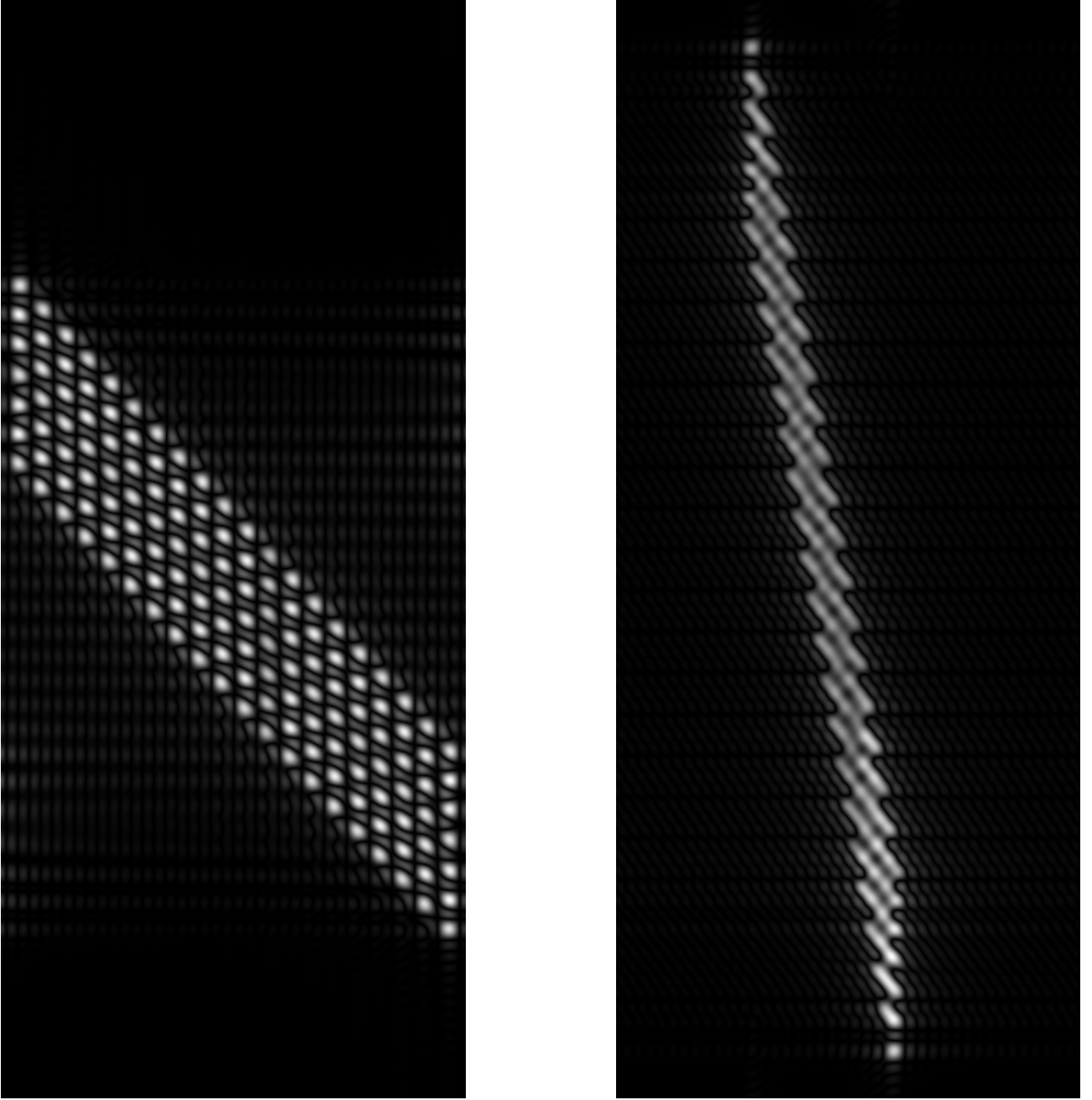
Figure 33. Simulated SAR images of a facade consisting of 21 windows in each row of 7 floors. The spacing between equal corners of the windows is set to 2.7 m. The radar resolution of TerraSAR-X is used for the simulation, whereas the images are oversampled by a factor of 8 for better visualization purposes. The incidence angle is set to 55^\circ . In the left image, the facade is rotated by 35^\circ with respect to an alignment perpendicular to ground range direction. The signatures corresponding to trihedral reflections at the windows can be separated easily, i.e., one PS per window is available. In the right image, the rotation angle is 75^\circ . In this case, the separation of all signatures is not possible any more. SAR images are generated using RaySAR. See Auer (2011) for more details on this simulation software.
