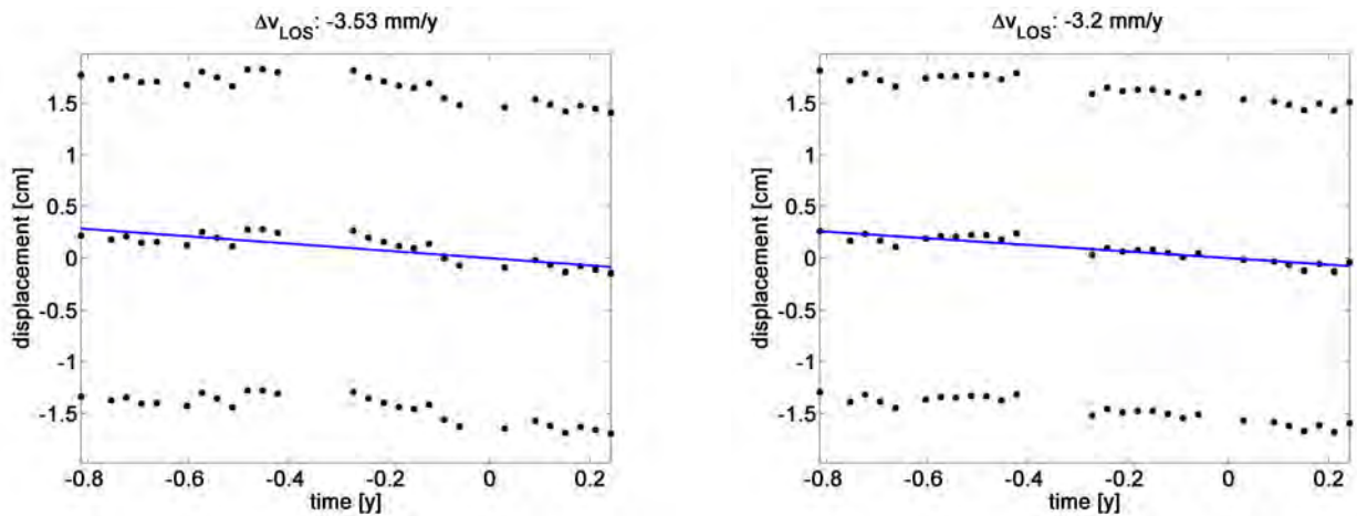
Figure 41. Phase history (including \pm 2\pi ambiguities) showing relative deformation rate between two PS of area 1. Black dots represent relative deformation signal. Blue line indicates estimated deformation. Left: -3.53 mm/y of subsidence (selection P-A). Right: -3.2 mm/y of subsidence (selection P-B).
