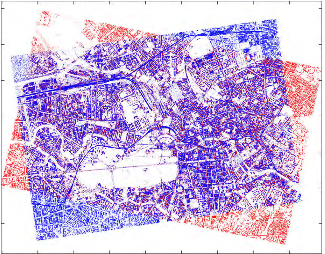
Figure 72. Fusion result of cross-heading tracks of the Berlin test site. PS of ascending track indicated in blue. PS of descending track plotted in red.
