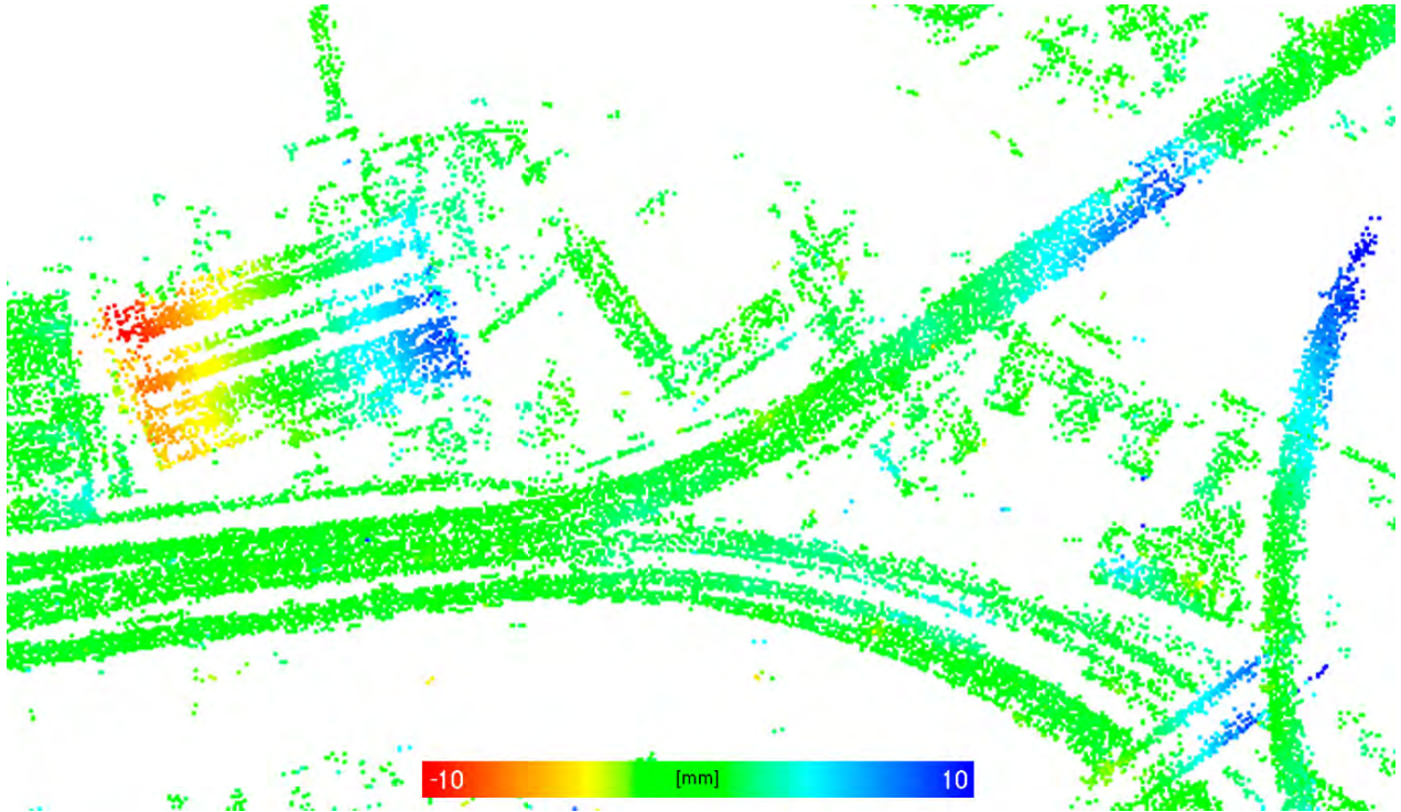
Figure 82. Top view on PS of area 2 in Berlin (cf. Section 4.4.2) colorcoded by the estimated seasonal components in west-eastern direction in the interval [-10, +10] mm.
