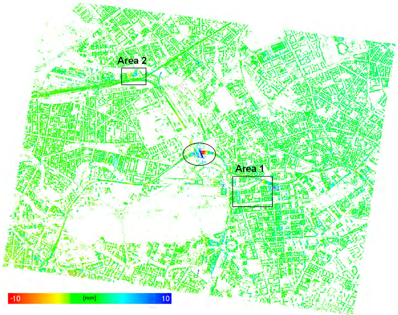
Figure 45. Results of seasonal deformation estimation for stack D55 in Berlin: Geocoded PS colorcoded by their amplitudes of motion between -10 mm (red) and +10 mm (blue) are shown. Green colors indicate no deformation. Several groups of PS can be identified showing significant seasonal displacement. Central train station is marked by circle. Areas 1 and 2 are investigated in more detail in this section.
