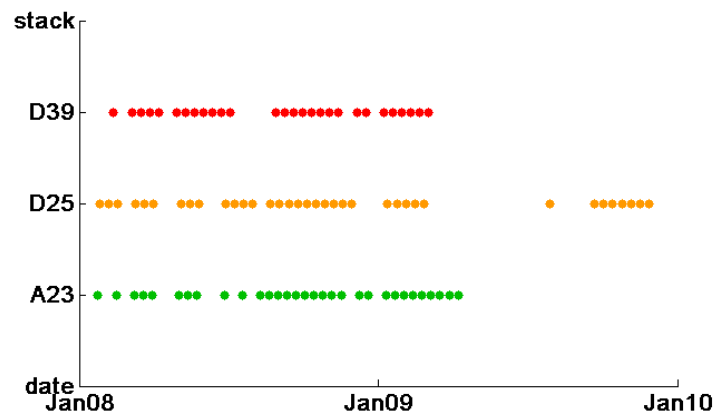
Figure 20. Acquisition time plot for Munich test site showing temporal distribution of datasets.
