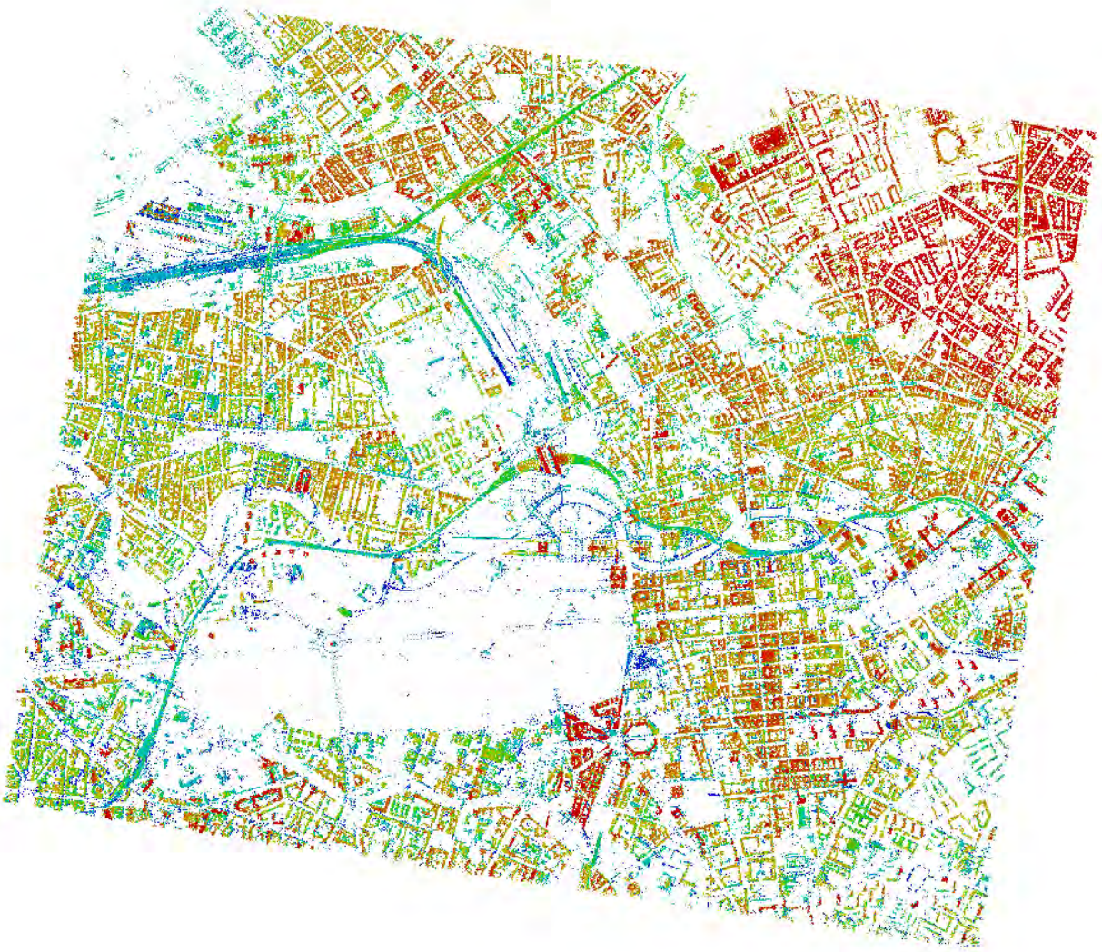
Figure 58. Top view on geocoded PS of stack D55, Berlin. Colors indicate relative height deviations from the chosen reference surface. Lower points in blue colors, higher points in red colors. Difference in height between limits is 35 m.
