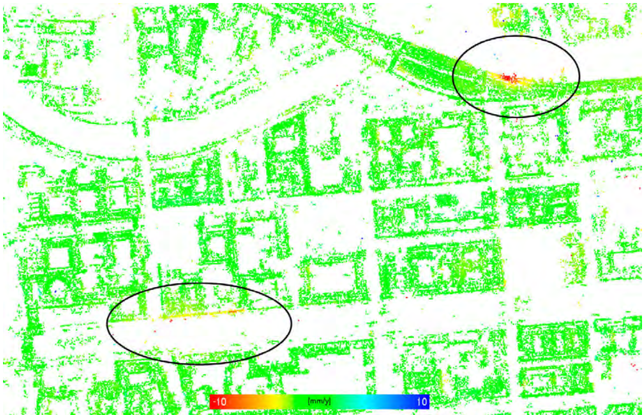
Figure 87. Top view on PS of Berlin test site colorcoded by the estimated linear components in vertical direction in the interval [-10, +10] mm/y. Significant subsidence is visible for two areas, highlighted by black ellipses.
