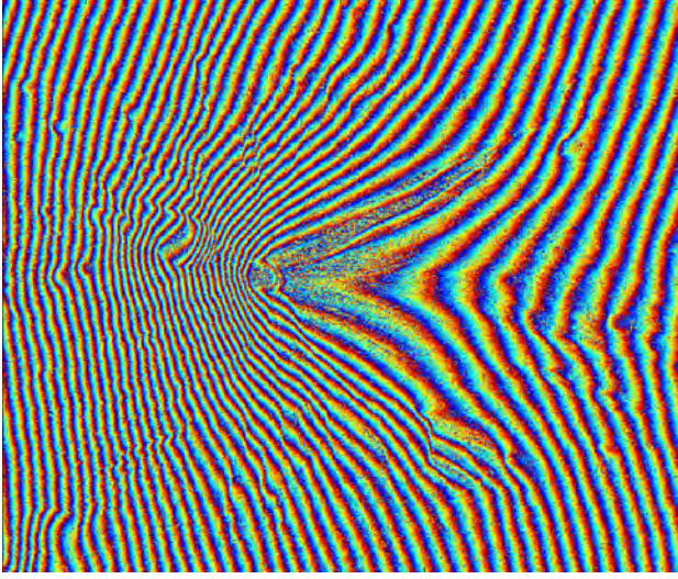
(a) Interferogram of a volcano including flat earth phase.
