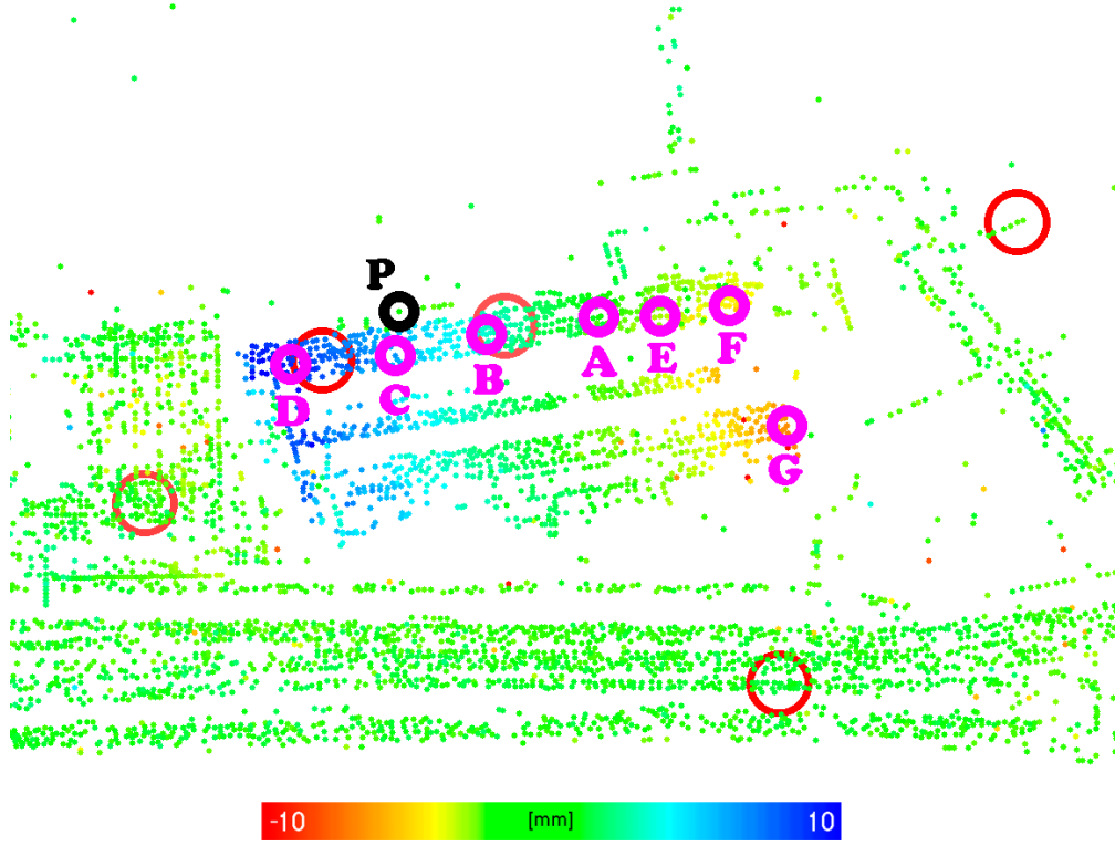
Figure 49. Sample location (area 2) 1.5 km north-west of central train station in Berlin (Friedrich-Krause-Ufer) showing larger deformation signals at final PS in Berlin. Circles indicate points of reference network, intensity of circle color shows deformation rate between 0 and 1 mm (intense red color) of periodic motion. Colors of points represent estimated seasonal amplitudes of deformation signal between -10 mm (red = subsidence in summer) and +10 mm (blue = uplift in summer) in LOS. Relative displacement in subsequent phase history plots between PS indicated by black (P) and each magenta (A-G) circle. Points are plotted in the azimuth-range plane.
