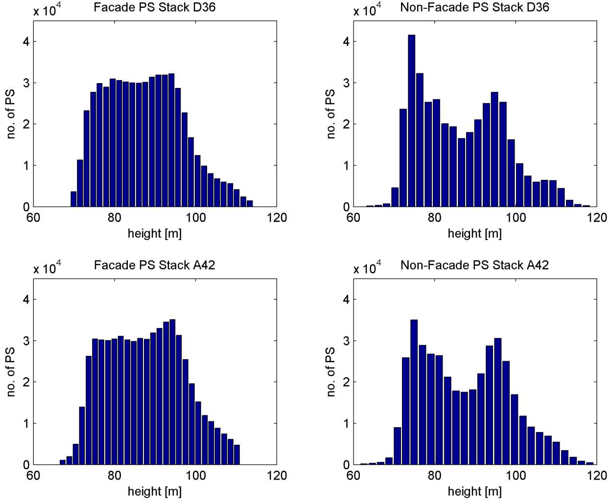
Figure 60. Histograms of PS absolute heights, geocoded to the UTM coordinate system of stacks D36 and A42. The unknown height offsets are already fixed (see Section 5.2). The left column shows the graphs of potential facade PS. On the right hand side the distribution of the remaining PS heights is plotted. The two peaks indicate approximately the heights of ground surface (first peak) and the roofs of a majority of houses (second peak). This interpretation is facilitated by the almost horizontal ground surface in Berlin.
