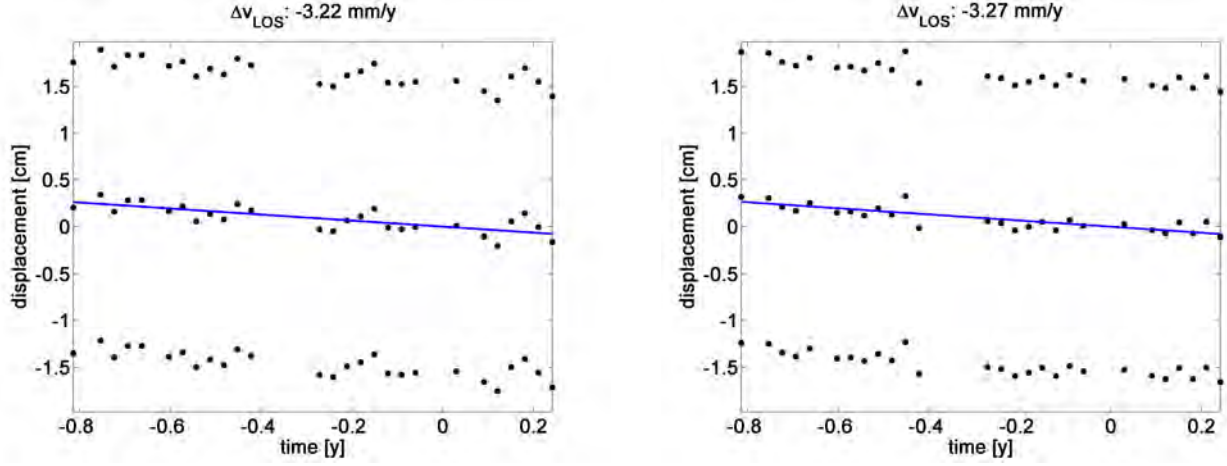
Figure 42. Phase history (including \pm 2\pi ambiguities) showing relative deformation rate between two PS of area 2. Black dots represent relative deformation signal. Blue line indicates estimated deformation. Left: -3.22 mm/y of subsidence (selection P-A). Right: -3.27 mm/y of subsidence (selection P-B).
