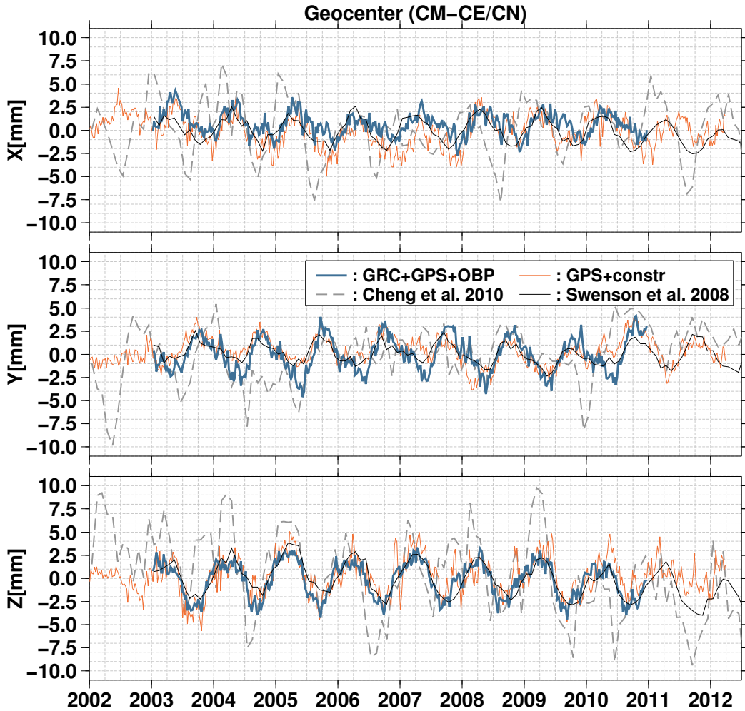
Figure 5.1: Time variation of the Cartesian components of the geocenter motion ( \mathbf{x}_{CM} - \mathbf{x}_{CE} ) for different estimates. The time series are relative to the release 05 Ocean-Atmosphere (GAC) product. The SLR based series represents the offset relative to the SLR network origin.
