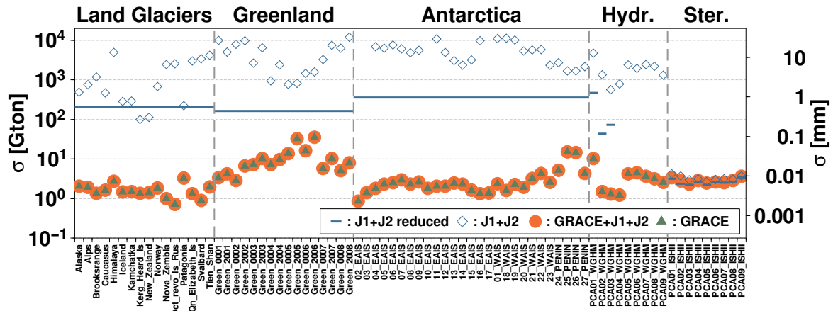
Figure 4.19: Monthly formal errors of the fingerprint inversion (September 2008), for several combinations of Jason-1, Jason-2, and GRACE. The solution of the ‘reduced’ altimetry-only inversion contain the total effect of Greenland, Antarctica and the land glaciers as single parameters, and the first three hydrological modes. All errors are expressed in terms of their ocean mass change and eustatic sea level contribution.
