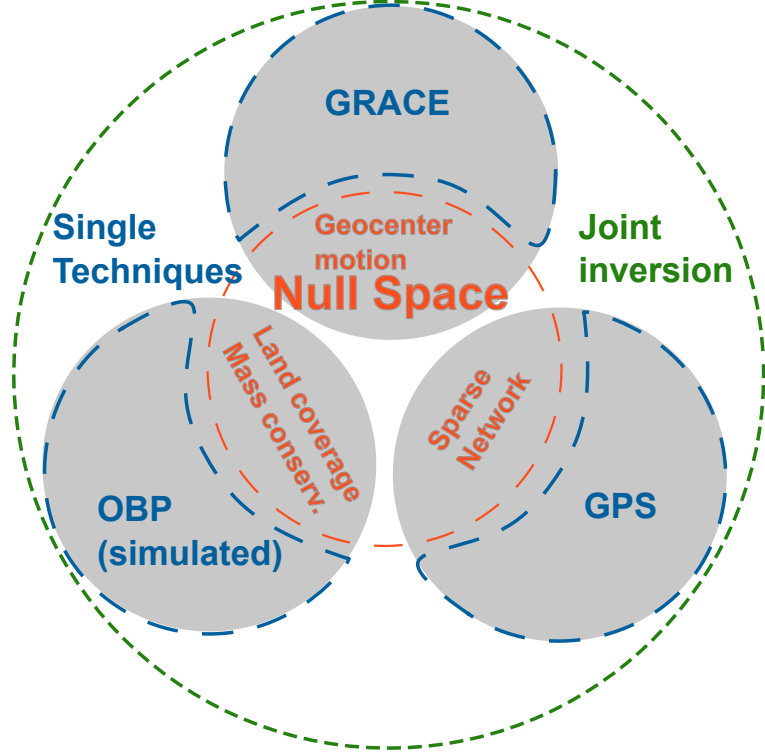
Figure 4.1: The joint inversion scheme allows resolving parts of the solution space, which could not have been resolved by single techniques alone (the null-space). For example, geocenter motion, unresolved by GRACE is constrained by GPS and the simulated OBP. On the other hand, regions not covered by GPS may be effectively constrained by GRACE and OBP. In addition, mass corrections for the model are resolved by GPS and GRACE.
