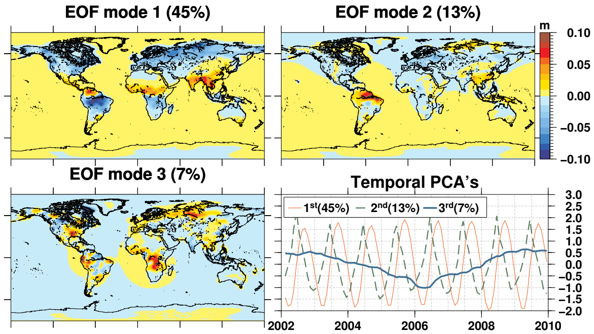
Figure 4.16: The self consistent surface load as computed from the first three hydrological EOFs from WGHM (Döll et al., 2003), and the associated time variations of the principal components. The sign of the modes is adapted such that each EOF is associated with a positive contribution to the ocean.
