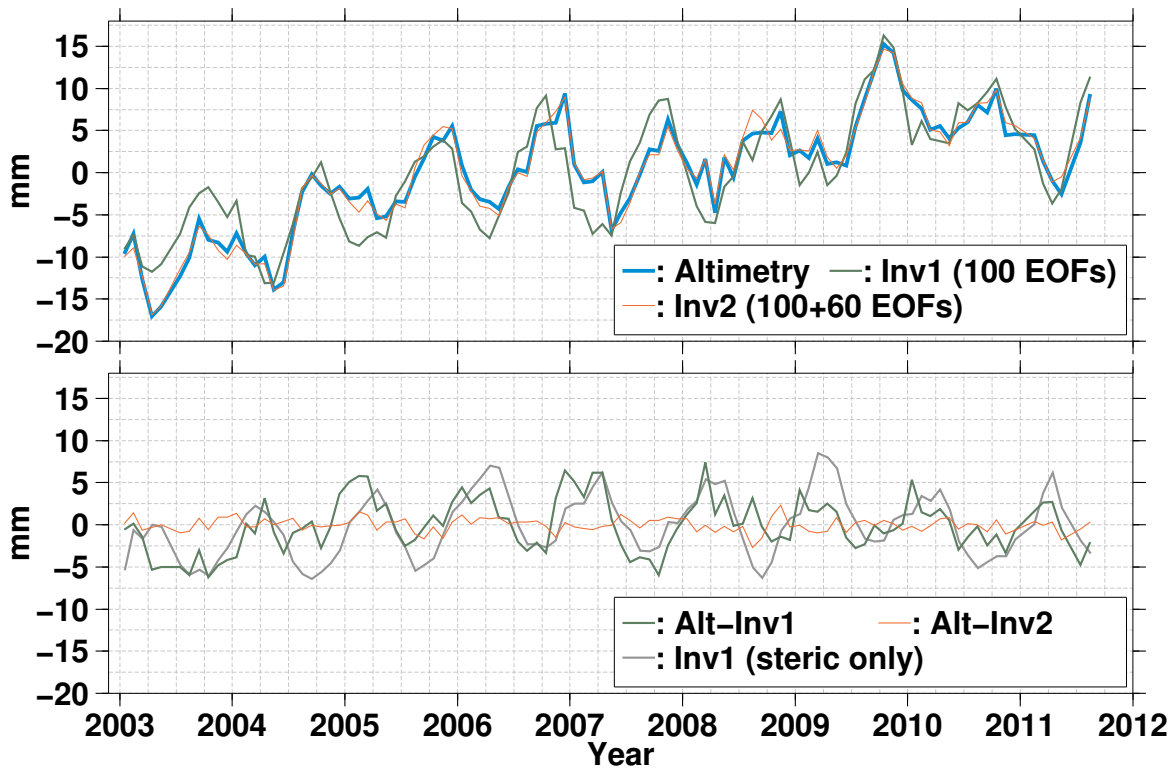
Figure 4.15: Geocentric mean sea level of the altimetry and residual
