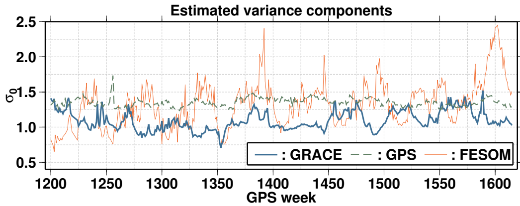
Figure 4.2: Estimated variance components, \sigma_0 , of the joint inversion of GRACE (RL05), GPS and FESOM data.
