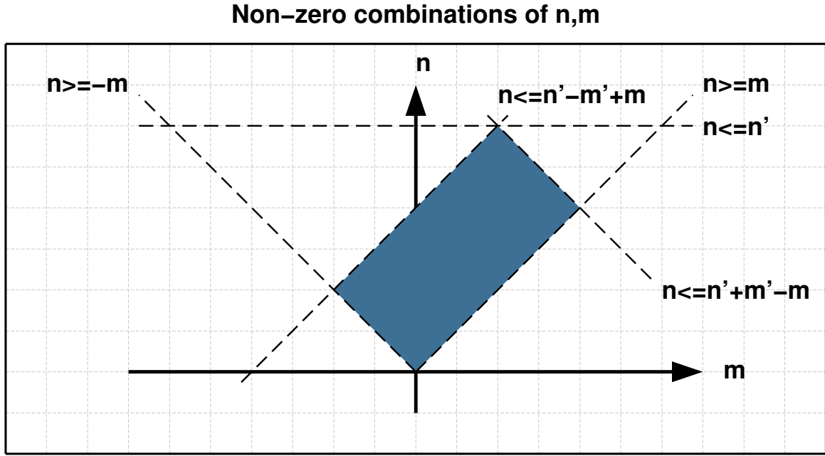
Figure A.1: Obeying four constraints, the double summation from Eq. A.9 will only yield non-zero combinations for n and m in the shaded area.
