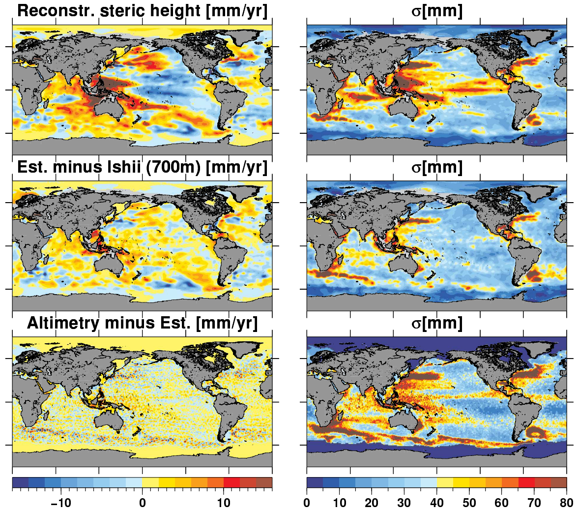
Figure 5.22: Reconstructed steric sea level trend and the standard deviation of the residual (after removing the mean, trend and annual harmonic curve per grid point). The middle plots shows the trend and standard deviation of the reconstructed steric sea level but now with the gridded steric height from the upper 700m of Ishii and Kimoto (2009) removed. The bottom plots display the trend and the standard deviation of the altimetric residual after removing the total fit (mass-induced, GIA and steric sea level and the effect of the nuisance parameters).
