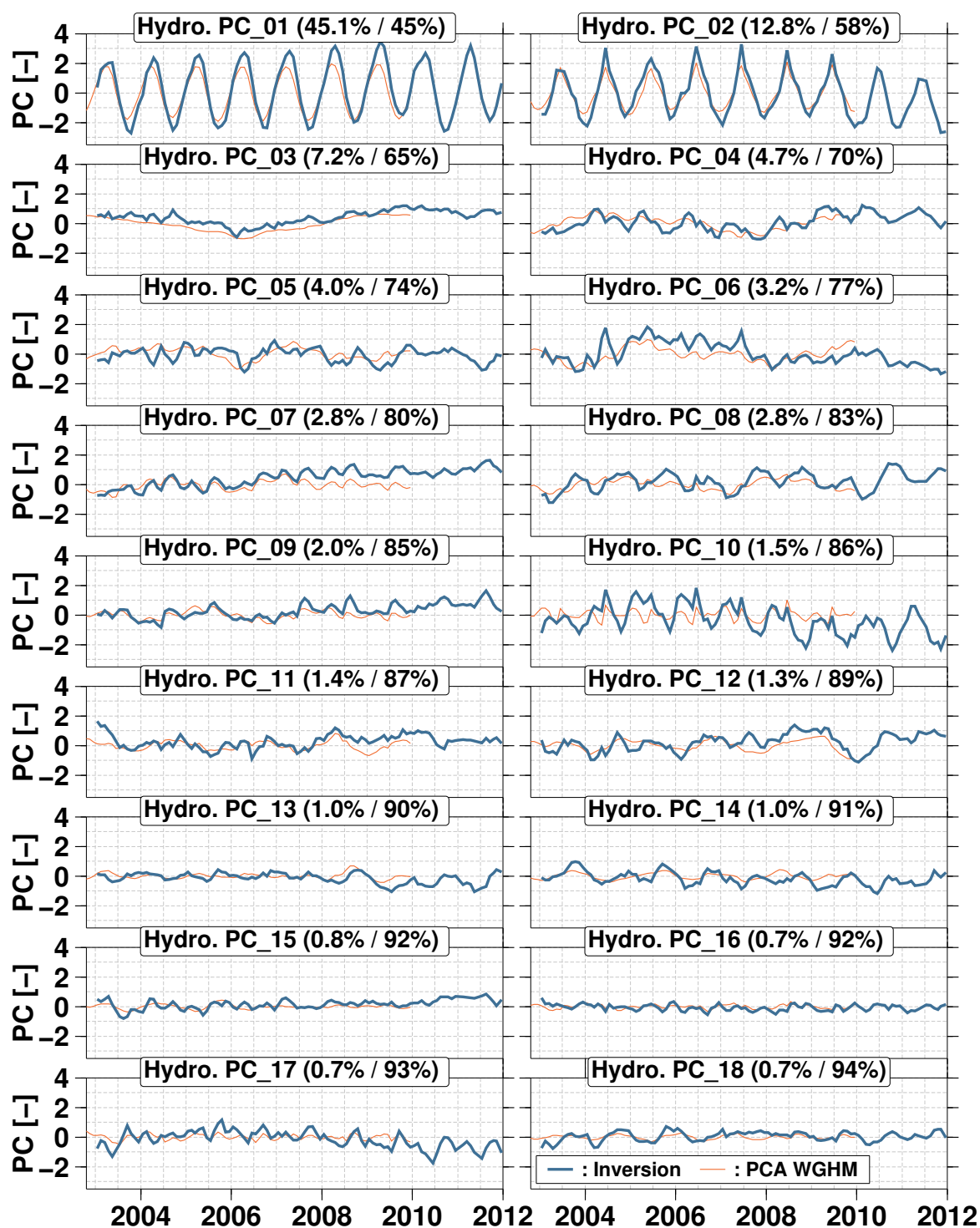
Figure 5.19: Time variation of the first 18 principal components of the changes in terrestrial total water storage. The scales, as estimated by the inversion, are plotted along the principal components which were computed from the PCA of the dataset from WGHM Döll et al. (2003). The percentages denote the variance explained (per mode/cumulative).
