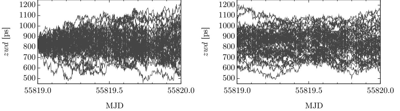
Figure 5.19: 50 realizations of the simulated zenith wet delay for the station in Kokee Park for the first 24 h of the CONT11 campaign. Left without forerun of the simulation, right with a forerun of 12 h.
