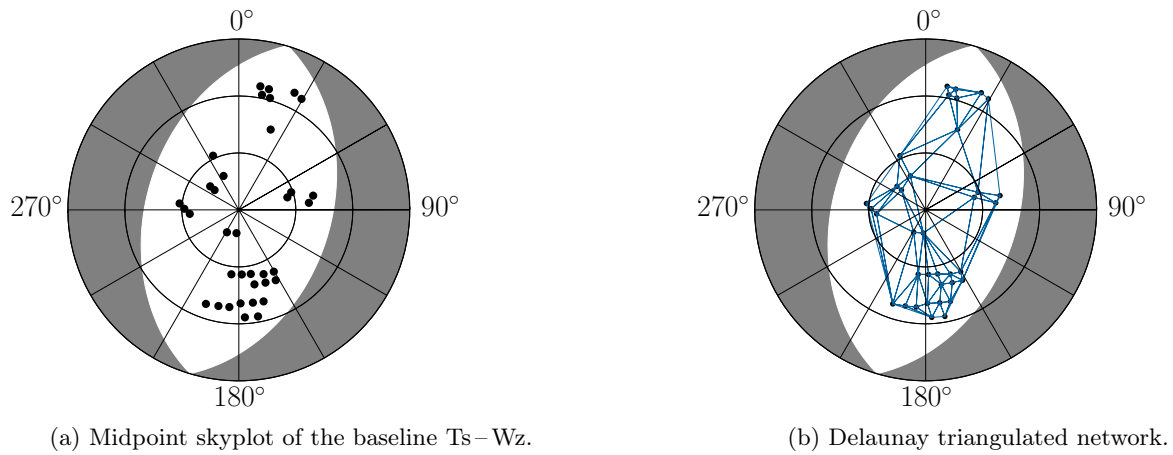
Figure 5.6: A midpoint skyplot of the baseline Tsukuba – Wettzell showing the observed sources of a typical IVS-INT2 session (a) and its Delaunay triangulated network (b).
