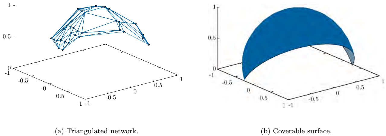
Figure 5.7: Three-dimensional depiction of the triangulated network shown in Fig. 5.6b (a) and three-dimensional depiction of the coverable surface for the baseline Tsukuba – Wettzell (b).
