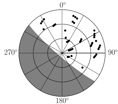
Figure 5.5: Skyplot of the station Wettzell of an INT2 session with the gray area being the unscannable sky area of the partner telescope in Tsukuba.
