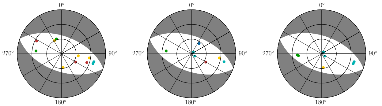
Figure 3.13: Observations with high impact factors for \Delta UT1 (left), at_A (middle) and at_B (right) for the examined INT1 session (I12010).
