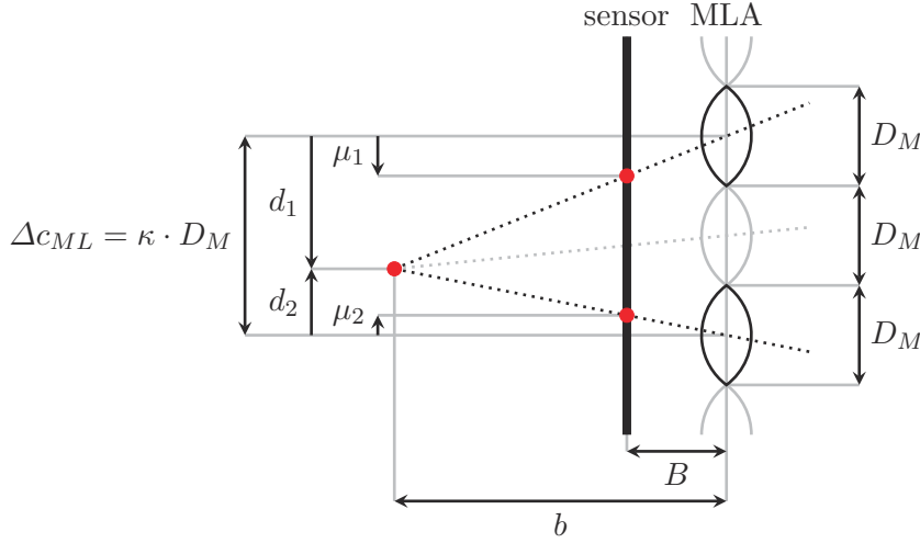
Figure 2.8: Depth estimation in a focused plenoptic camera based on the Galilean mode. The distance b between a virtual image point and the MLA can be calculated based on its projection in two or more micro images.
