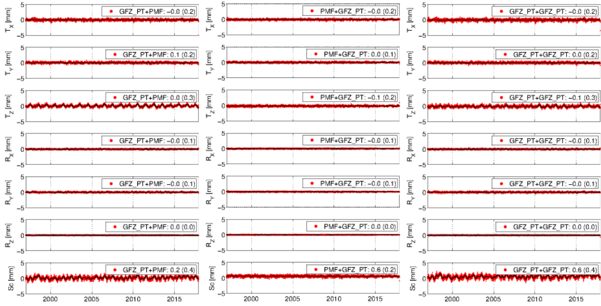
Figure 6.3.1: The time series of a 7-parameter similarity transformation between the ensemble mean of the solution where GFZ-PT served as mapping functions (left), the solution where GFZ-PT was used to calculate the d_h^z (middle), and the solution where GFZ-PT was used for m_{fh} , m_{fnh} , and d_h^z (right), with respect to the GNSS solution where no systematic errors were simulated. In the legend of these graphs, the average offset appears, as well as the WRMS of a straight-line fit, enclosed in parenthesis.
