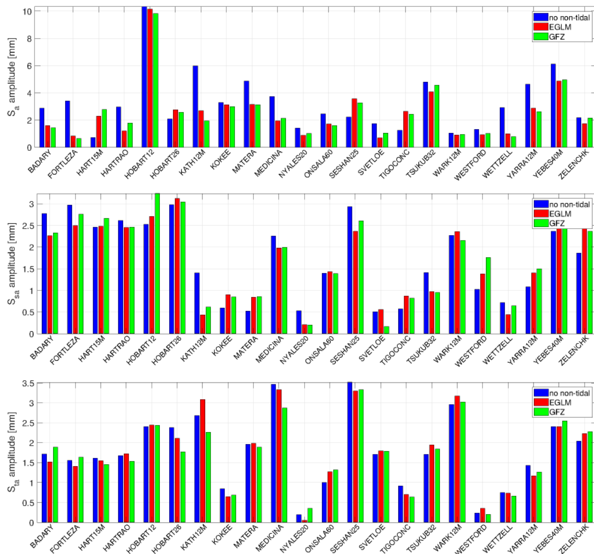
Figure 7.1.1: The S_a (1 st row), S_{sa} (2 nd row), and S_{ta} (3 rd row) amplitudes of station displacements in the radial coordinate component after applying no non-tidal displacement models (blue), the fully fledged EGLM (red), and the discrete series of detrended accumulated geophysical loading (green), at the observation equation level.
