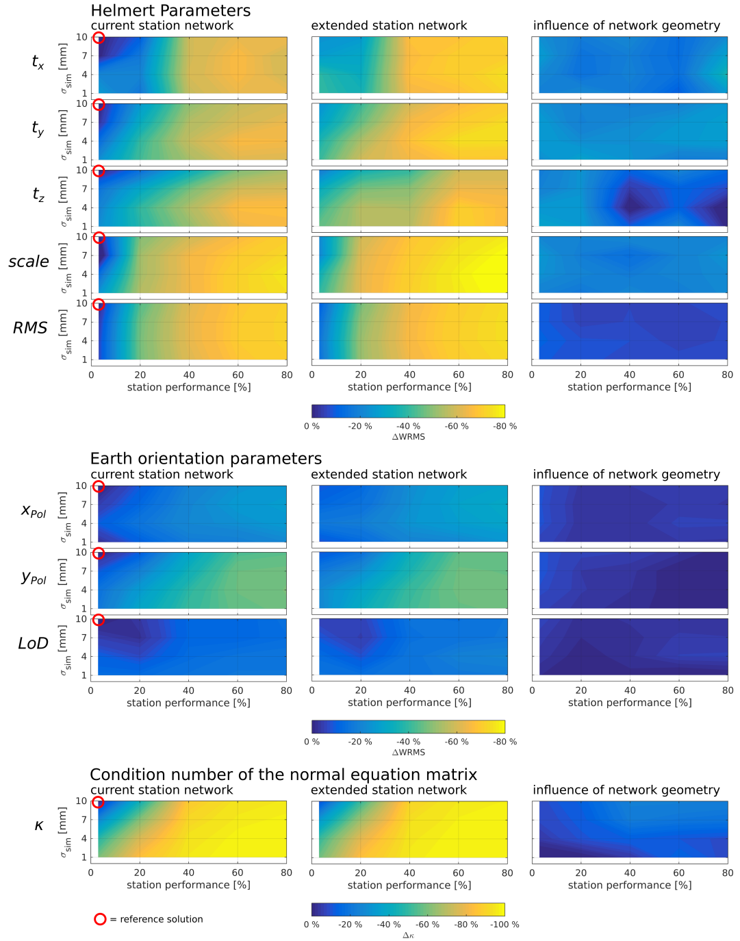
Figure A.1: ■Solutions from Study A . The x-axes represent the minimum station performance, the y-axes represent the simulation noise of a scenario. First column: relative WRMS improvement w.r.t. reference scenario ( \sigma_{sim} = 10 mm, real performances), starting with 0% improvement in the upper left of a plot (red circles). Second column: same as before but with extended station network, i.e., combined effect of technical improvement and network geometry. Third column: effect of network geometry only, i.e., relative improvement between scenarios with current and the extended station networks assuming the same noise and performance conditions.
