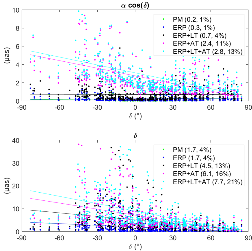
Figure 6.12 Improvement of the AGN coordinate formal errors of the solutions with different ties applied compared to the solution without ties applied (solution “NONE”), as a function of the declination. All the AGN in CONT05–CONT17 are depicted, and the average value of each solution is presented in the legend, together with the relative improvement in percentage. The linear fit results of the improvement as a function of the declination are also presented. Note the different vertical axis scales.
