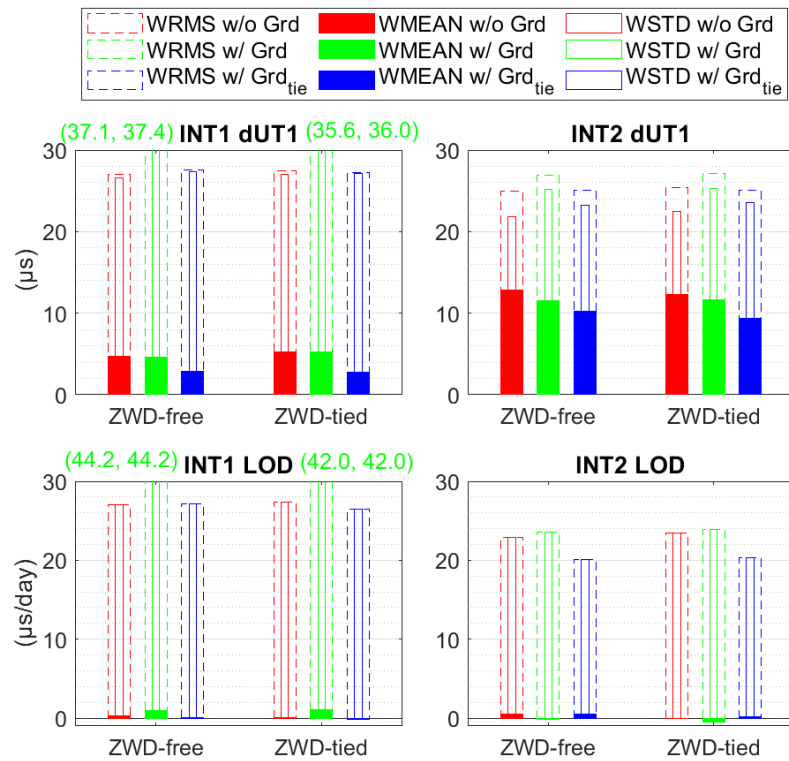
Figure 5.1 Statistics of the UT1-UTC differences compared to the IERS EOP 14 C04 product and LOD differences compared to the IGS product. The WSTD and WRMS values of INT1 exceeding the panels are given in the parentheses.
