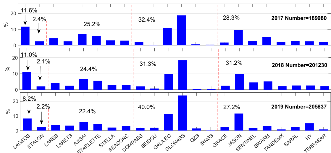
Figure 2.2 SLR session percentage of different satellites in 2017–2019. The LEO satellite list are taken from Table A.1 in Männel (2016). The horizontal axis is the satellite name.
