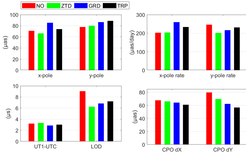
Figure 5.13 WSTD values of the EOP differences between the two VLBI networks in CONT17 (that is, IVS and VLBA) using different tropospheric ties.
