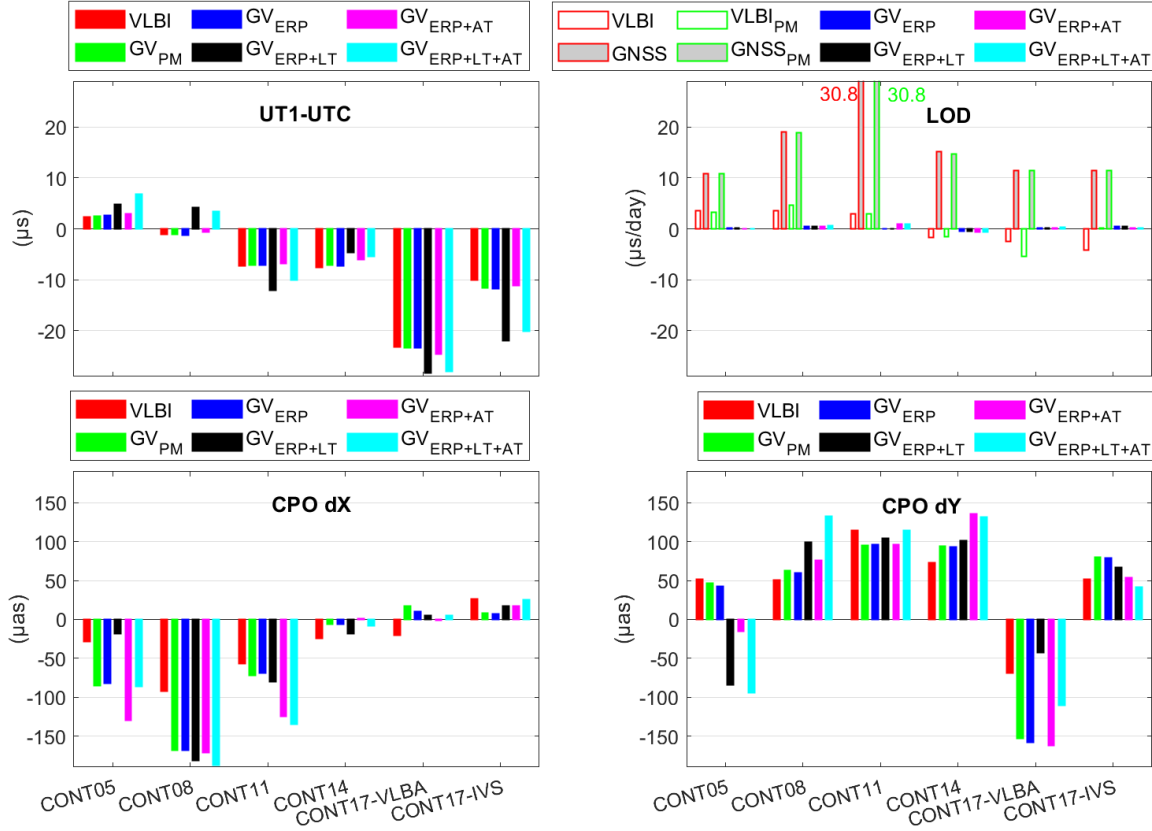
Figure 6.10 WMEAN values of the UT1-UTC, LOD, and CPO estimates compared to IERS EOP 14 C04 in CONT05–CONT17.
