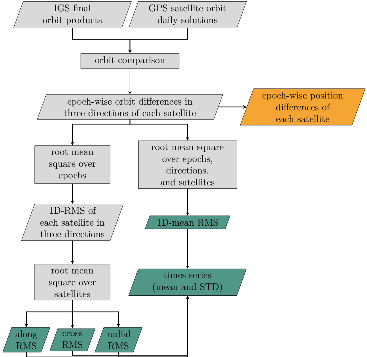
Figure 4.7: Flowchart of the statistical computation. The green and orange outputs are the values used in the analysis of this study.
