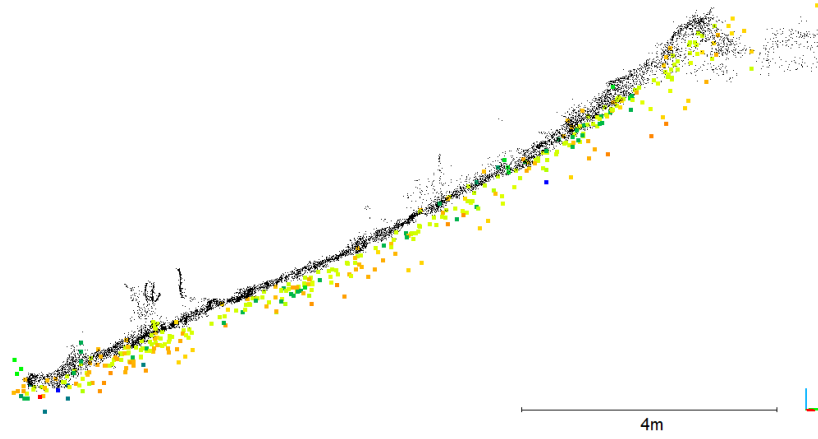
Figure 15: Cross section of mobile lidar point cloud (colorized according to UWB position) and TLS point cloud (black).
