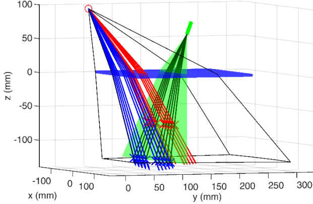
Fig. 10 Calibration result: Refracted image rays intersect with refracted sub-beams (dark green) on top level (red) and bottom level (blue).
