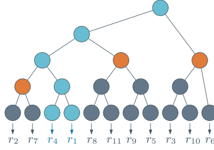
Figure 6.16: The query procedure for a time-window query Q . Blue nodes report true, orange nodes report false, and grey nodes are not queried. The road segments of the two blue leaf nodes correspond to the frequently served road segments for Q .
