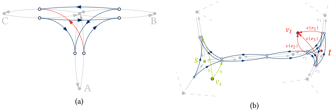
Figure 2.7: Modeling turn weights and turn restrictions with a pseudo-dual graph. (a) The pseudo-dual graph D (blue) of a primal graph (gray) representing a T-junction. If turning left (from A to C) is forbidden, the corresponding edge (red) can be removed from D . (b) To allow finding optimal paths between vertices of the primal graph, dummy source (green) and target (red) vertices are added to the outgoing (resp. incoming) edges of the primal source and target.
