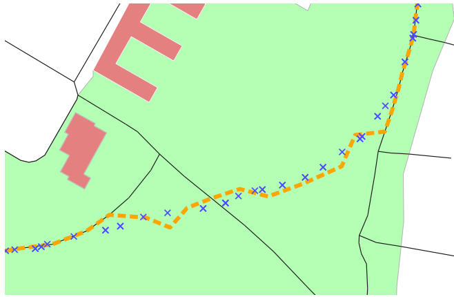
Figure 4.1: Example of a map with an embedded road network as well as free spaces and obstacles. The blue measurement-based trajectory is best explained by movement along the orange dashed path, which follows roads and free spaces where possible but contains no obstacle intersections.
