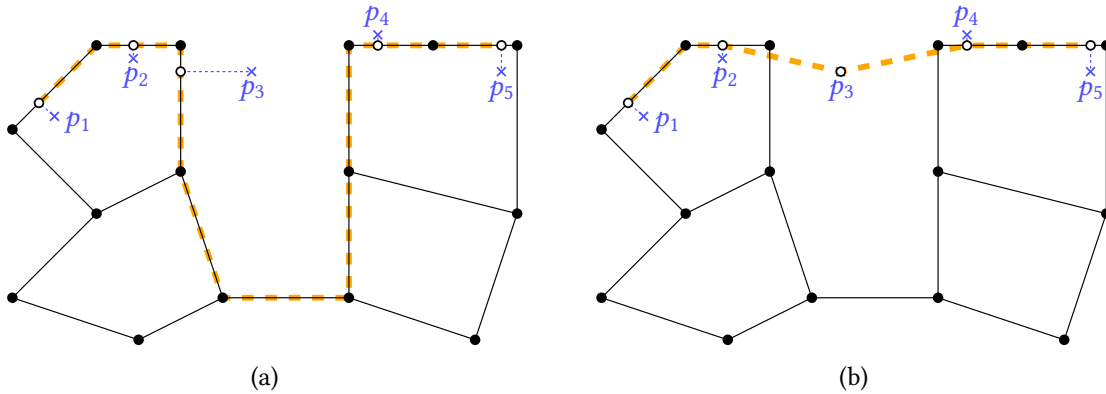
Figure 4.3: (a) Forcing the input trajectory (blue) to the network causes a detour in the output path (dashed). (b) Adding unmatched candidates and connecting segments prevents the detour.
