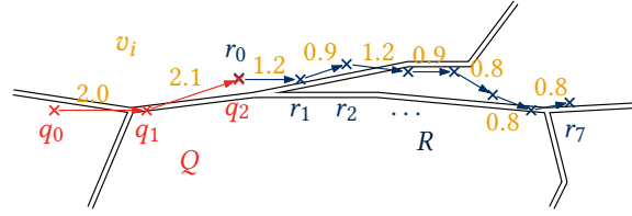
Figure 2.9: The trajectory depicted in Figure 2.8 with velocity per segment (orange). The trajectory is split into two subtrajectories Q (red) and R (blue), using the speed variance as the criterion. Within each subtrajectory, the speed varies by at most one unit. The displayed segmentation is a minimum segmentation for this criterion.
