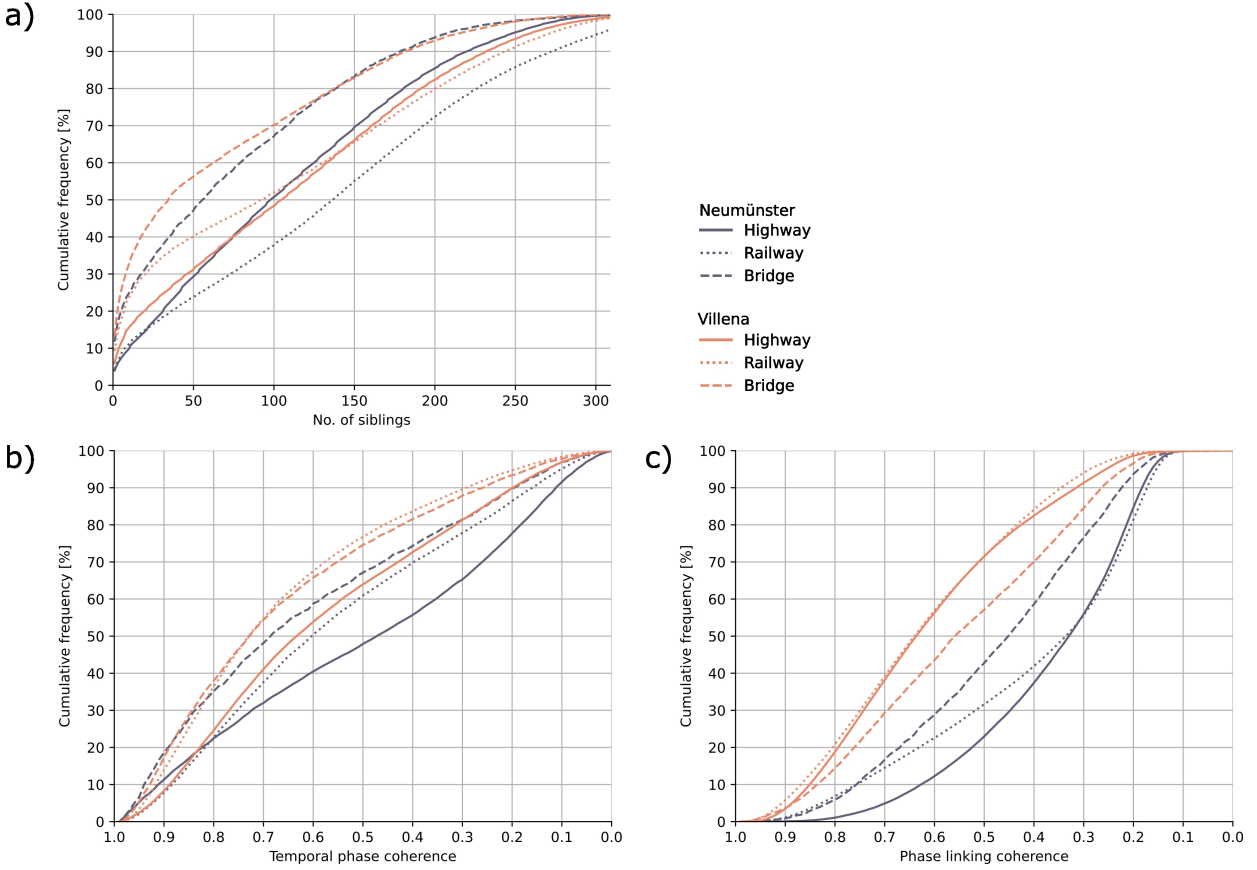
Figure 6.3: Cumulative distributions of a) the number of siblings, b) the TPC, and c) the PLC for highways, railway tracks and bridges in Neumünster and Villena.
