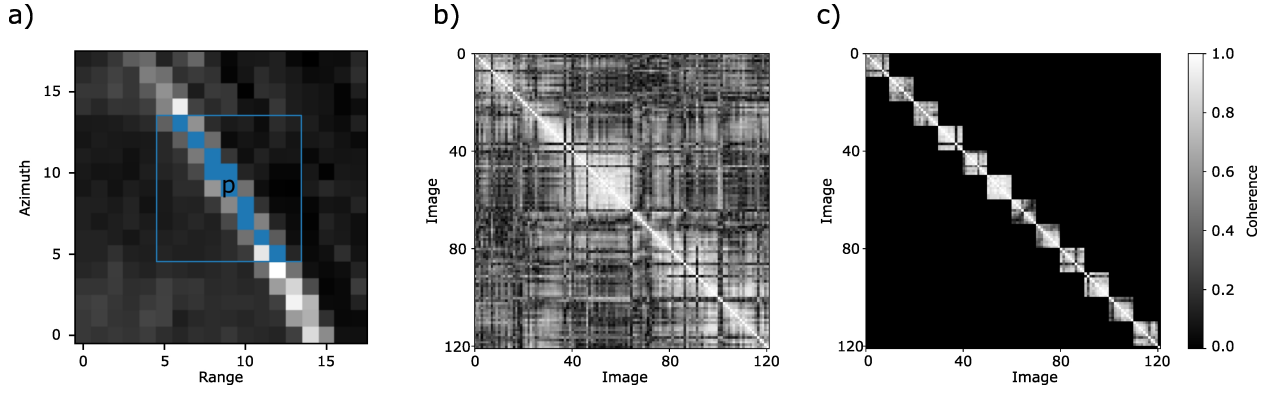
Figure 4.7: Example for the estimation of the coherence matrix from a spatially adaptive neighbourhood for a pixel on a highway in the study area Villena, Spain (Section 5.2). a) Temporally averaged amplitude image with a neighbourhood window of size 9 \times 9 pixels 2 (blue rectangle) around the center pixel p . Blue pixels mark the sibling pixels of p detected with the KS-test. Notably, the sibling pixels coincide with the shape of the highway. b) Estimated coherence matrix \hat{\Gamma} for pixel p . c) The same coherence matrix as in b) but restricted to mini-stacks along the diagonal containing 10 images each to reduce the computational burden of phase linking (Ansari et al., 2017).
