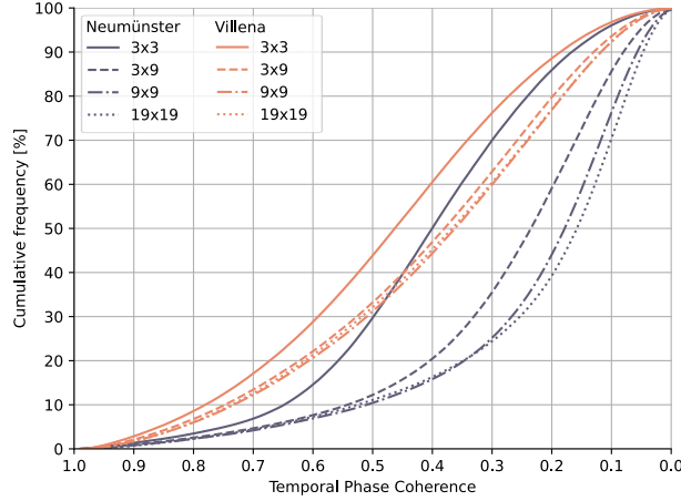
Figure 6.1: Cumulative distribution of TPC for pixels at the transport infrastructure estimated from different window sizes for Villena and Neumünster.
