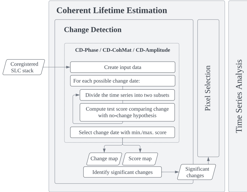
Figure 4.4: Flowchart of the proposed change detection. The three modularly usable change detection methods, CD-Phase, CD-CohMat, and CD-Amplitude, follow the same processing steps, but differ in the type of input data and the computation of the test scores.
