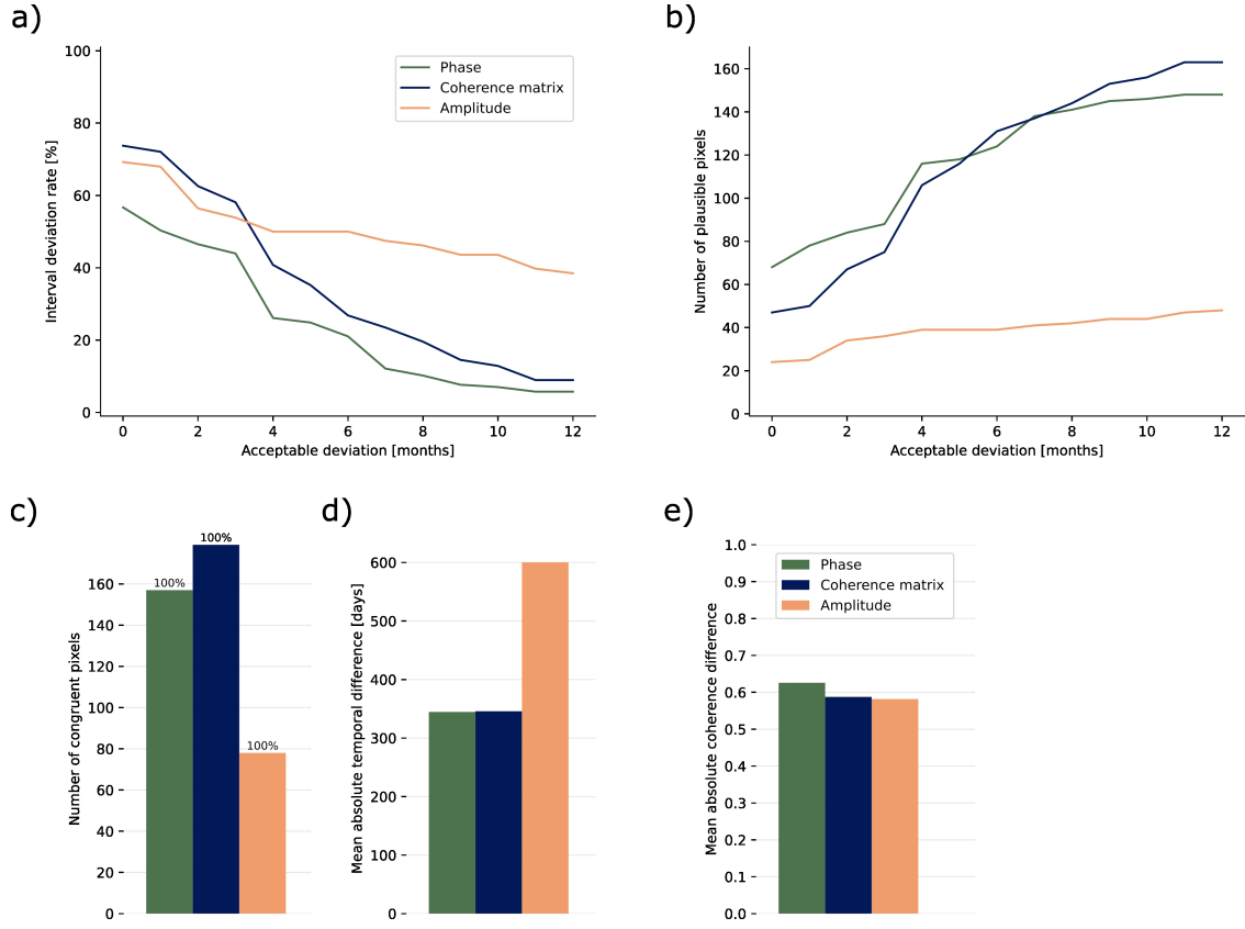
Figure 6.13: Comparison of the plausibility metrics for the three change detection methods at the railway track in the study area Sande. a) Interval deviation rate, b) number of plausible pixels, c) number of congruent pixels as well as the percentage of the congruent pixels among all pixels, d) similarity of the change dates in terms of MATD, and e) mean absolute coherence difference.
