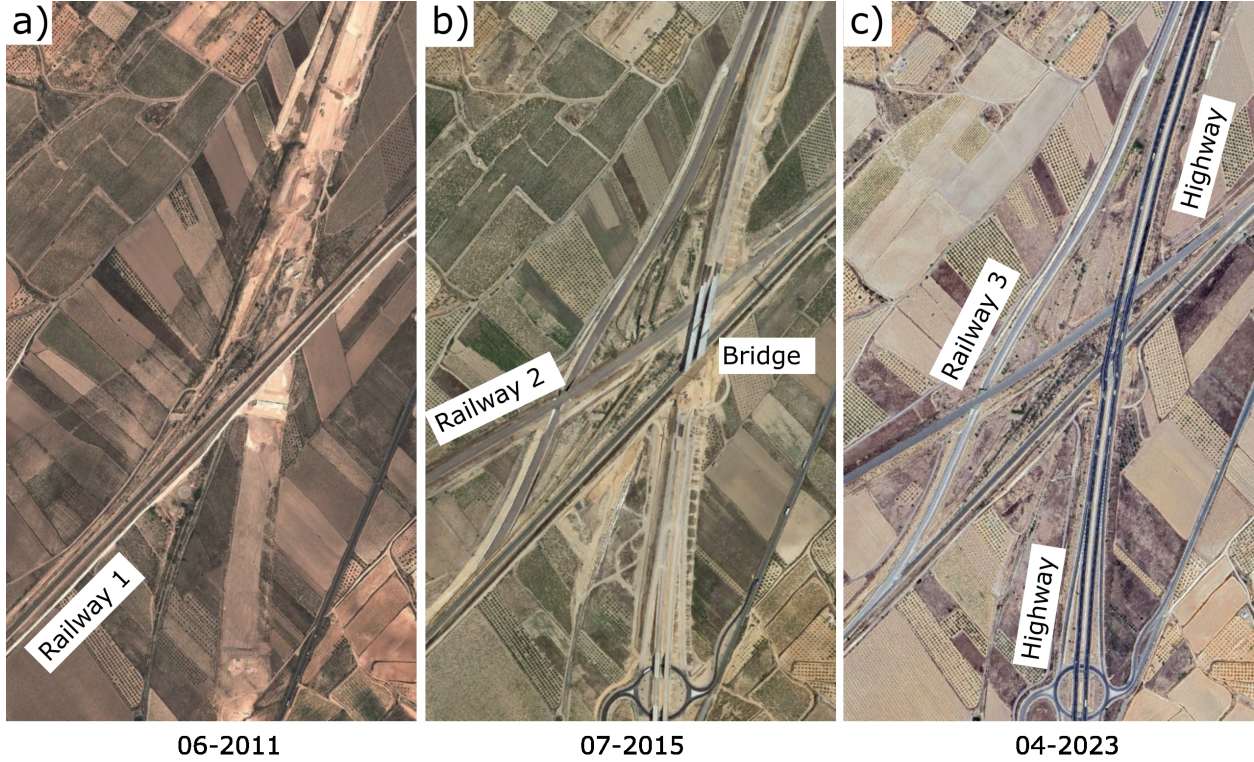
Figure 5.2: Study area Figuera for which a larger dataset is analysed with three railway tracks, a highway and a highway bridge. This study area is a subset of the Villena study area shown in Figure 5.1a. a)-c) Optical satellite images showing the different stages of the construction before and during the study period (Google Earth, Image ©2025 Airbus).
