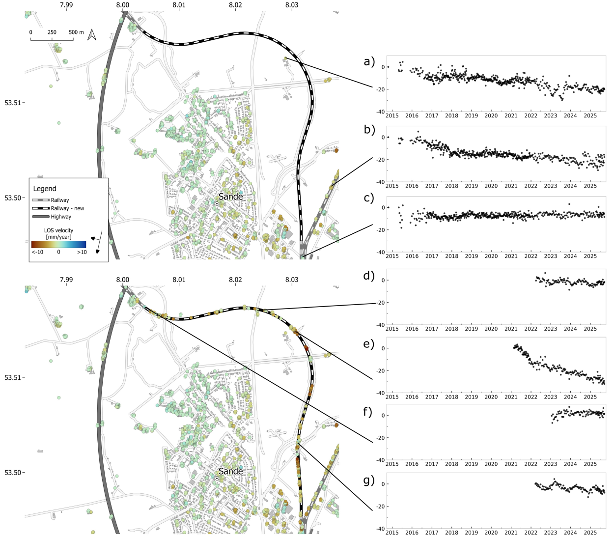
Figure 6.16: Velocity maps of Sande showing LOS displacement derived from CCS pixels only (top), and jointly from CCS and TCS pixels (bottom). Displacement time series (in mm) are shown for selected scatterers on the transport infrastructure (b-g) and on a building close to the new railway track (a). The geolocation of the scatterers were corrected based on the estimated DEM error. Background map is created from OSM data (OpenStreetMap contributors, 2025).
