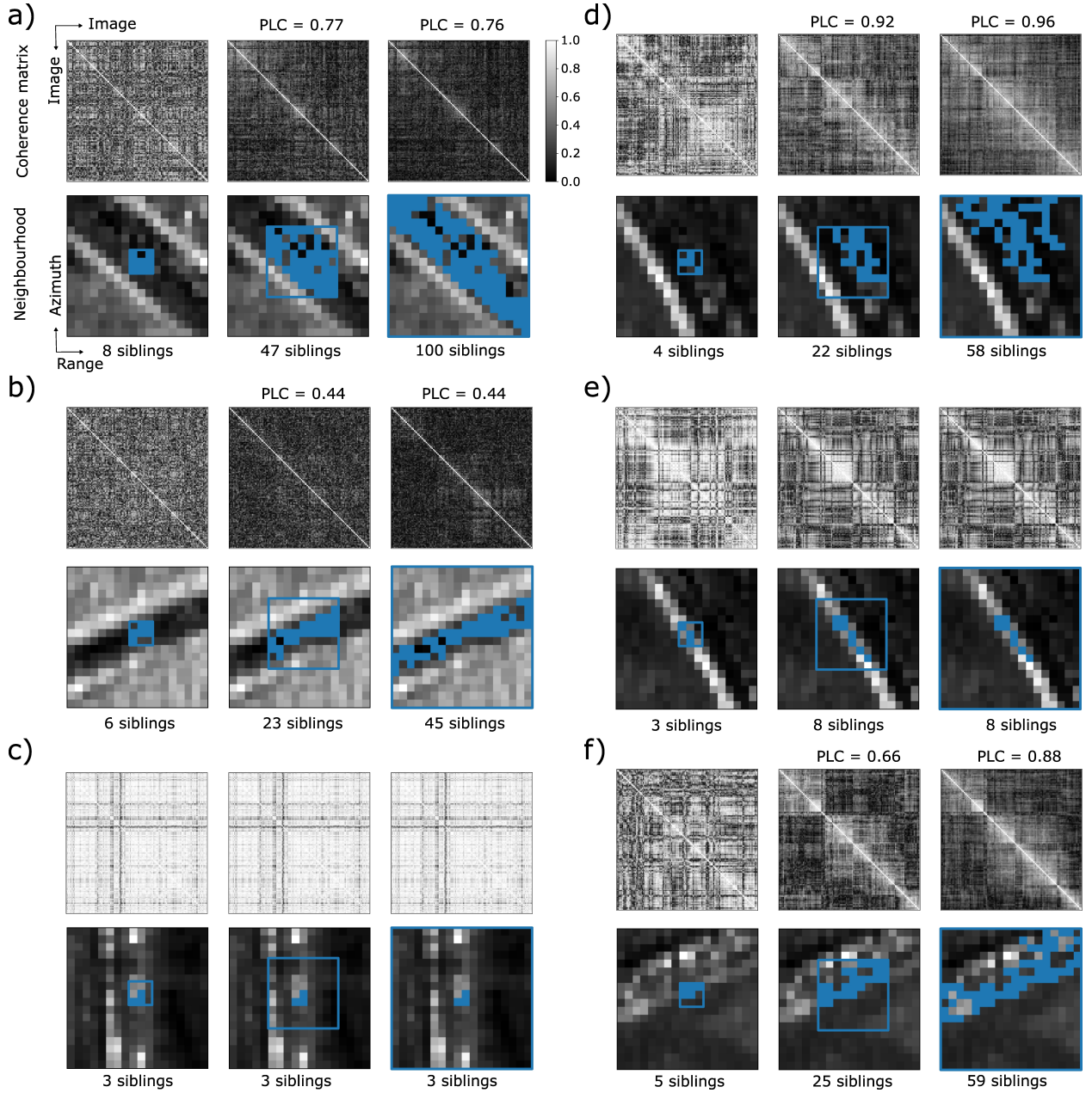
Figure 6.2: Examples for the detection of sibling pixels at transport infrastructure. In each subfigure, the upper row shows the coherence matrix estimated from the set of siblings shown in the bottom row. The sibling pixels are coloured blue and are depicted on top of the temporally averaged amplitude image. The spatial neighbourhood among which the siblings are searched is framed by a blue window. Three different window sizes are exemplarily shown: 3 \times 3 pixels 2 , 9 \times 9 pixels 2 and 19 \times 19 pixels 2 . For each window size, the number of selected siblings and the corresponding PLC are listed. If the number of siblings is below 10, phase linking is not applied and the PLC cannot be estimated. The pixels in a)-c) are taken from Neumünster, while d)-f) are taken from Villena. The pixels in a)-e) correspond to highways and f) corresponds to a railway track.
