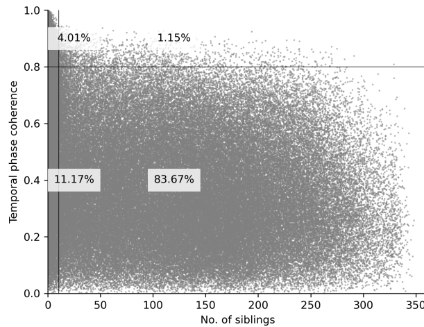
Figure 6.4: Comparison of TPC with the number of siblings found for pixels associated with highways in Villena. The black lines mark the applied thresholds on the number of siblings (10) to identify DS candidate pixels and on the coherence (0.8) for pixel selection. Note that the location of each point on the x-axis is shifted by a random value sampled from a uniform distribution in the interval [-0.25, 0.25] to better visualise points with the same location.
