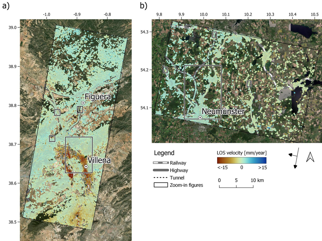
Figure 6.7: Velocity maps of a) Villena and b) Neumünster showing the LOS displacement. Zoom-in figures with regional displacements are shown in Figure 6.8. Zoom-in figures with local displacements are depicted in Figure 6.9 for Villena and in Figure 6.10 for Neumünster. Background image: ©ESRI.
