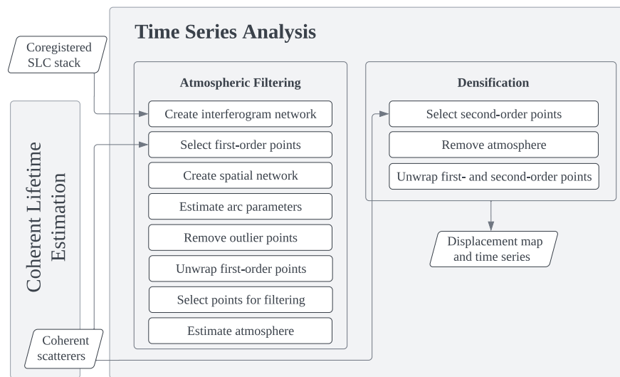
Figure 4.8: Flowchart of the proposed time series analysis.
