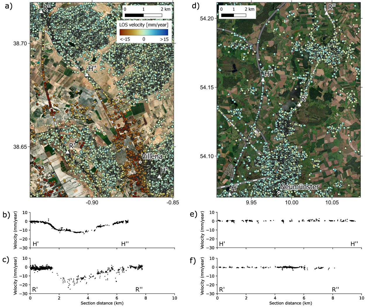
Figure 6.8: Velocity maps showing the LOS displacements for the zoom-ins in a) Villena and d) Neumünster. The mean velocity profiles along a highway (b and e) and a railway (c and f) segment are shown for each study area. The legend is the same as in Figure 6.7. The start and end points of the velocity profiles are marked with a white triangle.
