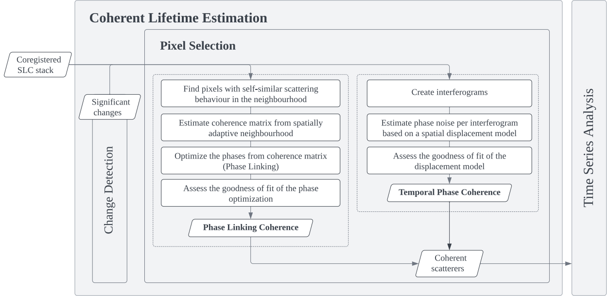
Figure 4.6: Flowchart of the proposed pixel selection.
