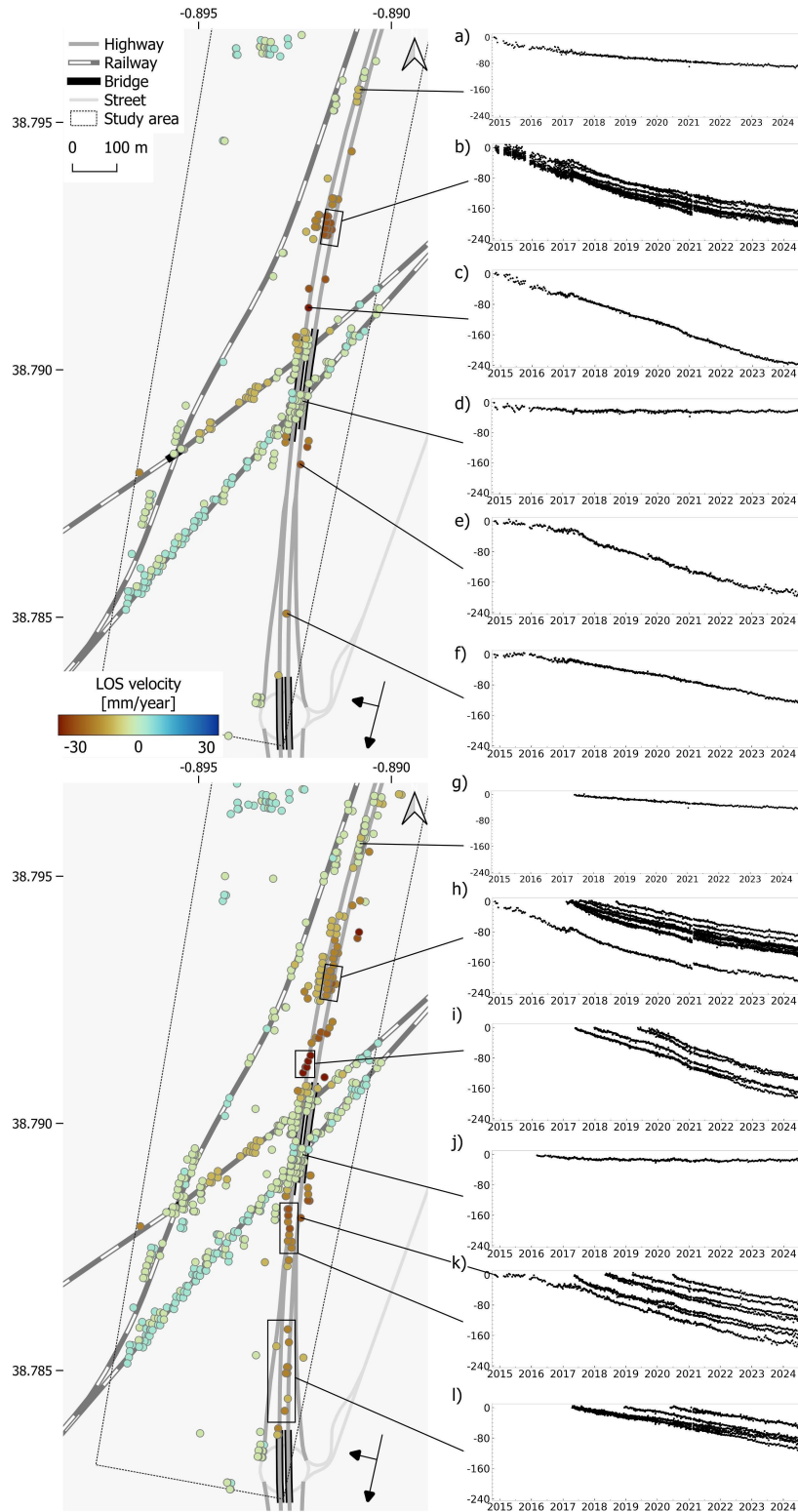
Figure 6.17: Velocity maps of Figuera showing LOS displacement derived from CCS pixels only (top), and jointly from CCS and TCS pixels (bottom). The displacement time series are derived using the InSAR time series for joint phase unwrapping of CCS and TCS pixels. Displacement time series (in mm) are shown for selected scatterers on the transport infrastructure (a-l). The geolocation of the scatterers are corrected based on the estimated DEM error. Background map is created from OSM data (OpenStreetMap contributors, 2025).
