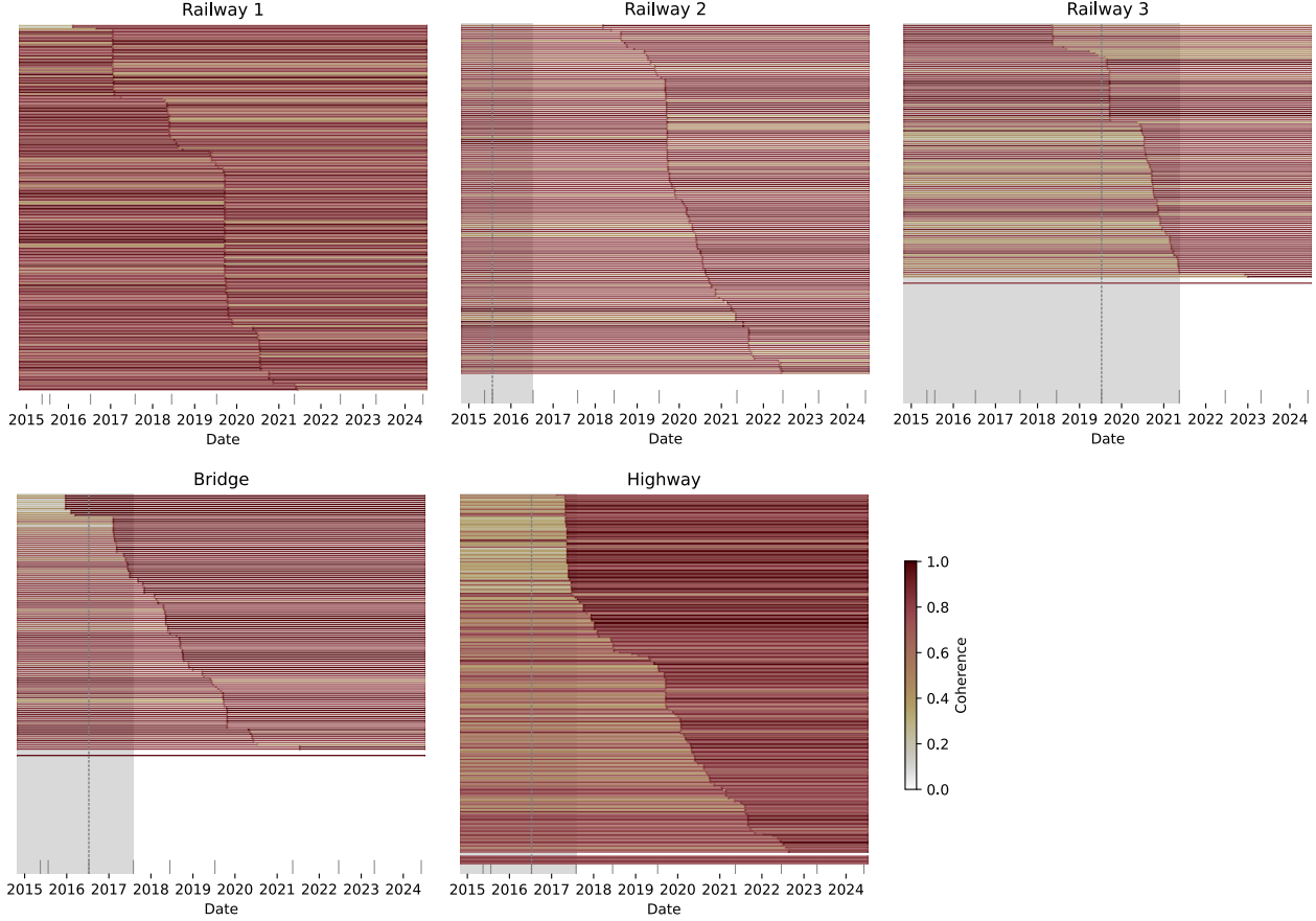
Figure A.1: Coherent lifetime of TCS pixels at five transport infrastructure in Figuera derived from CD-CohMat. Each line represents one scatterer within the mask of a transport infrastructure. Only TCS pixels that were selected during the coherent lifetime estimation are depicted. The lines are coloured by the coherence of the scattering within the time span before and after the estimated change and sorted by the change date in ascending order. The grey areas show the period in which the construction has happened according to optical satellite images (from Google Earth and National Air Orthophotography Plan (PNOA)). The short vertical gray lines along the x-axis indicate the dates of available optical images. The vertical dashed lines highlight the last optical image in which the construction was still visible.
