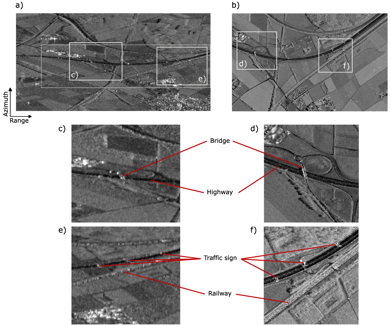
Figure 1.3: Mean amplitude images of transport infrastructure from a) Sentinel-1 and b) TerraSAR-X Stripmap with a spatial resolution of 5\text{ m} \times 20\text{ m} and 3\text{ m} \times 3\text{ m} , respectively. The images show a part of the highway A4 and of the railway tracks between Aachen and Cologne, located south of the Hambach open-pit mine in Germany. The amplitude images are averaged temporally to reduce the effect of speckle, hence, smoothing the image. Moreover, image normalisation is applied to improve the contrast of the images. The white box with a dotted outline in a) corresponds to the extent of the TerraSAR-X amplitude image shown in b). Notably, the areas appear differently due to the non-quadratic shape of the Sentinel-1 pixels. The white boxes in a) are shown in more detail in c) and e), while the white boxes in b), corresponding to approximately the same areas, are depicted in d) and f). The backscattering at the transport infrastructure is similar in TerraSAR-X and Sentinel-1 images. The highway appears dark in images of both sensors, indicating a low backscattering. However, due to the differences in the spatial resolution, the highway lanes can only be differentiated in the TerraSAR-X image. The backscattering is higher at railway tracks compared to highways, as a consequence these appear brighter in the mean amplitude images.
