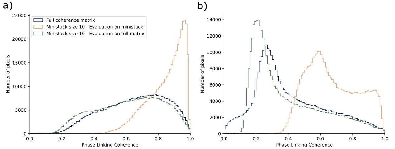
Figure 6.5: Histograms of the PLC evaluated on three phase linking variants considering the full or part of the coherence matrix for all DS candidate pixels on transport infrastructure in a) Villena and b) Neumünster. Pixels on railway tracks, highways or bridges are not differentiated.
