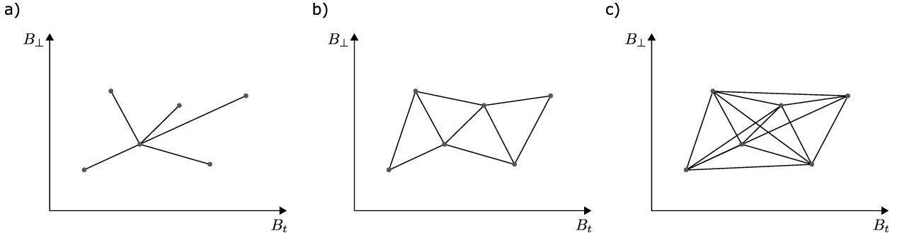
Figure 2.6: Examples of interferogram network types: a) single-reference network, b) small baseline network, c) full network. Each dot denotes an image, while an arc between two images represents an interferogram.
