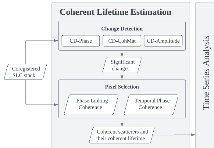
Figure 4.3: Flowchart of the proposed coherent lifetime estimation.
