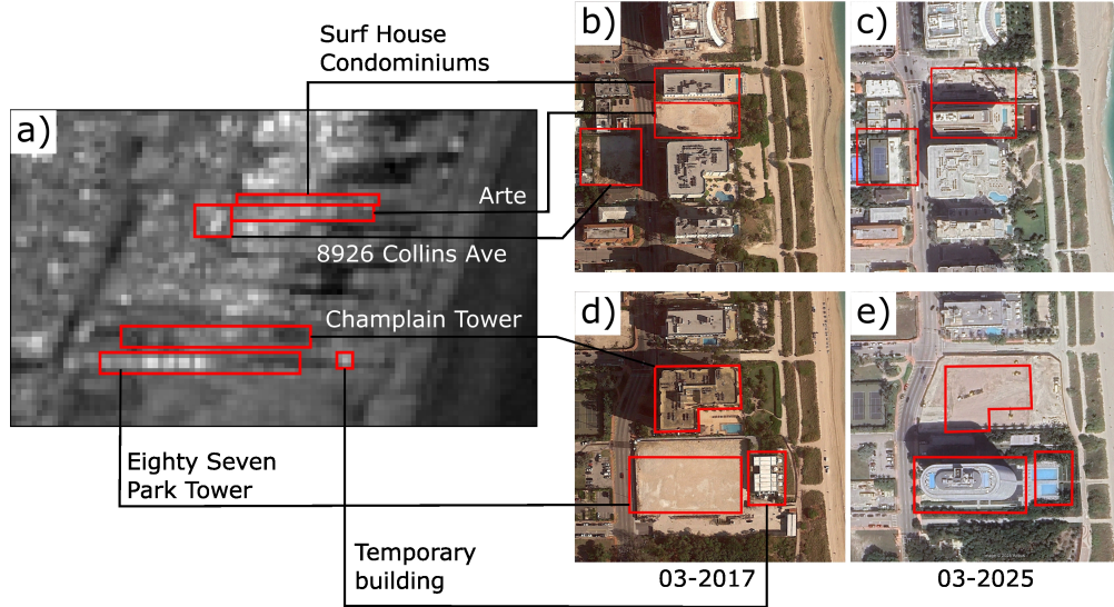
Figure 5.4: Study area in Miami with the location of the six analysed buildings shown with red masks. a) Mean SAR amplitude image. Optical satellite images b) and d) from the beginning (2017), and c) and e) from the end (2025) of the study period (Google Earth, Image ©2025 Airbus). The building masks in the SAR image appear elongated compared to those in optical images because the resolution is higher in the range direction than in the azimuth direction. Moreover, several scatterers are located along different heights of the building, but appear in different pixels in the range direction due to the SAR imaging geometry (see Figure 2.1).
