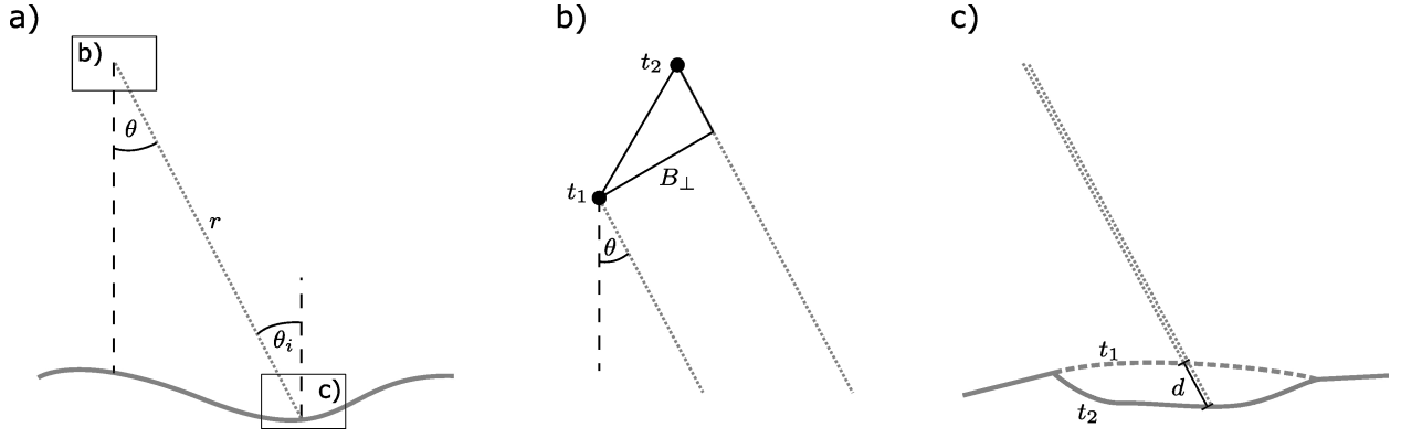
Figure 2.2: Imaging geometry for repeat-pass interferometry with image acquisitions at time t_1 and t_2 , the distance between the sensor and the target r , the look angle of the sensor \theta , the local incidence angle of the target \theta_i , the perpendicular baseline between the two satellite positions B_\perp , and the displacement d at the target due to surface changes. The rectangles in a) are shown in more detail in b) and c).
