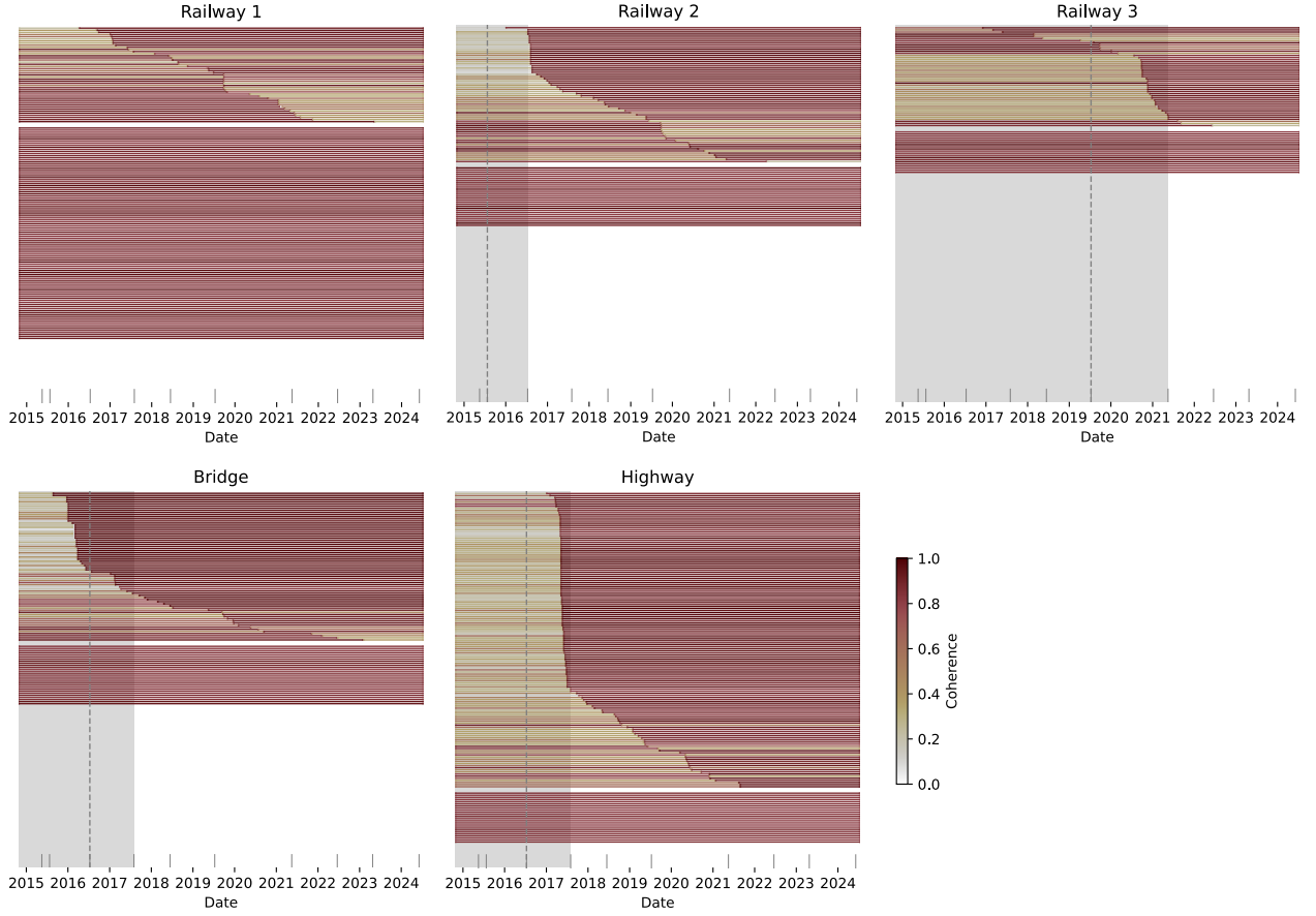
Figure 6.14: Coherent lifetime of TCS pixels at five transport infrastructure in Figuera derived from CD-Phase. Each line represents one scatterer within the mask of a transport infrastructure. Only TCS pixels that were selected during the coherent lifetime estimation are depicted. The lines are coloured by the coherence of the scattering within the time span before and after the estimated change and sorted by the change date in ascending order. The grey areas show the period in which the construction has happened according to optical satellite images (from Google Earth and National Air Orthophotography Plan (PNOA)). The short vertical gray lines along the x-axis indicate the dates of available optical images. The vertical dashed lines highlight the last optical image in which the construction was still visible.
