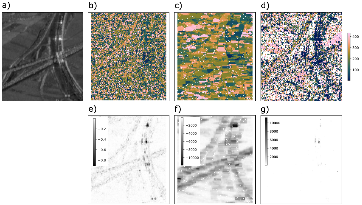
Figure 6.11: Change detection results for the study area Figuera with a) mean amplitude image, b)-d) change maps indicating the image acquisition for each pixel after which the change has occurred, and e)-g) change scores for each pixel belonging to the change dates in the change maps. The corresponding change maps and score maps from the change detection methods are presented column-wise with CD-Phase (b, e), CD-CohMat (c, f), and CD-Amplitude (d, g). The change cannot be estimated for pixels at the border of the maps from CD-Phase and CD-CohMat due to the estimation window and are depicted in white. Changes which are classified as insignificant based on the F-test in CD-Amplitude are also depicted in white.
