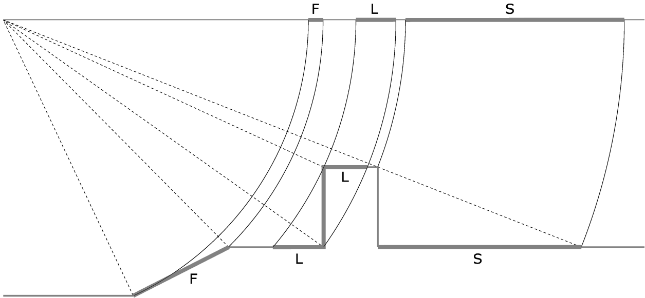
Figure 2.1: Simplified scheme of the SAR imaging geometry with the side-looking sensor located in the top left corner. The slope oriented towards the sensor appears foreshortened (F) in the SAR image. The building yields layover (L) at the roof, the wall and the ground in front of the building. The area behind the building is not illuminated which results in shadow (S).
