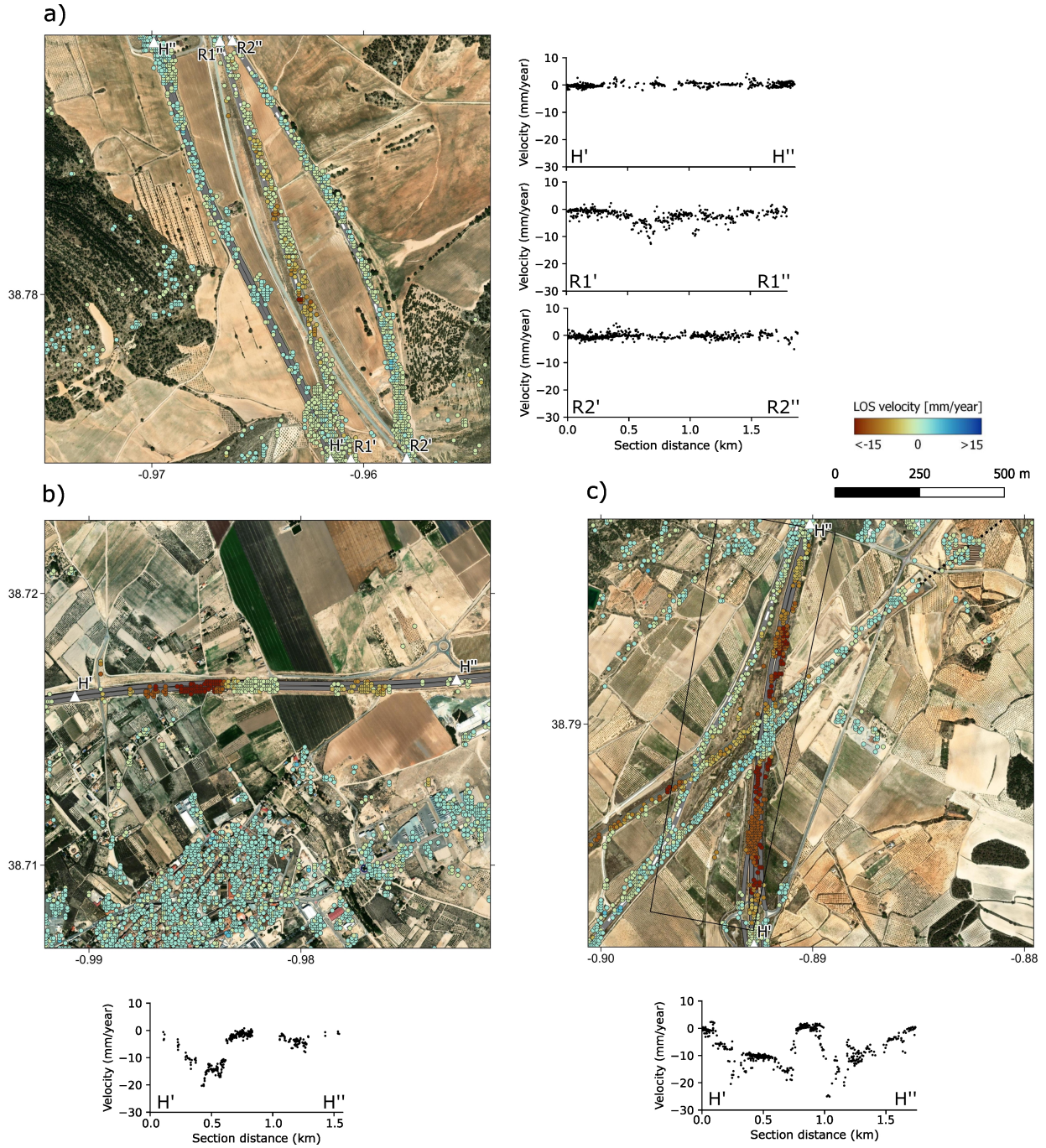
Figure 6.9: Velocity maps showing the LOS displacement for the zoom-ins in Villena (Figure 6.7a) for two railway and three highway segments. The legend is the same as in Figure 6.7. For each segment, the mean velocity profile is shown along the transport infrastructure. Start and end points of the profiles are depicted by the white triangles. The extent of the study area Figuera used in other experiments is depicted in c) by the black rectangle. Background image: ©ESRI.
