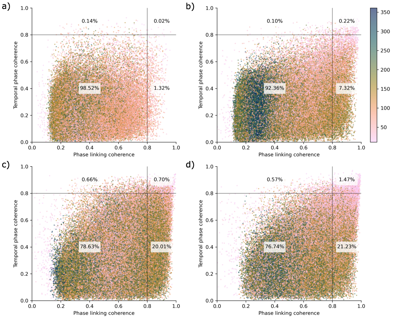
Figure 6.6: Pixel-wise comparison of TPC and PLC for DS candidate pixels for highways (a, c) and railway tracks (b, d) from Neumünster (a, b) and Villena (c, d). The black lines mark the applied thresholds on the coherence (0.8) for pixel selection. The colour represents the number of siblings found for each pixel.
