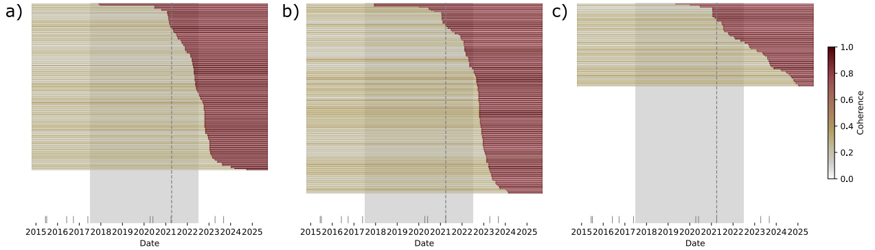
Figure 6.12: Coherent lifetime of TCS pixels at the railway track in Sande derived from a) CD-Phase, b) CD-CohMat, and c) CD-Amplitude. Each line represents one scatterer at the railway track. Only TCS pixels that were selected during the coherent lifetime estimation are depicted. The lines are coloured by the coherence of the scattering within the time span before and after the estimated change and are sorted by the change date in ascending order. The grey areas show the period in which the construction has happened according to optical satellite images (from Google Earth and LGLN, compare Figure 5.3). The short vertical gray lines along the x-axis indicate the dates of available optical images. The vertical dashed lines highlight the last optical image in which the construction was still visible.
