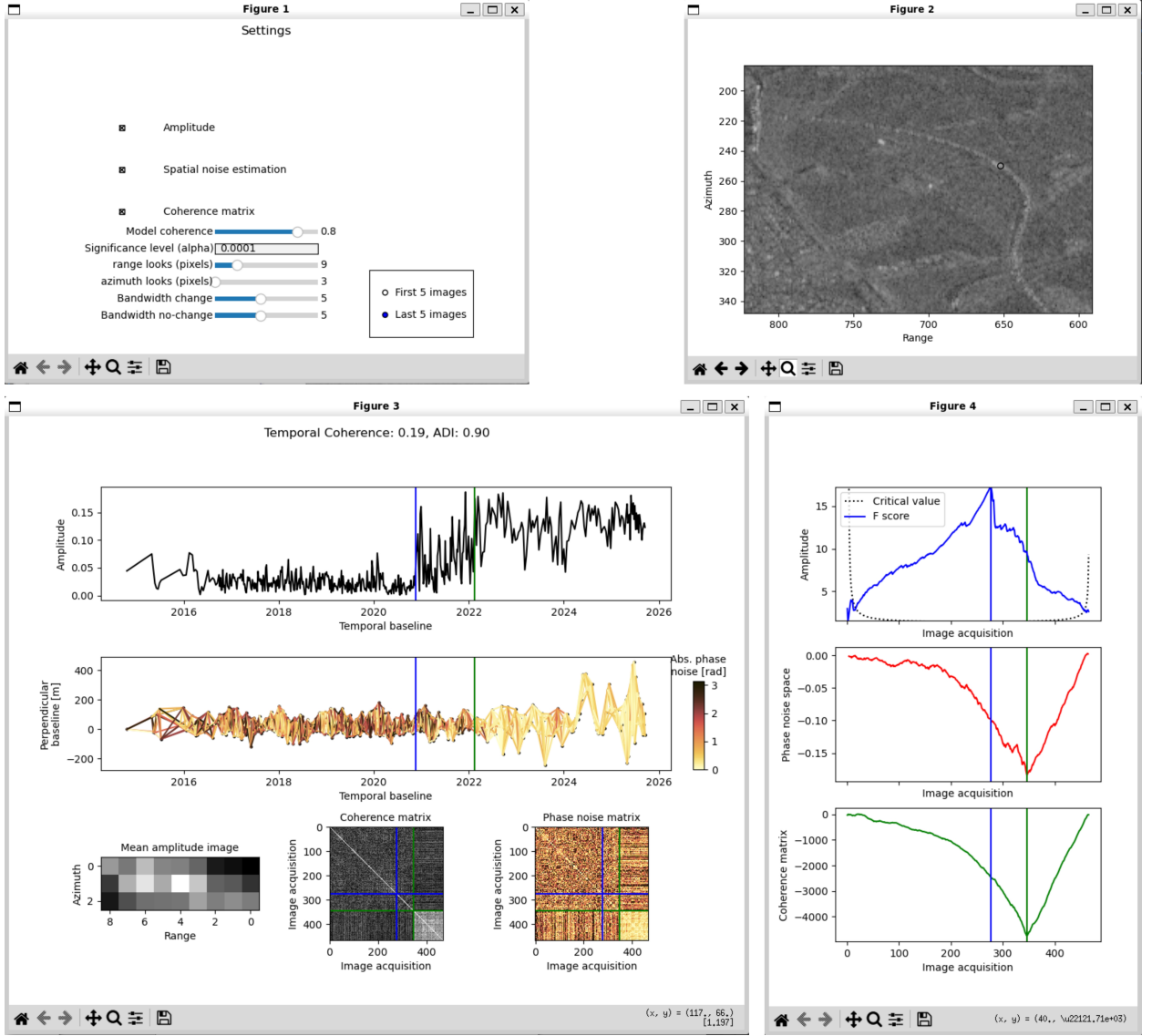
Figure A.3: Interactive change detection tool implemented in the software SpaTZ, developed within the scope of this thesis, for analysing the temporal behaviour of individual scatterers and for comparing the change detection methods. The example shows a TCS pixel in the study area Sande (see Section 5.2) at the new railway track marked with a black circle in the top right window ( Figure 2 ). Figure 1 : Settings for controlling the three change detection methods CD-Amplitude, CD-Phase and CD-CohMat. Figure 2 : Amplitude image averaged over the last five images of the SAR stack. Figure 3 : Input to each of the change detection methods including the amplitude time series, the absolute phase noise in a small baseline interferogram network, the mean amplitude image within the spatial neighbourhood considered during estimation (here 3 \times 9 pixels 2 ), the coherence matrix and the phase noise matrix. Figure 4 : Score time series for each change detection method and the detected changes. The vertical lines in Figure 3 and Figure 4 highlight the location of the detected changes. These changes are also marked by horizontal lines in the coherence matrix and the phase noise matrix due to the symmetry of the matrices. The vertical and horizontal lines correspond to the change detection methods as shown by the colours: blue for CD-Amplitude, red for CD-Phase, and green for CD-CohMat. The lines are depicted in each of the graphs to enable the direct comparison of the detected changes. Notably, CD-Phase and CD-CohMat detected the same change date and, thus, the red line is not visible because it is overlaid by the green line.
