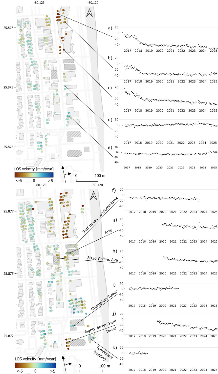
Figure 6.19: Velocity maps of the study area in Miami showing the LOS displacement derived from CCS pixels only (top), and jointly from CCS and TCS pixels (bottom). The changes are detected with CD-Phase. Displacement time series (in mm) are shown for selected scatterers on the high-rise buildings. The geolocation of the scatterers were corrected based on the estimated DEM error. Buildings with cross-hatched area are analysed in more detail in Figure 6.18. Background map is created from OSM data (OpenStreetMap contributors, 2025).
