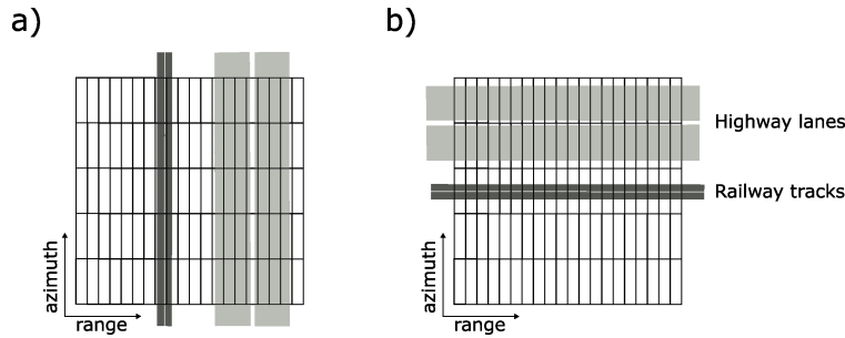
Figure 1.2: Pixel coverage at a highway and a railway track for the spatial resolution of Sentinel-1 with 5\text{ m} \times 20\text{ m} pixel size in range and azimuth, respectively, depending on the direction of the transport infrastructure: a) Transport infrastructure is parallel to, and b) perpendicular to the flight direction of the satellite (azimuth direction).
