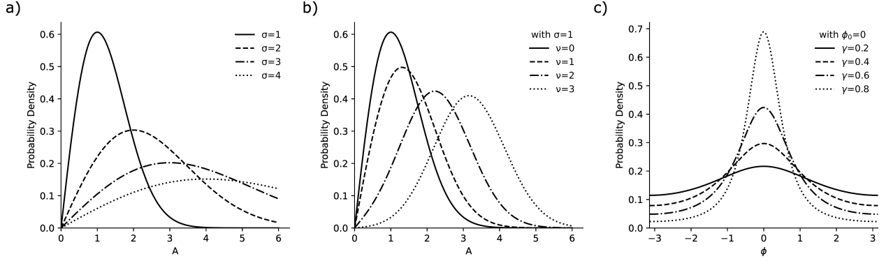
Figure 2.3: The amplitude of the SAR signal follows either a) the Rayleigh or b) the Rice distribution. Notably, the two distributions are the same for \nu = 0 . The PDF of the interferometric phase for single-look resolution interferograms is shown in c) for different coherence values.
