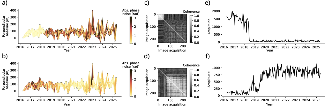
Figure 4.5: Examples of input for the three change detection methods: a) and b) phase noise in each interferogram of a small baseline interferogram network (Section 4.3.1.1), c) and d) coherence matrix (Section 4.3.1.2), e) and f) amplitude time series (Section 4.3.1.3). The examples are taken from the study area in the Miami, USA analysed in Experiment 5 in Section 6.5. Top row panels (a, c and e) correspond to one scatterer on the temporary building, while the bottom row panels (b, d and f) correspond to one scatterer on the Eighty Seven Park Tower (see Figure 5.4 for SAR and optical view of the buildings and Figure 6.19 for the corresponding displacement time series). For the scatterer on the temporary building, the change is apparent and clear in the phase noises in the interferogram network, in the coherence matrix and in the amplitude time series. In contrast, while the change is noticeable at the scatterer on the Eighty Seven Park Tower, it cannot be clearly attributed to a specific date.
